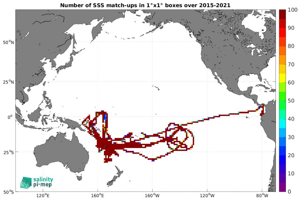
Figure 5: Number of SSS match-ups between TSG (GOSUD-Research-vessel) SSS and the SMAP SSS L3 v5.0 - 8-Day running (JPL) SSS product for the Pacific Ocean Pi-MEP region over 1°x1° boxes and for the full satellite product period.
