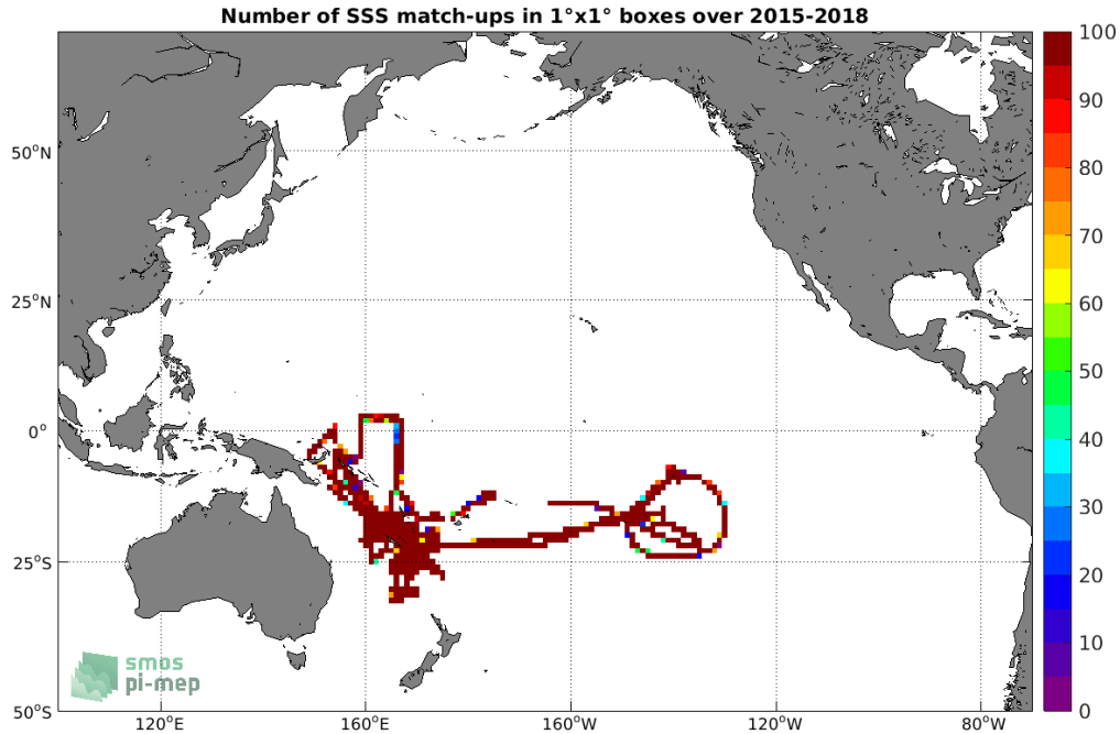
Figure 4: Number of SSS match-ups between TSG (GOSUD-Research-vessel) SSS and the SMAP SSS L3 v5.0 - 8-Day running (JPL) SSS product for the Pacific Ocean Pi-MEP region over 1^\circ \times 1^\circ boxes and for the full satellite product period.
