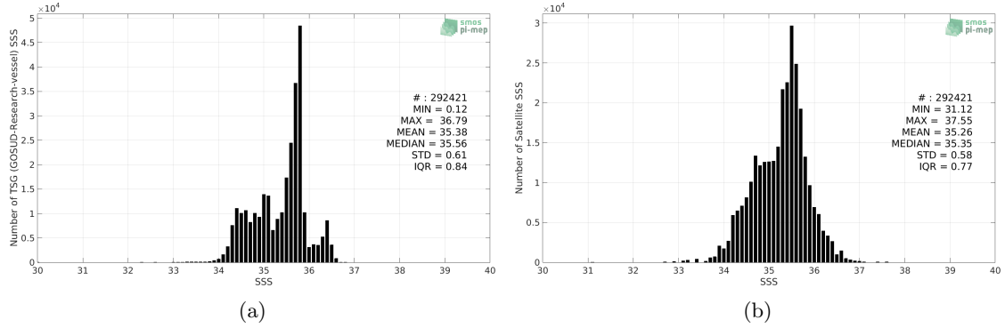
Figure 2: Histograms of SSS from TSG (GOSUD-Research-vessel) (a) and SMAP SSS L3 v5.0 - 8-Day running (JPL) (b) considering all match-up pairs per bins of 0.1 over the Pacific Ocean Pi-MEP region and for the full satellite product period.
