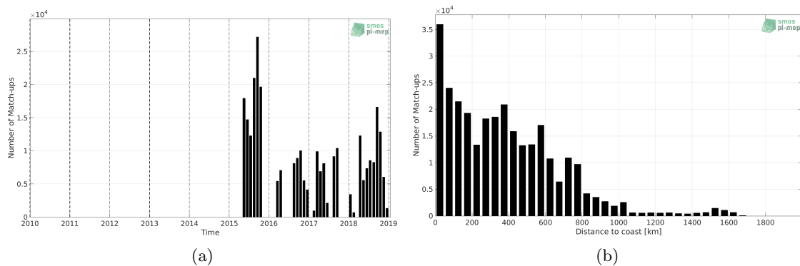
Figure 1: Number of match-ups between TSG (GOSUD-Research-vessel) and SMAP SSS L3 v5.0 - 8-Day running (JPL) SSS as a function of time (a) and as function of the distance to coast (b) over the Pacific Ocean Pi-MEP region and for the full satellite product period.
