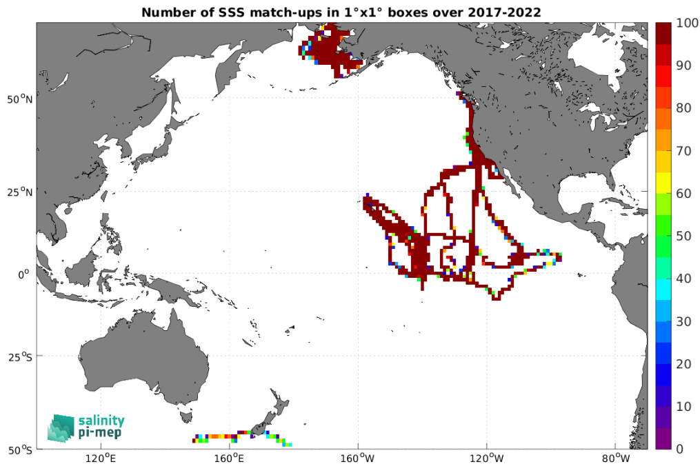
Figure 5: Number of SSS match-ups between Saildrone SSS and the SMAP SSS L3 v5.0 - 8-Day running (JPL) SSS product for the Pacific Ocean Pi-MEP region over 1^\circ \times 1^\circ boxes and for the full satellite product period.
