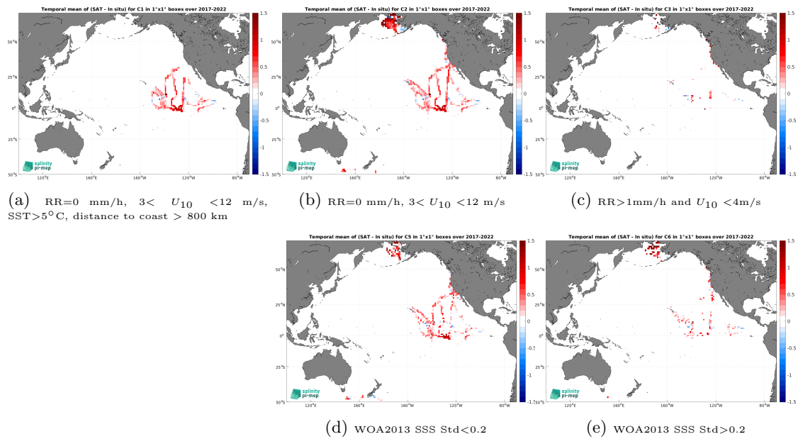
Figure 14: Temporal mean gridded over spatial boxes of size 1^\circ \times 1^\circ of \Delta SSS (SMAP SSS L3 v5.0 - 8-Day running (JPL) - Saifdrone) for 5 different subdatasets corresponding to:RR=0 mm/h, 3 < U_{10} < 12 m/s, SST > 5^\circ\text{C} , distance to coast > 800 km (a), RR=0 mm/h, 3 < U_{10} < 12 m/s (b), RR > 1 mm/h and U_{10} < 4 m/s (c), WOA2013 SSS Std < 0.2 (d), WOA2013 SSS Std > 0.2 (e).
