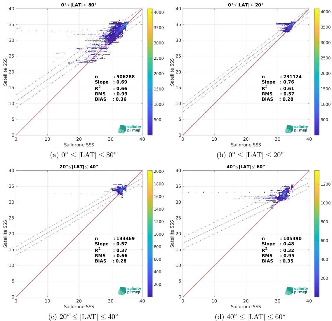
Figure 10: Contour maps of the concentration of SMAP SSS L3 v5.0 - 8-Day running (JPL) SSS (y-axis) versus Saildrone SSS (x-axis) at match-up pairs for different latitude bands. For each plot, the red line shows x=y . The black thin and dashed lines indicate a linear fit through the data cloud and the \pm 95\% confidence levels, respectively. The number match-up pairs n , the slope and R^2 coefficient of the linear fit, the root mean square (RMS) and the mean bias between satellite and in situ data are indicated for each latitude band in each plots.
