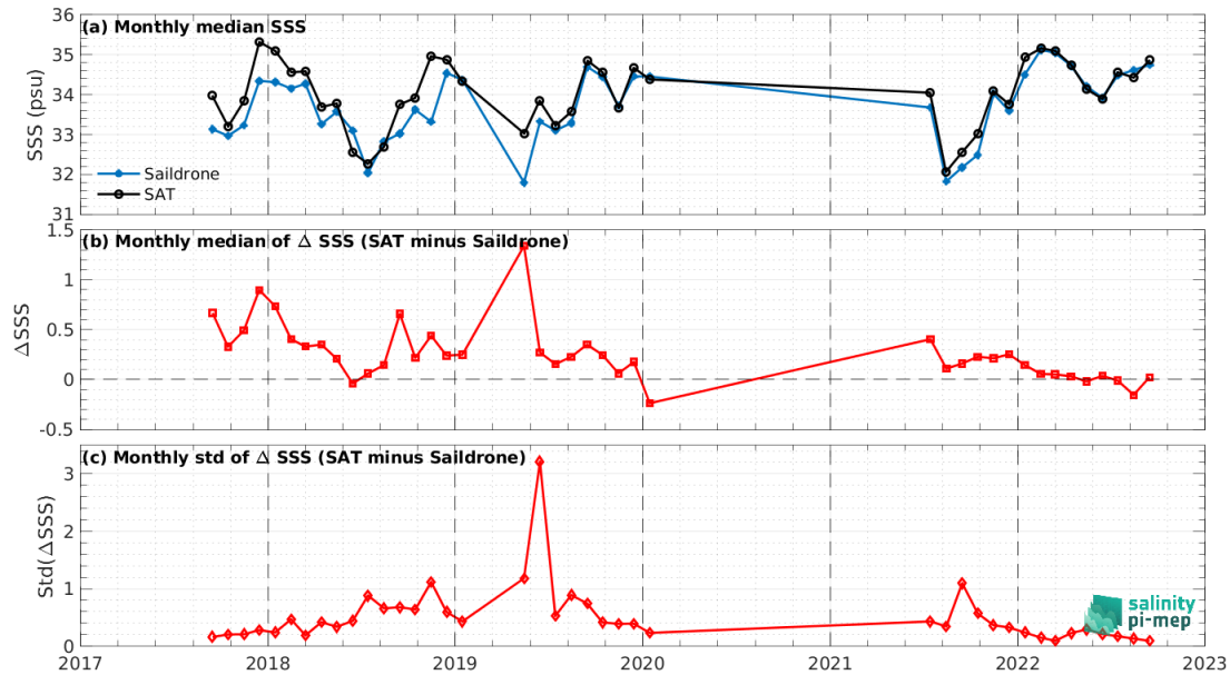
Figure 8: Time series of the monthly median SSS (top), median of \Delta SSS (Satellite - Saildrone) and Std of \Delta SSS (Satellite - Saildrone) over the Pacific Ocean Pi-MEP region considering all match-ups collected by the Pi-MEP.
