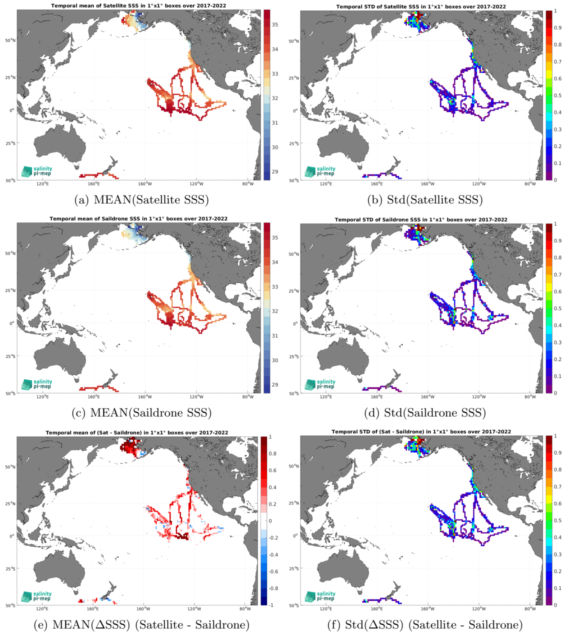
Figure 7: Temporal mean (left) and Std (right) of SSS from SMAP SSS L3 v5.0 - 8-Day running (JPL) (top), Saildrone (middle), and of \Delta SSS (Satellite - Saildrone). Only match-up pairs are used to generate these maps.
