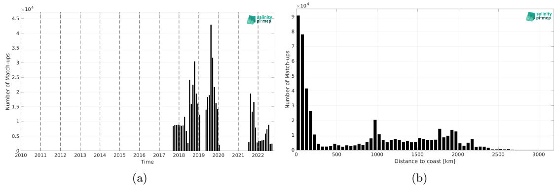
Figure 2: Number of match-ups between Sairdrone and SMAP SSS L3 v5.0 - 8-Day running (JPL) SSS as a function of time (a) and as function of the distance to coast (b) over the Pacific Ocean Pi-MEP region and for the full satellite product period.
