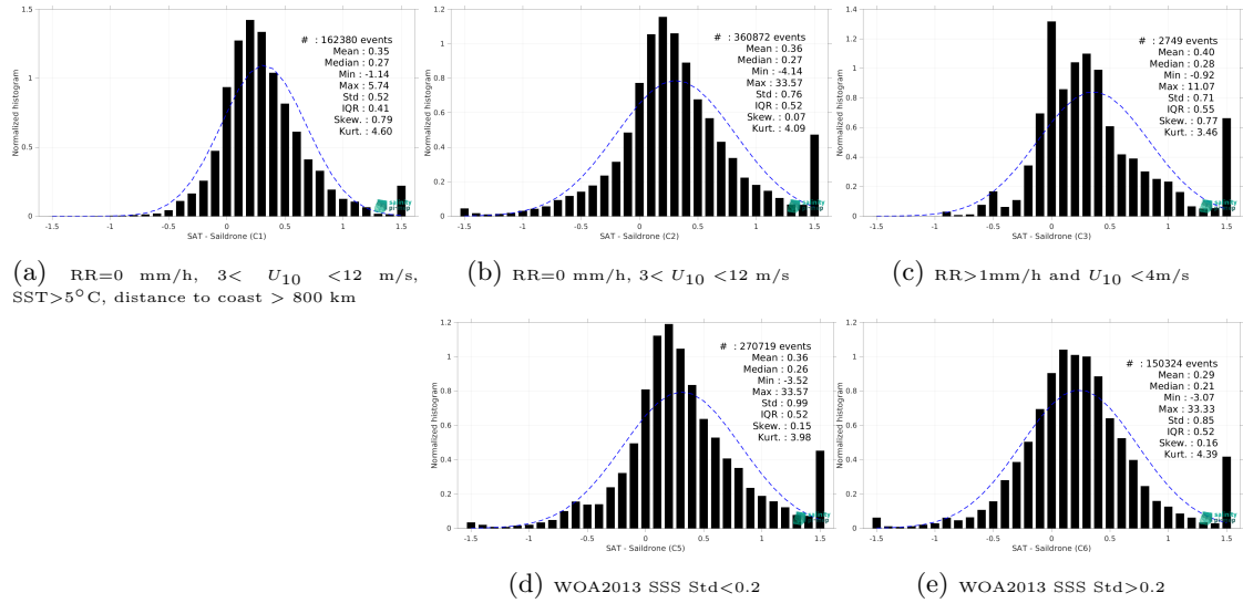
Figure 15: Normalized histogram of \Delta SSS (SMAP SSS L3 v5.0 - 8-Day running (JPL) - Salsdrone) for 5 different subdatasets corresponding to: RR=0 mm/h, 3 < U_{10} < 12 m/s, SST>5°C, distance to coast > 800 km (a), RR=0 mm/h, 3 < U_{10} < 12 m/s (b), RR>1mm/h and U_{10} < 4 m/s (c), WOA2013 SSS Std<0.2 (d), WOA2013 SSS Std>0.2 (e).
