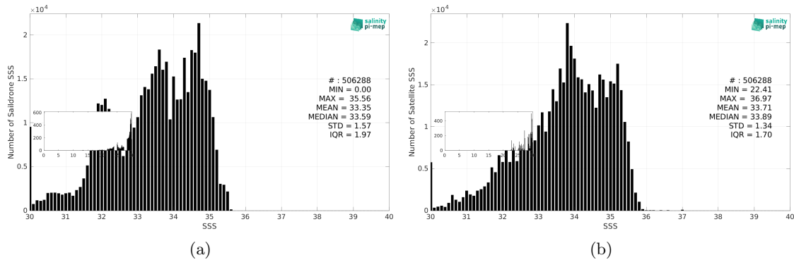
Figure 3: Histograms of SSS from Sairdrone (a) and SMAP SSS L3 v5.0 - 8-Day running (JPL) (b) considering all match-up pairs per bins of 0.1 over the Pacific Ocean Pi-MEP region and for the full satellite product period.
