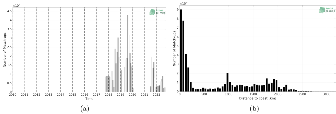
Figure 1: Number of match-ups between Sairdrone and SMAP SSS L3 v5.0 - 8-Day running (JPL) SSS as a function of time (a) and as function of the distance to coast (b) over the Pacific Ocean Pi-MEP region and for the full satellite product period.
