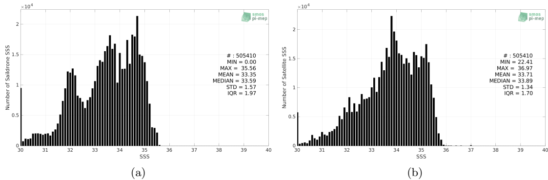
Figure 2: Histograms of SSS from Sairdrone (a) and SMAP SSS L3 v5.0 - 8-Day running (JPL) (b) considering all match-up pairs per bins of 0.1 over the Pacific Ocean Pi-MEP region and for the full satellite product period.
