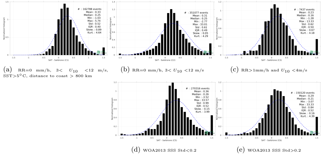
Figure 13: Normalized histogram of \Delta SSS (SMAP SSS L3 v5.0 - 8-Day running (JPL) - Saldrone) for 5 different subdatasets corresponding to: RR=0 mm/h, 3 < U_{10} < 12 m/s, SST>5°C, distance to coast > 800 km (a), RR=0 mm/h, 3 < U_{10} < 12 m/s (b), RR>1mm/h and U_{10} < 4 m/s (c), WOA2013 SSS Std<0.2 (d), WOA2013 SSS Std>0.2 (e).
