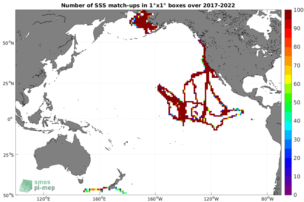
Figure 4: Number of SSS match-ups between Saildrone SSS and the SMAP SSS L3 v5.0 - 8-Day running (JPL) SSS product for the Pacific Ocean Pi-MEP region over 1^\circ \times 1^\circ boxes and for the full satellite product period.
