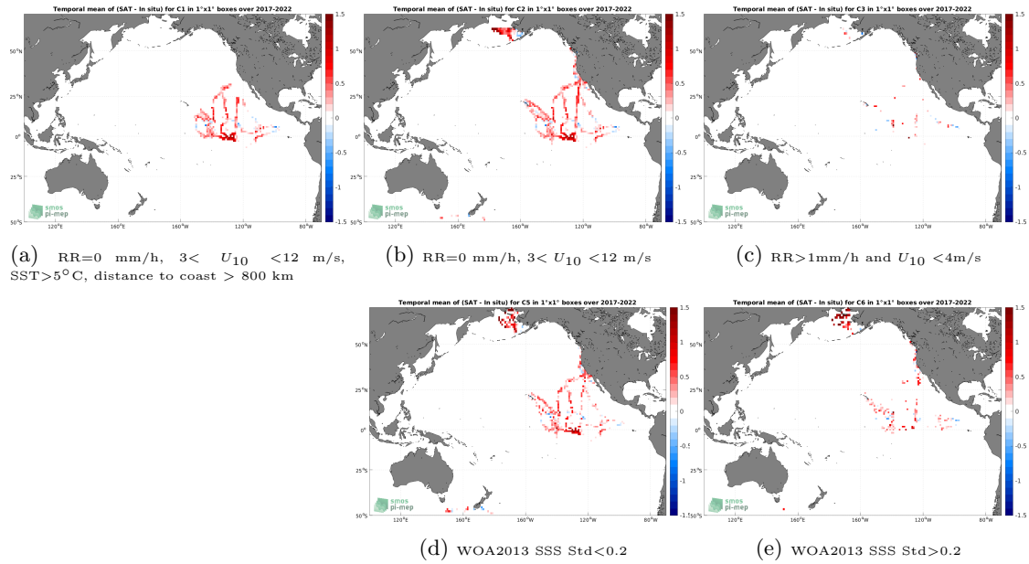
Figure 12: Temporal mean gridded over spatial boxes of size 1^\circ \times 1^\circ of \Delta SSS (SMAP SSS L3 v5.0 - 8-Day running (JPL) - Sairdrone) for 5 different subdatasets corresponding to:RR=0 mm/h, 3 < U_{10} < 12 m/s, SST >5^\circ C, distance to coast > 800 km (a), RR=0 mm/h, 3 < U_{10} < 12 m/s (b), RR >1 mm/h and U_{10} < 4 m/s (c), WOA2013 SSS Std <0.2 (d), WOA2013 SSS Std >0.2 (e).
