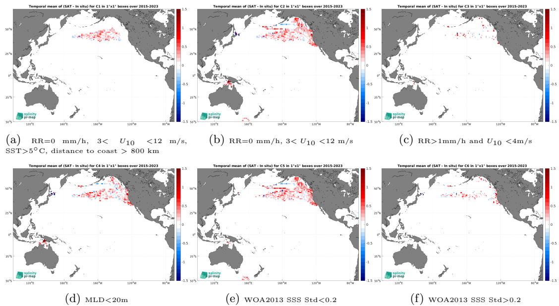
Figure 14: Temporal mean gridded over spatial boxes of size 1^\circ \times 1^\circ of \Delta SSS (SMAP SSS L3 v5.0 - 8-Day running (JPL) - Marine mammals) for 6 different subdatasets corresponding to:RR=0 mm/h, 3 < U_{10} < 12 m/s, SST > 5^\circ\text{C} , distance to coast > 800 km (a), RR=0 mm/h, 3 < U_{10} < 12 m/s (b), RR > 1 mm/h and U_{10} < 4 m/s (c),MLD < 20 m (d),WOA2013 SSS Std < 0.2 (e),WOA2013 SSS Std > 0.2 (f).
