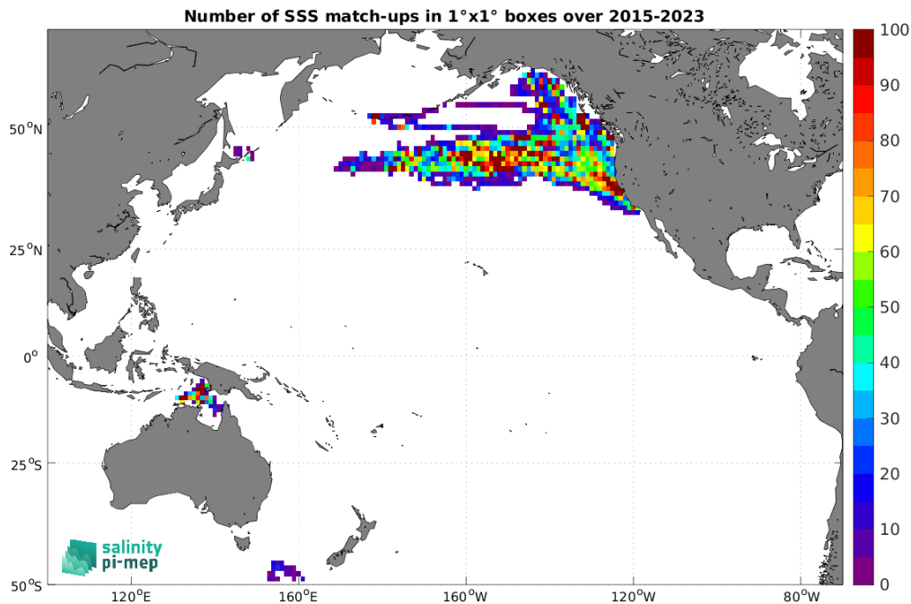
Figure 5: Number of SSS match-ups between Marine mammals SSS and the SMAP SSS L3 v5.0 - 8-Day running (JPL) SSS product for the Pacific Ocean Pi-MEP region over 1^\circ \times 1^\circ boxes and for the full satellite product period.
