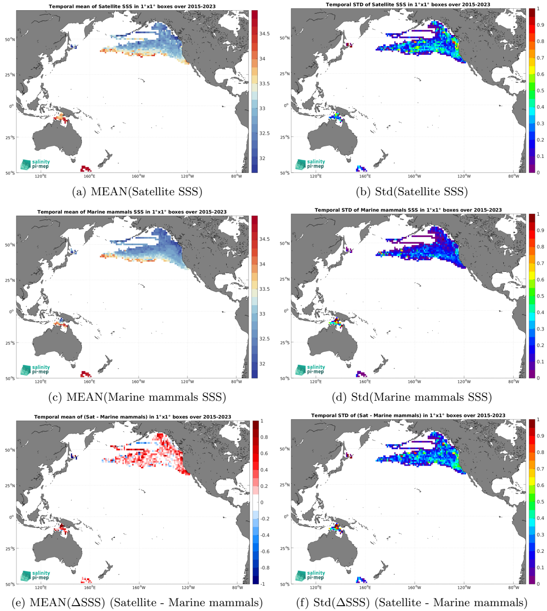
Figure 7: Temporal mean (left) and Std (right) of SSS from SMAP SSS L3 v5.0 - 8-Day running (JPL) (top), Marine mammals (middle), and of \Delta SSS (Satellite - Marine mammals). Only match-up pairs are used to generate these maps.
