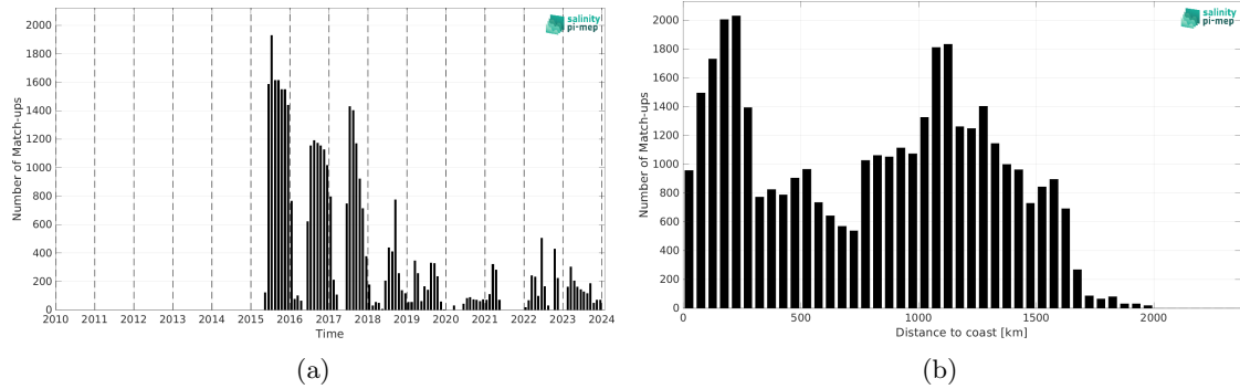
Figure 2: Number of match-ups between Marine mammals and SMAP SSS L3 v5.0 - 8-Day running (JPL) SSS as a function of time (a) and as function of the distance to coast (b) over the Pacific Ocean Pi-MEP region and for the full satellite product period.
