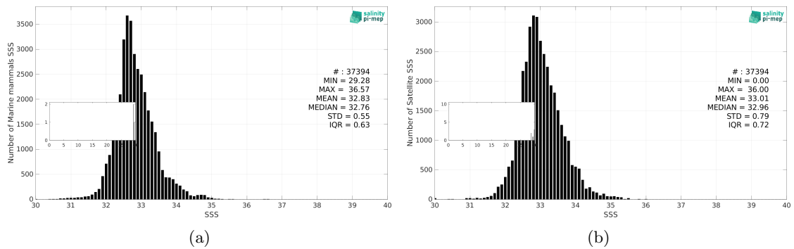
Figure 3: Histograms of SSS from Marine mammals (a) and SMAP SSS L3 v5.0 - 8-Day running (JPL) (b) considering all match-up pairs per bins of 0.1 over the Pacific Ocean Pi-MEP region and for the full satellite product period.
