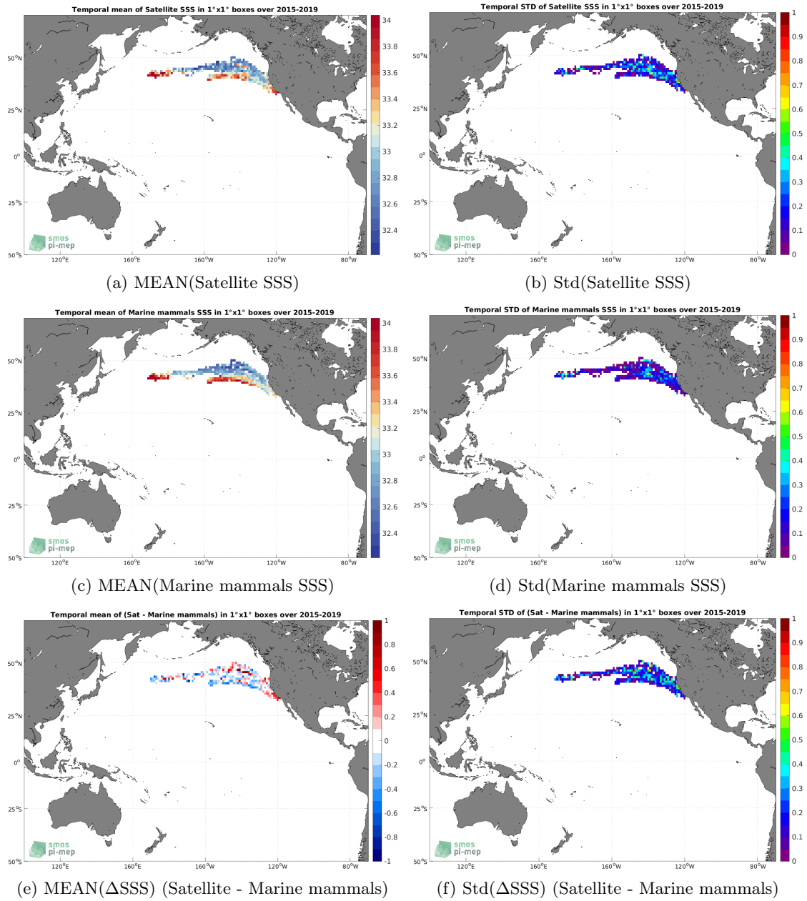
Figure 6: Temporal mean (left) and Std (right) of SSS from SMAP SSS L3 v5.0 - 8-Day running (JPL) (top), Marine mammals (middle), and of \Delta SSS (Satellite - Marine mammals). Only match-up pairs are used to generate these maps.
