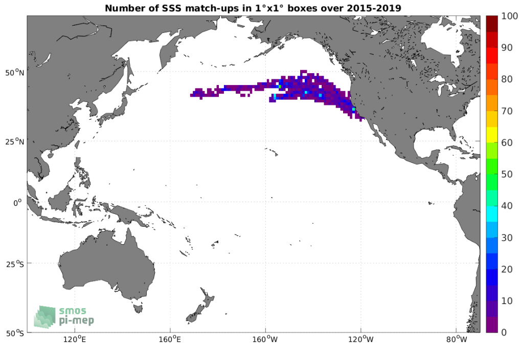
Figure 4: Number of SSS match-ups between Marine mammals SSS and the SMAP SSS L3 v5.0 - 8-Day running (JPL) SSS product for the Pacific Ocean Pi-MEP region over 1^\circ \times 1^\circ boxes and for the full satellite product period.
