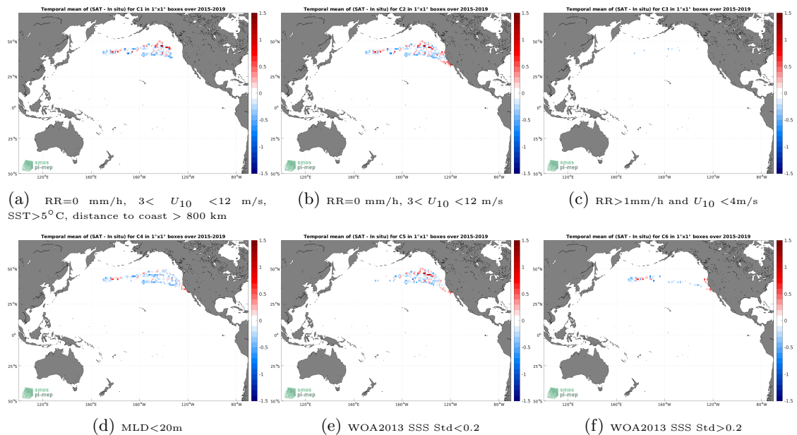
Figure 12: Temporal mean gridded over spatial boxes of size 1^\circ \times 1^\circ of \Delta SSS (SMAP SSS L3 v5.0 - 8-Day running (JPL) - Marine mammals) for 6 different subdatasets corresponding to:RR=0 mm/h, 3 < U_{10} < 12 m/s, SST > 5^\circ\text{C} , distance to coast > 800 km (a), RR=0 mm/h, 3 < U_{10} < 12 m/s (b), RR > 1 mm/h and U_{10} < 4 m/s (c),MLD < 20 m (d),WOA2013 SSS Std < 0.2 (e),WOA2013 SSS Std > 0.2 (f).
