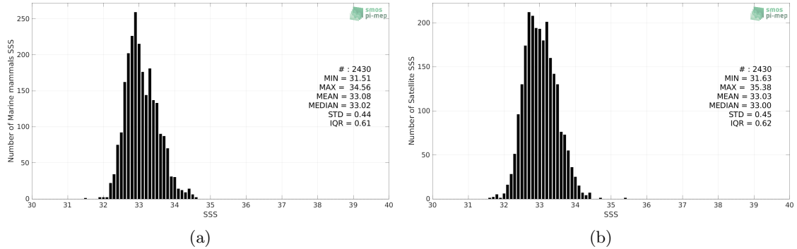
Figure 2: Histograms of SSS from Marine mammals (a) and SMAP SSS L3 v5.0 - 8-Day running (JPL) (b) considering all match-up pairs per bins of 0.1 over the Pacific Ocean Pi-MEP region and for the full satellite product period.
