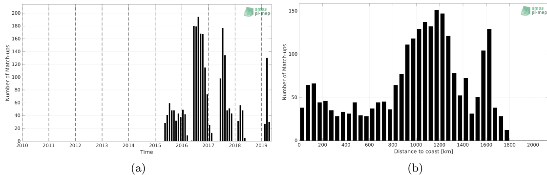
Figure 1: Number of match-ups between Marine mammals and SMAP SSS L3 v5.0 - 8-Day running (JPL) SSS as a function of time (a) and as function of the distance to coast (b) over the Pacific Ocean Pi-MEP region and for the full satellite product period.
