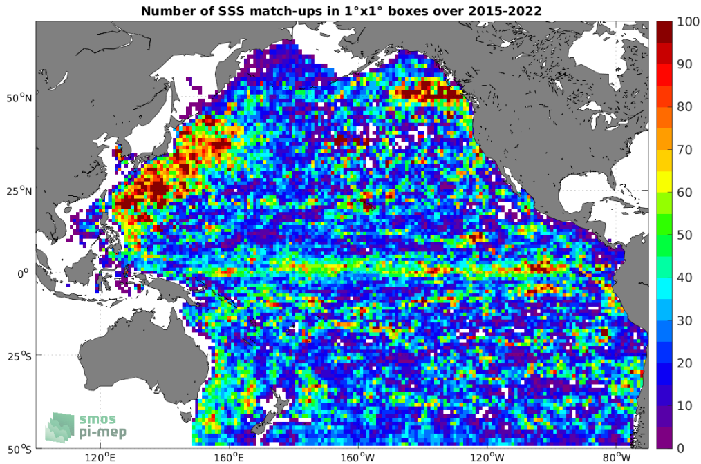
Figure 4: Number of SSS match-ups between Argo SSS and the SMAP SSS L3 v5.0 - 8-Day running (JPL) SSS product for the Pacific Ocean Pi-MEP region over 1^\circ \times 1^\circ boxes and for the full satellite product period.
