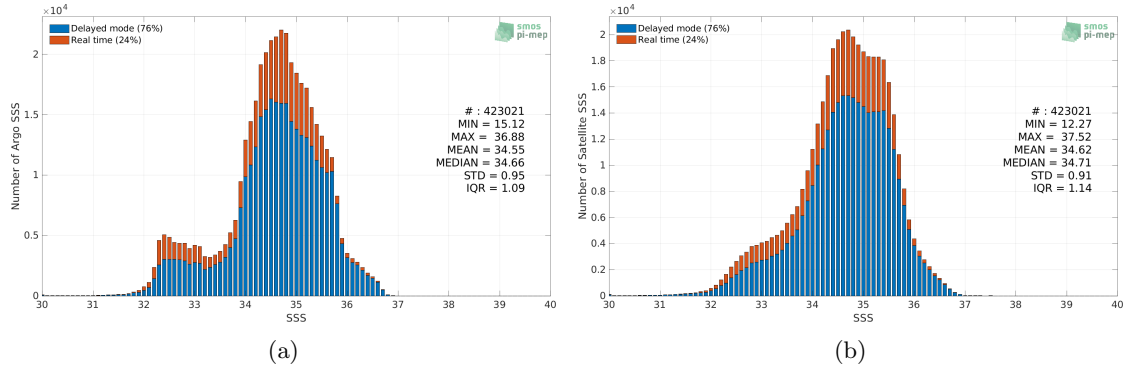
Figure 2: Histograms of SSS from Argo (a) and SMAP SSS L3 v5.0 - 8-Day running (JPL) (b) considering all match-up pairs per bins of 0.1 over the Pacific Ocean Pi-MEP region and for the full satellite product period.
