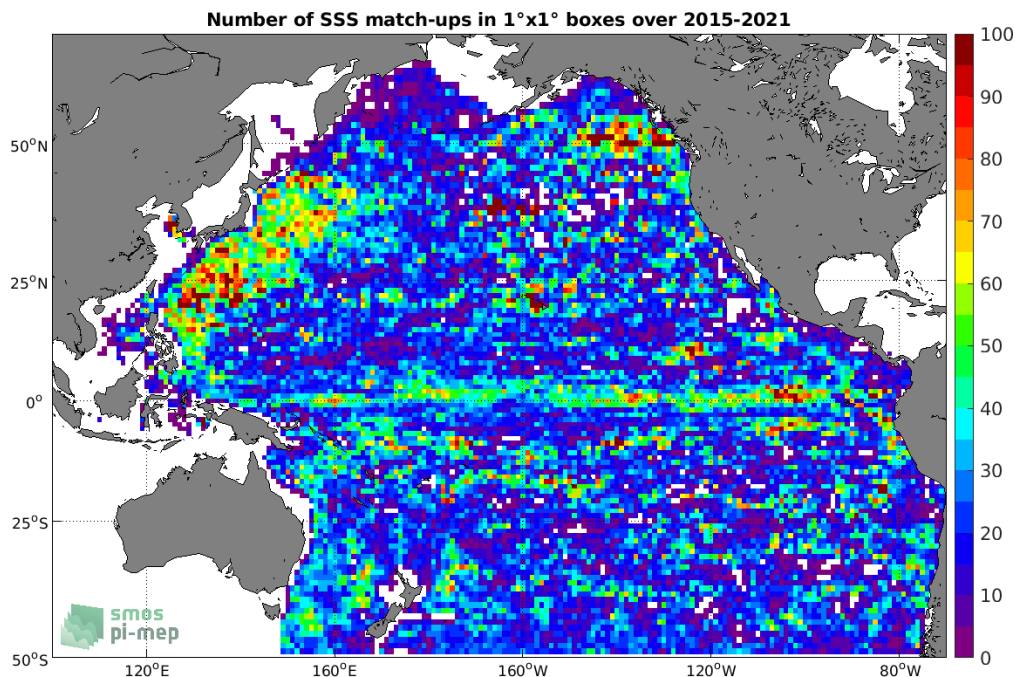
Figure 4: Number of SSS match-ups between Argo SSS and the SMAP SSS L3 v5.0 - 8-Day running (JPL) SSS product for the Pacific Ocean Pi-MEP region over 1°x1° boxes and for the full satellite product period.
