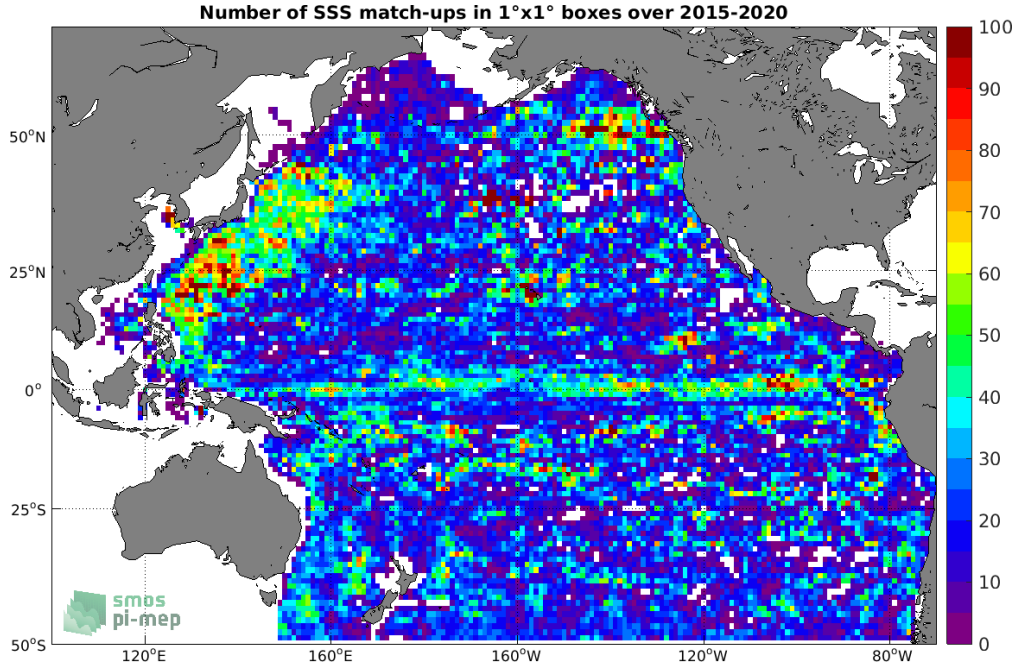
Figure 4: Number of SSS match-ups between Argo SSS and the SMAP SSS L3 v5.0 - 8-Day running (JPL) SSS product for the Pacific Ocean Pi-MEP region over 1°x1° boxes and for the full satellite product period.
