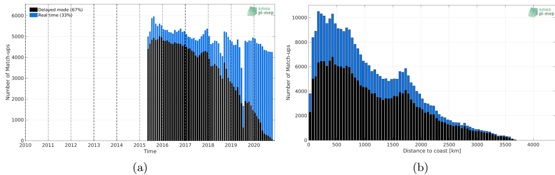
Figure 1: Number of match-ups between Argo and SMAP SSS L3 v5.0 - 8-Day running (JPL) SSS as a function of time (a) and as function of the distance to coast (b) over the Pacific Ocean Pi-MEP region and for the full satellite product period.
