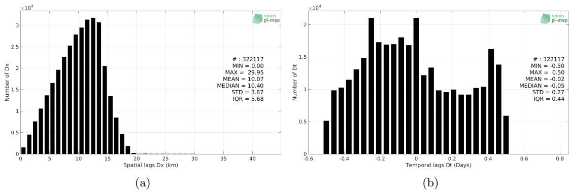
Figure 5: Histograms of the spatial (a) and temporal (b) lags between the time of the Argo measurements and the date of the corresponding SMAP SSS L3 v5.0 - 8-Day running (JPL) SSS product.
