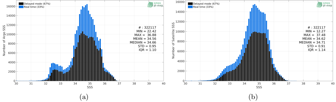
Figure 2: Histograms of SSS from Argo (a) and SMAP SSS L3 v5.0 - 8-Day running (JPL) (b) considering all match-up pairs per bins of 0.1 over the Pacific Ocean Pi-MEP region and for the full satellite product period.
