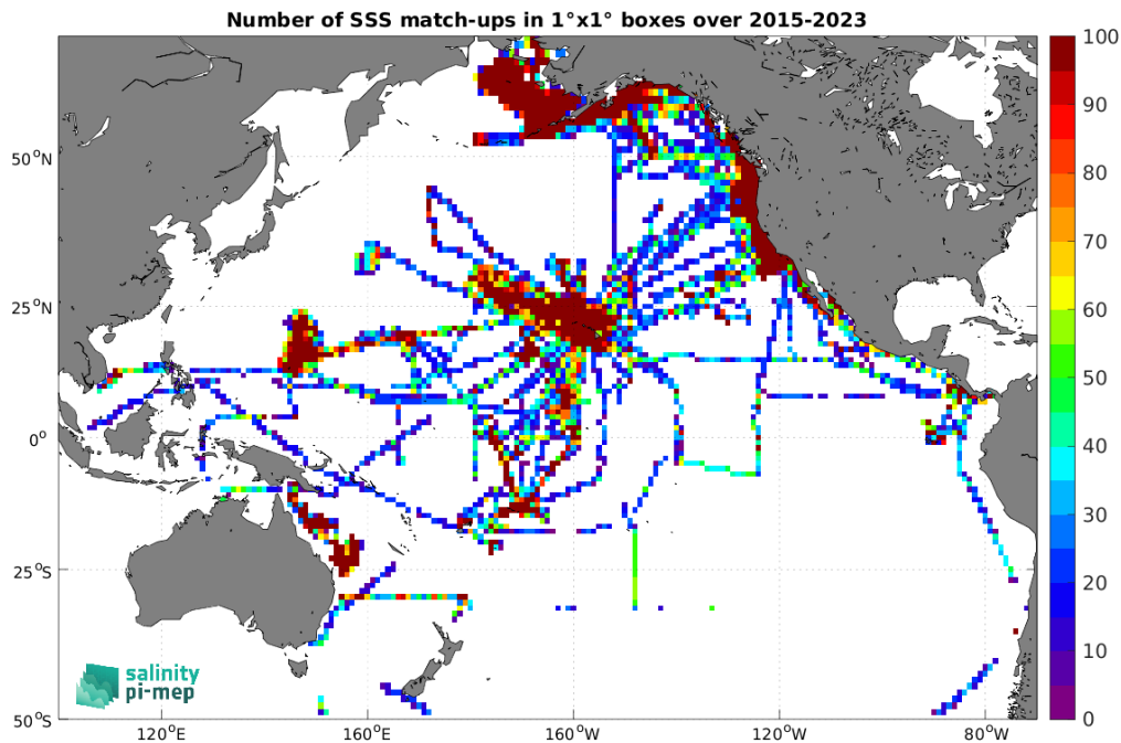
Figure 5: Number of SSS match-ups between TSG (SAMOS) SSS and the SMAP SSS L3 v5.0 - Monthly (JPL) SSS product for the Pacific Ocean Pi-MEP region over 1^\circ \times 1^\circ boxes and for the full satellite product period.
