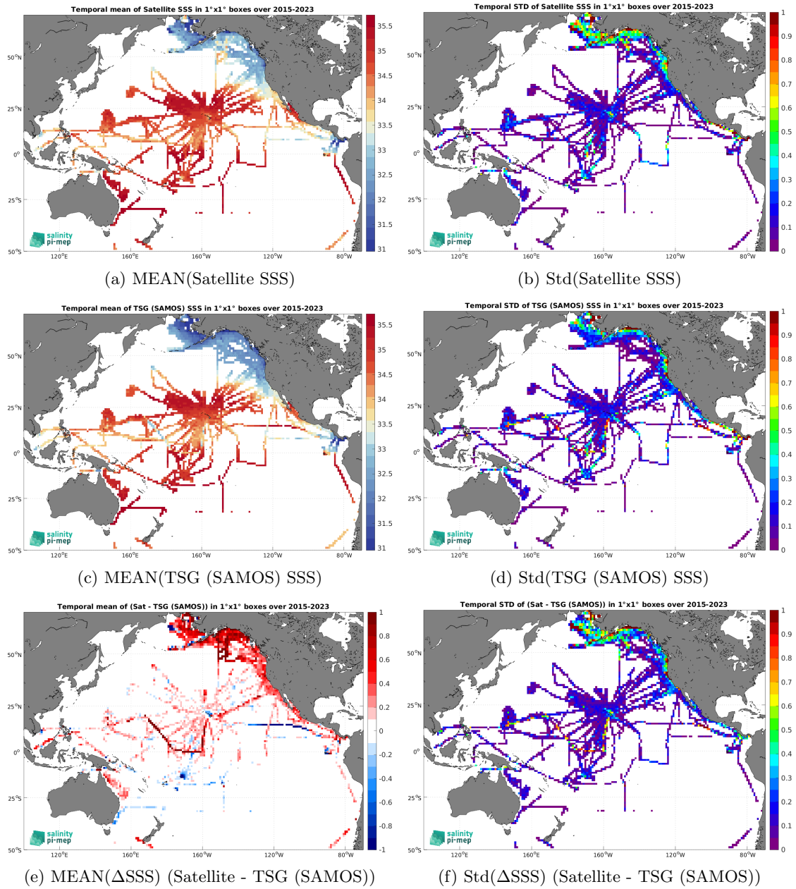
Figure 7: Temporal mean (left) and Std (right) of SSS from SMAP SSS L3 v5.0 - Monthly (JPL) (top), TSG (SAMOS) (middle), and of \Delta SSS (Satellite - TSG (SAMOS)). Only match-up pairs are used to generate these maps.
