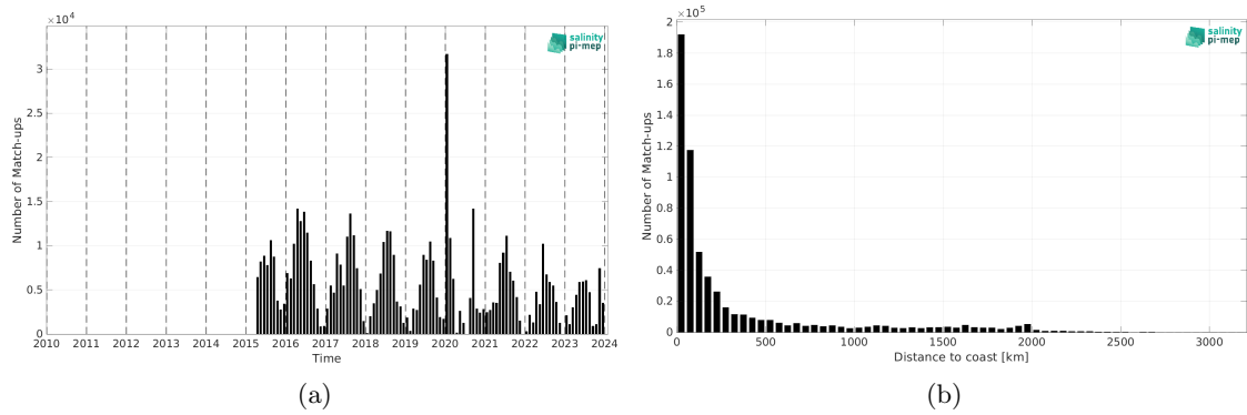
Figure 2: Number of match-ups between TSG (SAMOS) and SMAP SSS L3 v5.0 - Monthly (JPL) SSS as a function of time (a) and as function of the distance to coast (b) over the Pacific Ocean Pi-MEP region and for the full satellite product period.
