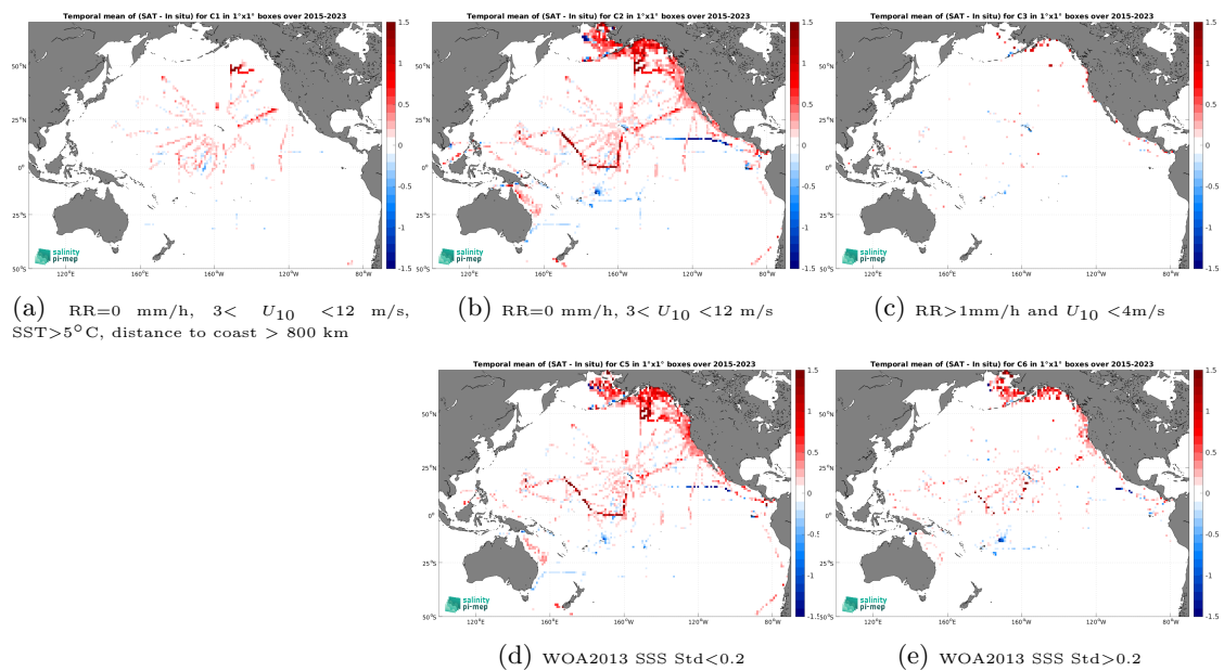
Figure 14: Temporal mean gridded over spatial boxes of size 1^\circ \times 1^\circ of \Delta SSS (SMAP SSS L3 v5.0 - Monthly (JPL) - TSG (SAMOS)) for 5 different subdatasets corresponding to:RR=0 mm/h, 3 < U_{10} < 12 m/s, SST > 5^\circ\text{C} , distance to coast > 800 km (a), RR=0 mm/h, 3 < U_{10} < 12 m/s (b), RR > 1 mm/h and U_{10} < 4 m/s (c), WOA2013 SSS Std < 0.2 (d), WOA2013 SSS Std > 0.2 (e).
