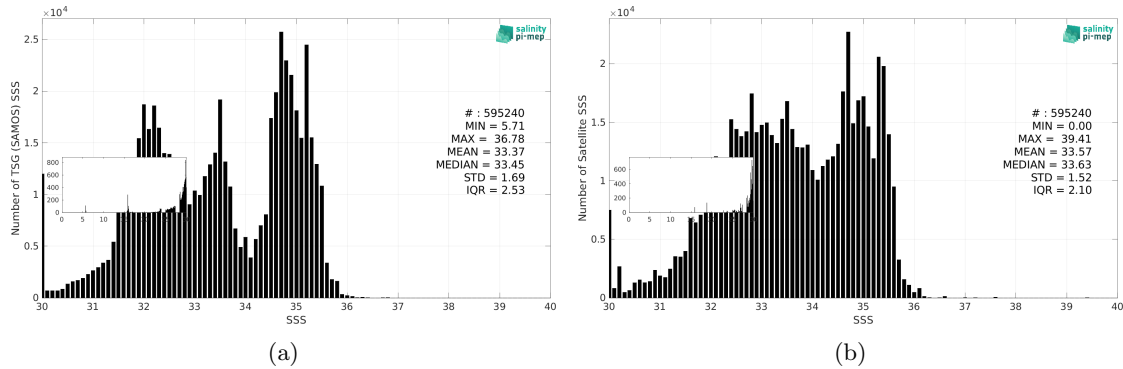
Figure 3: Histograms of SSS from TSG (SAMOS) (a) and SMAP SSS L3 v5.0 - Monthly (JPL) (b) considering all match-up pairs per bins of 0.1 over the Pacific Ocean Pi-MEP region and for the full satellite product period.
