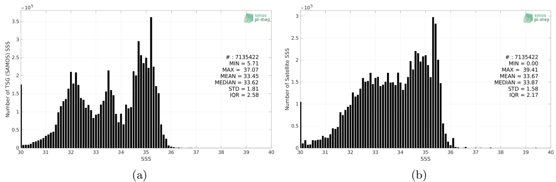
Figure 2: Histograms of SSS from TSG (SAMOS) (a) and SMAP SSS L3 v5.0 - Monthly (JPL) (b) considering all match-up pairs per bins of 0.1 over the Pacific Ocean Pi-MEP region and for the full satellite product period.
