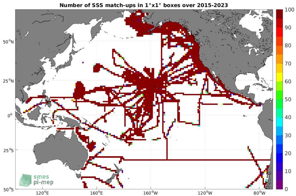
Figure 4: Number of SSS match-ups between TSG (SAMOS) SSS and the SMAP SSS L3 v5.0 - Monthly (JPL) SSS product for the Pacific Ocean Pi-MEP region over 1^\circ \times 1^\circ boxes and for the full satellite product period.
