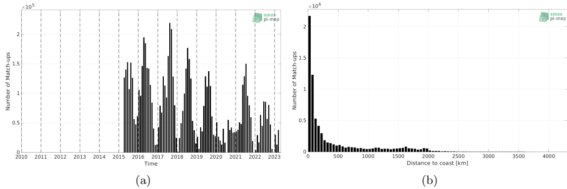
Figure 1: Number of match-ups between TSG (SAMOS) and SMAP SSS L3 v5.0 - Monthly (JPL) SSS as a function of time (a) and as function of the distance to coast (b) over the Pacific Ocean Pi-MEP region and for the full satellite product period.
