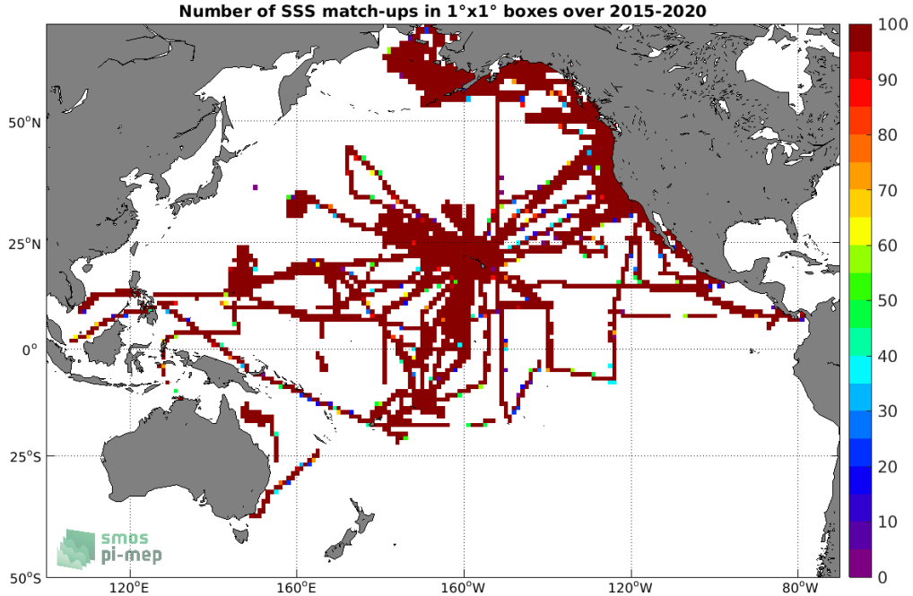
Figure 4: Number of SSS match-ups between TSG (SAMOS) SSS and the SMAP SSS L3 v5.0 - Monthly (JPL) SSS product for the Pacific Ocean Pi-MEP region over 1°x1° boxes and for the full satellite product period.
