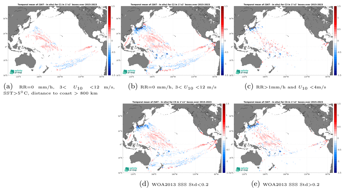
Figure 14: Temporal mean gridded over spatial boxes of size 1^\circ \times 1^\circ of \Delta SSS (SMAP SSS L3 v5.0 - Monthly (JPL) - TSG (LEGOS-DM)) for 5 different subdatasets corresponding to: RR=0 mm/h, 3 < U_{10} < 12 m/s, SST > 5°C, distance to coast > 800 km (a), RR=0 mm/h, 3 < U_{10} < 12 m/s (b), RR > 1mm/h and U_{10} < 4 m/s (c), WOA2013 SSS Std < 0.2 (d), WOA2013 SSS Std > 0.2 (e).
