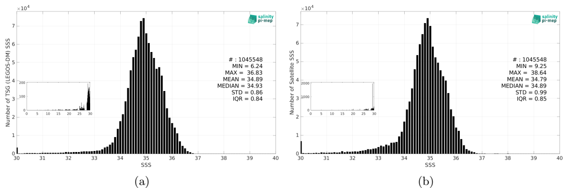
Figure 3: Histograms of SSS from TSG (LEGOS-DM) (a) and SMAP SSS L3 v5.0 - Monthly (JPL) (b) considering all match-up pairs per bins of 0.1 over the Pacific Ocean Pi-MEP region and for the full satellite product period.
