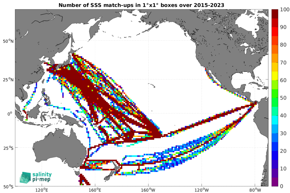
Figure 5: Number of SSS match-ups between TSG (LEGOS-DM) SSS and the SMAP SSS L3 v5.0 - Monthly (JPL) SSS product for the Pacific Ocean Pi-MEP region over 1^\circ \times 1^\circ boxes and for the full satellite product period.
