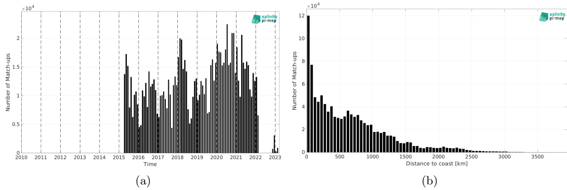
Figure 2: Number of match-ups between TSG (LEGOS-DM) and SMAP SSS L3 v5.0 - Monthly (JPL) SSS as a function of time (a) and as function of the distance to coast (b) over the Pacific Ocean Pi-MEP region and for the full satellite product period.
