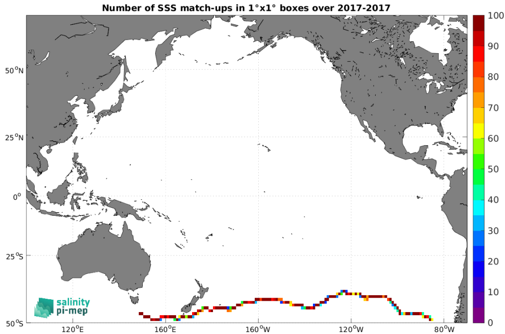
Figure 5: Number of SSS match-ups between TSG (GOSUD-Sailing-ship) SSS and the SMAP SSS L3 v5.0 - Monthly (JPL) SSS product for the Pacific Ocean Pi-MEP region over 1^\circ \times 1^\circ boxes and for the full satellite product period.
