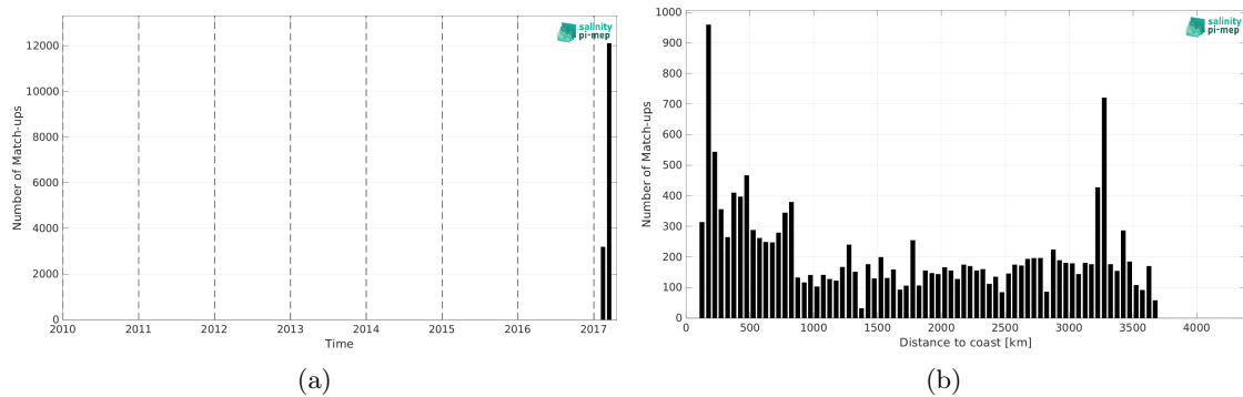
Figure 2: Number of match-ups between TSG (GOSUD-Sailing-ship) and SMAP SSS L3 v5.0 - Monthly (JPL) SSS as a function of time (a) and as function of the distance to coast (b) over the Pacific Ocean Pi-MEP region and for the full satellite product period.
