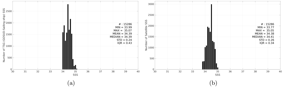
Figure 3: Histograms of SSS from TSG (GOSUD-Sailing-ship) (a) and SMAP SSS L3 v5.0 - Monthly (JPL) (b) considering all match-up pairs per bins of 0.1 over the Pacific Ocean Pi-MEP region and for the full satellite product period.
