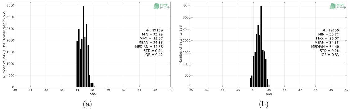
Figure 2: Histograms of SSS from TSG (GOSUD-Sailing-ship) (a) and SMAP SSS L3 v5.0 - Monthly (JPL) (b) considering all match-up pairs per bins of 0.1 over the Pacific Ocean Pi-MEP region and for the full satellite product period.
