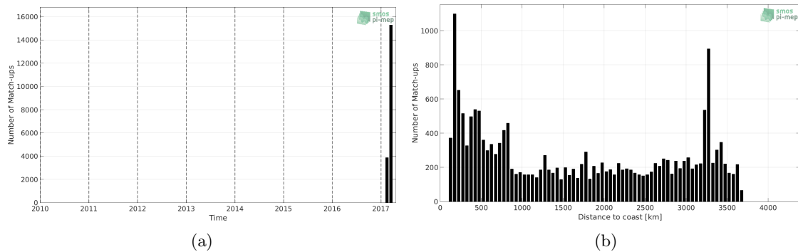
Figure 1: Number of match-ups between TSG (GOSUD-Sailing-ship) and SMAP SSS L3 v5.0 - Monthly (JPL) SSS as a function of time (a) and as function of the distance to coast (b) over the Pacific Ocean Pi-MEP region and for the full satellite product period.
