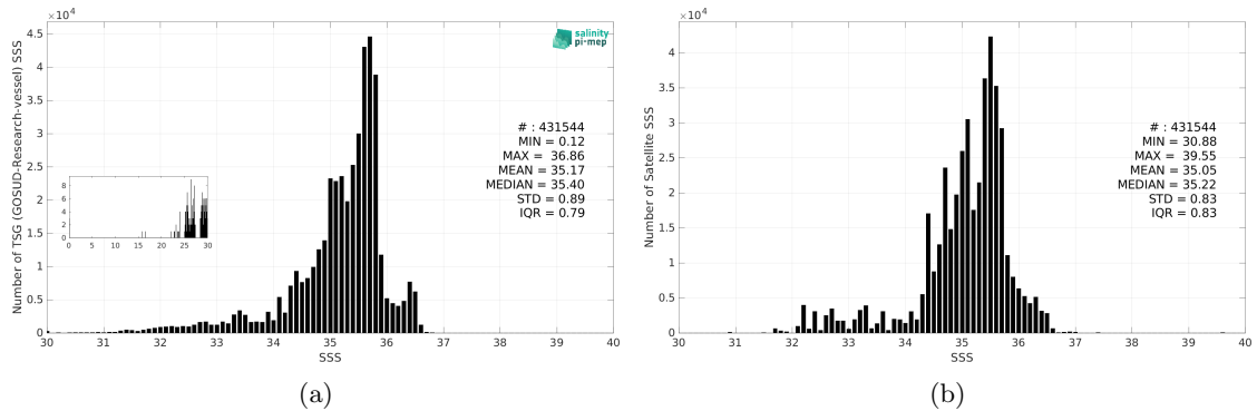
Figure 3: Histograms of SSS from TSG (GOSUD-Research-vessel) (a) and SMAP SSS L3 v5.0 - Monthly (JPL) (b) considering all match-up pairs per bins of 0.1 over the Pacific Ocean Pi-MEP region and for the full satellite product period.
