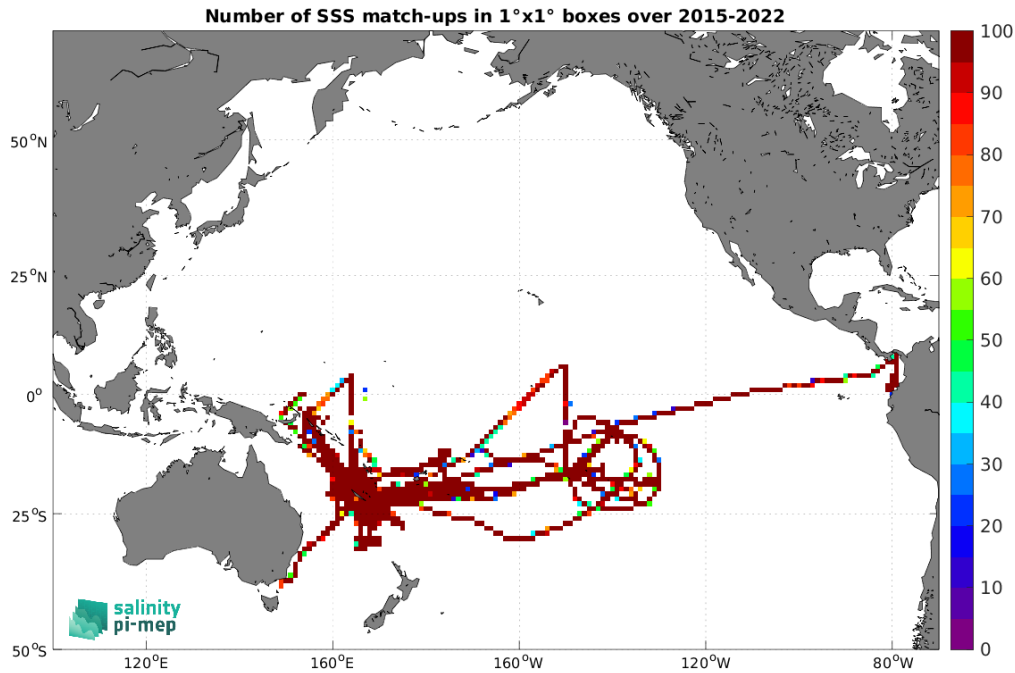
Figure 5: Number of SSS match-ups between TSG (GOSUD-Research-vessel) SSS and the SMAP SSS L3 v5.0 - Monthly (JPL) SSS product for the Pacific Ocean Pi-MEP region over 1^\circ \times 1^\circ boxes and for the full satellite product period.
