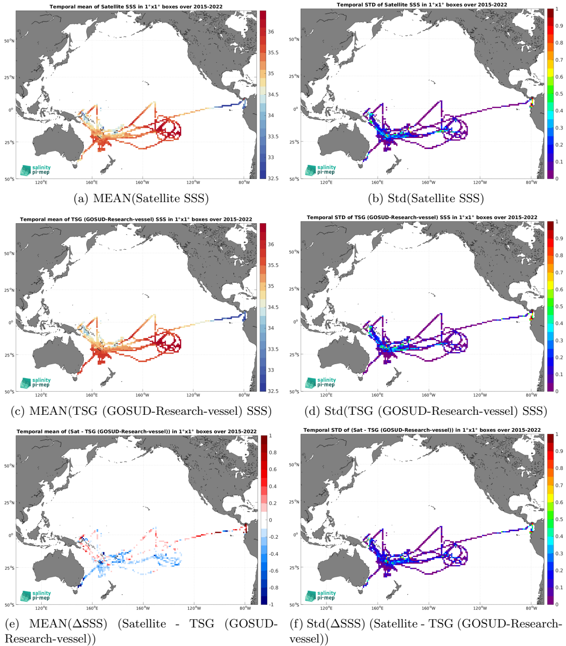
Figure 7: Temporal mean (left) and Std (right) of SSS from SMAP SSS L3 v5.0 - Monthly (JPL) (top), TSG (GOSUD-Research-vessel) (middle), and of \Delta SSS (Satellite - TSG (GOSUD-Research-vessel)). Only match-up pairs are used to generate these maps.
