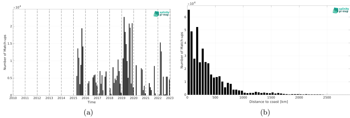
Figure 2: Number of match-ups between TSG (GOSUD-Research-vessel) and SMAP SSS L3 v5.0 - Monthly (JPL) SSS as a function of time (a) and as function of the distance to coast (b) over the Pacific Ocean Pi-MEP region and for the full satellite product period.
