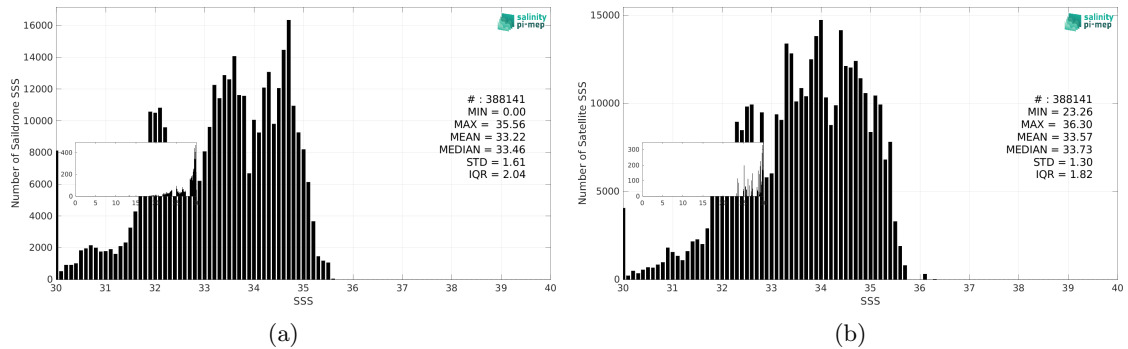
Figure 3: Histograms of SSS from Sairdrone (a) and SMAP SSS L3 v5.0 - Monthly (JPL) (b) considering all match-up pairs per bins of 0.1 over the Pacific Ocean Pi-MEP region and for the full satellite product period.
