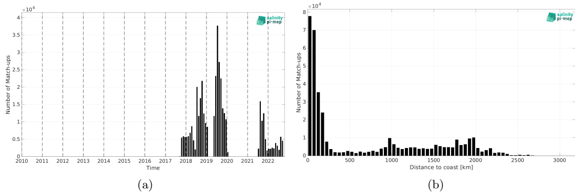
Figure 2: Number of match-ups between Sairdrone and SMAP SSS L3 v5.0 - Monthly (JPL) SSS as a function of time (a) and as function of the distance to coast (b) over the Pacific Ocean Pi-MEP region and for the full satellite product period.
