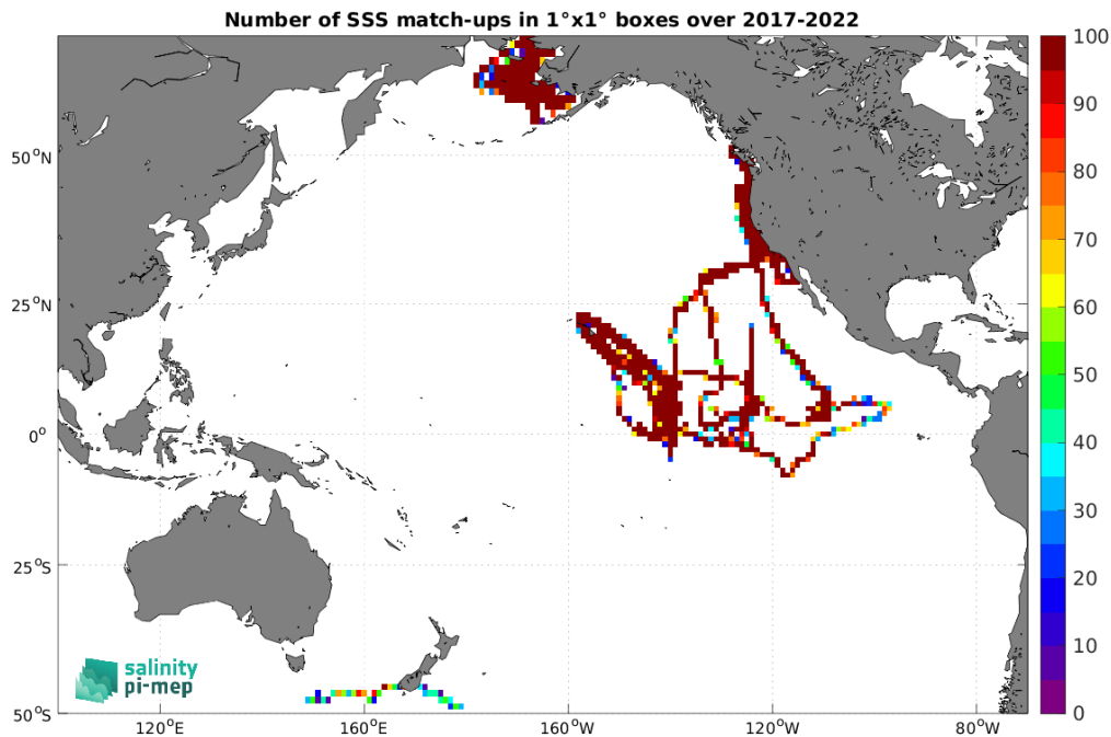
Figure 5: Number of SSS match-ups between Saildrone SSS and the SMAP SSS L3 v5.0 - Monthly (JPL) SSS product for the Pacific Ocean Pi-MEP region over 1^\circ \times 1^\circ boxes and for the full satellite product period.
