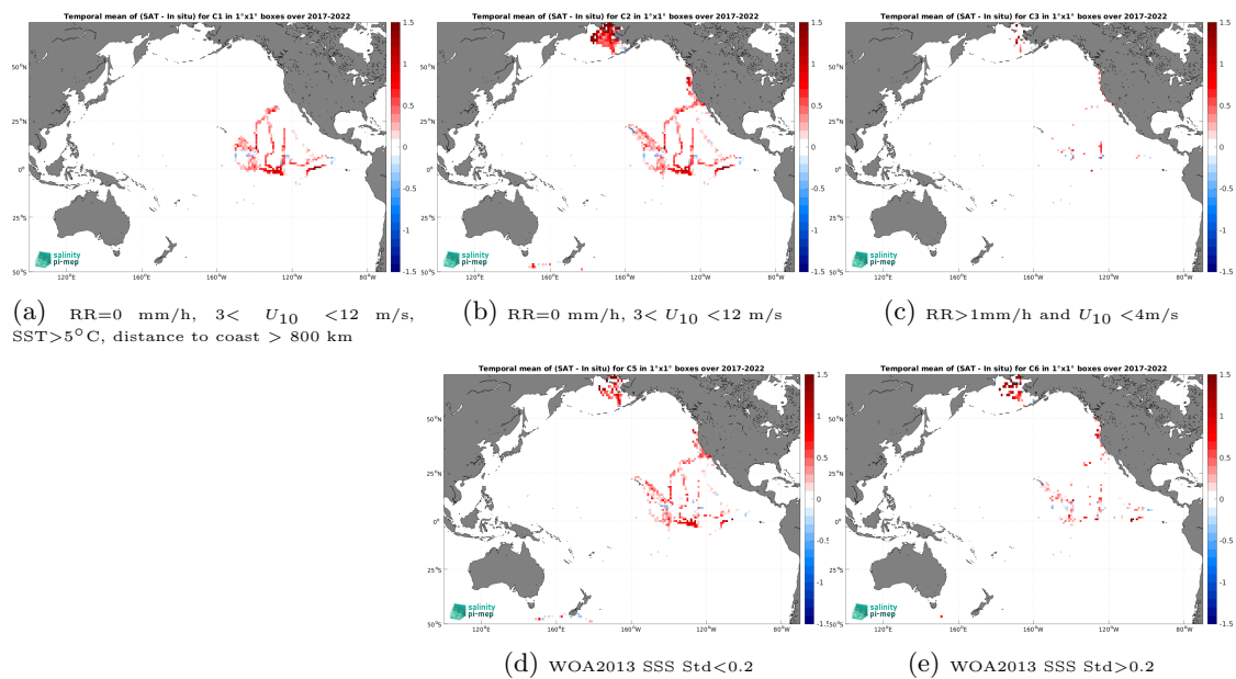
Figure 14: Temporal mean gridded over spatial boxes of size 1^\circ \times 1^\circ of \Delta SSS (SMAP SSS L3 v5.0 - Monthly (JPL) - Sairdrone) for 5 different subdatasets corresponding to:RR=0 mm/h, 3 < U_{10} < 12 m/s, SST > 5^\circ\text{C} , distance to coast > 800 km (a), RR=0 mm/h, 3 < U_{10} < 12 m/s (b), RR > 1 mm/h and U_{10} < 4 m/s (c), WOA2013 SSS Std < 0.2 (d), WOA2013 SSS Std > 0.2 (e).
