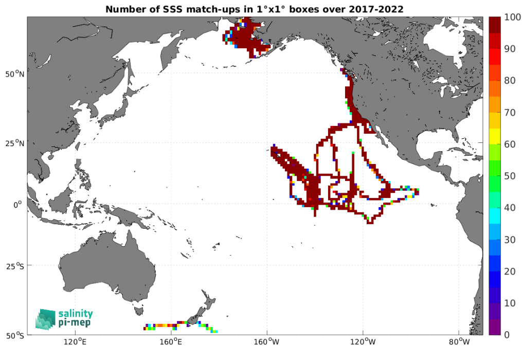
Figure 4: Number of SSS match-ups between Saildrone SSS and the SMAP SSS L3 v5.0 - Monthly (JPL) SSS product for the Pacific Ocean Pi-MEP region over 1^\circ \times 1^\circ boxes and for the full satellite product period.
