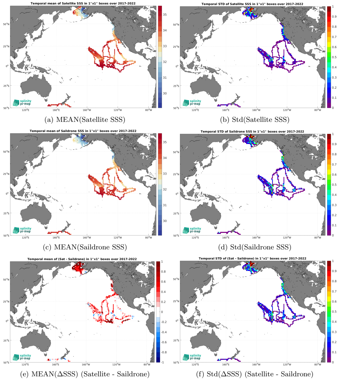
Figure 6: Temporal mean (left) and Std (right) of SSS from SMAP SSS L3 v5.0 - Monthly (JPL) (top), Saildrone (middle), and of \Delta SSS (Satellite - Saildrone). Only match-up pairs are used to generate these maps.
