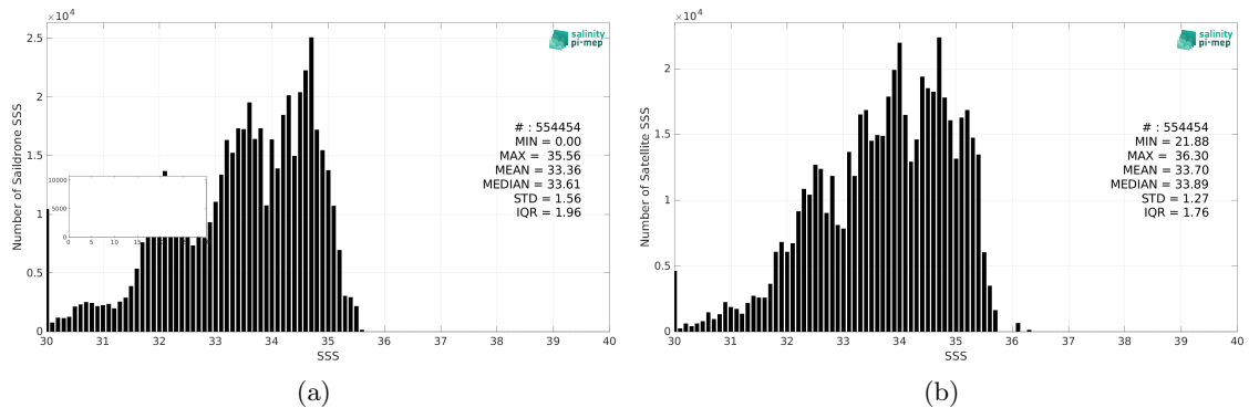
Figure 2: Histograms of SSS from Sairdrone (a) and SMAP SSS L3 v5.0 - Monthly (JPL) (b) considering all match-up pairs per bins of 0.1 over the Pacific Ocean Pi-MEP region and for the full satellite product period.
