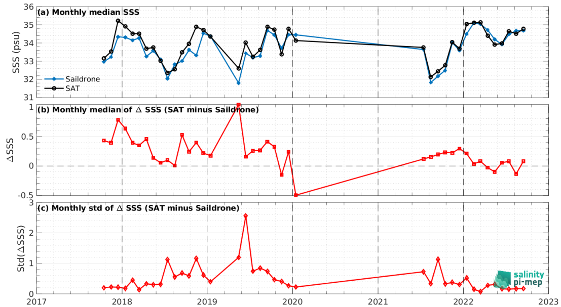
Figure 7: Time series of the monthly median SSS (top), median of \Delta\text{SSS} (Satellite - SSS) and Std of \Delta\text{SSS} (Satellite - SSS) over the Pacific Ocean Pi-MEP region considering all match-ups collected by the Pi-MEP.
