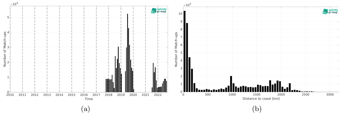
Figure 1: Number of match-ups between Sairdrone and SMAP SSS L3 v5.0 - Monthly (JPL) SSS as a function of time (a) and as function of the distance to coast (b) over the Pacific Ocean Pi-MEP region and for the full satellite product period.
