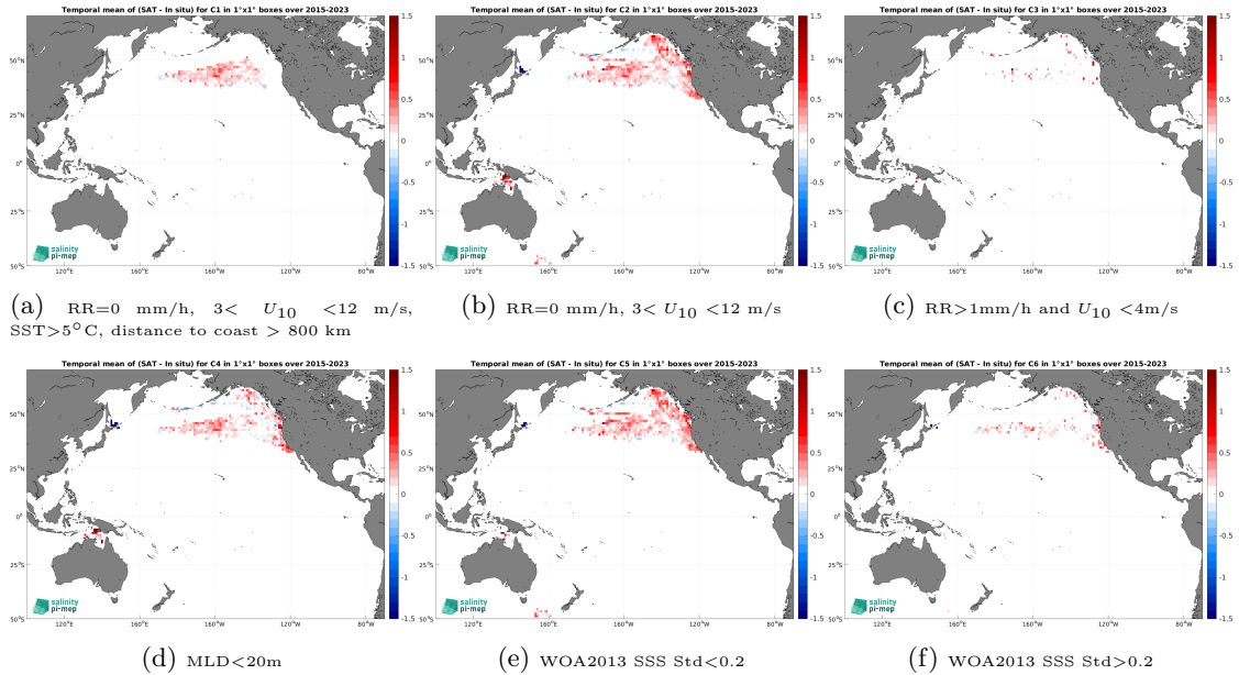
Figure 14: Temporal mean gridded over spatial boxes of size 1^\circ \times 1^\circ of \Delta SSS (SMAP SSS L3 v5.0 - Monthly (JPL) - Marine mammals) for 6 different subdatasets corresponding to:RR=0 mm/h, 3 < U_{10} < 12 m/s, SST>5°C, distance to coast > 800 km (a), RR=0 mm/h, 3 < U_{10} < 12 m/s (b), RR>1mm/h and U_{10} < 4 m/s (c),MLD<20m (d),WOA2013 SSS Std<0.2 (e),WOA2013 SSS Std>0.2 (f).
