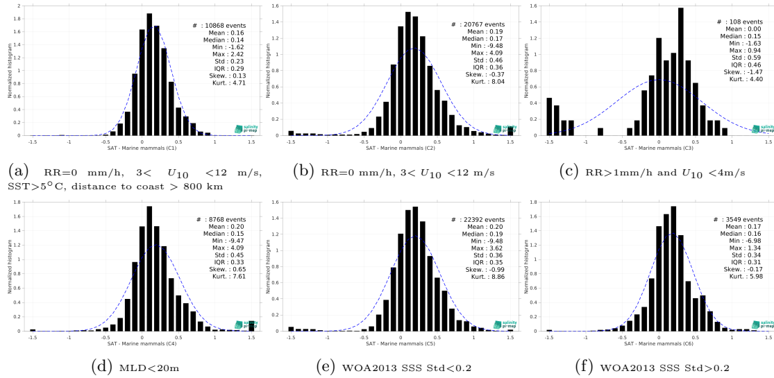
Figure 15: Normalized histogram of \Delta SSS (SMAP SSS L3 v5.0 - Monthly (JPL) - Marine mammals) for 6 different subdatasets corresponding to: RR=0 mm/h, 3 < U_{10} < 12 m/s, SST > 5°C, distance to coast > 800 km (a), RR=0 mm/h, 3 < U_{10} < 12 m/s (b), RR > 1mm/h and U_{10} < 4 m/s (c), MLD < 20m (d), WOA2013 SSS Std < 0.2 (e), WOA2013 SSS Std > 0.2 (f).
