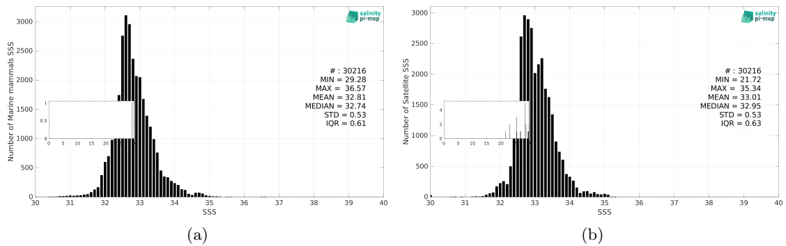
Figure 3: Histograms of SSS from Marine mammals (a) and SMAP SSS L3 v5.0 - Monthly (JPL) (b) considering all match-up pairs per bins of 0.1 over the Pacific Ocean Pi-MEP region and for the full satellite product period.
