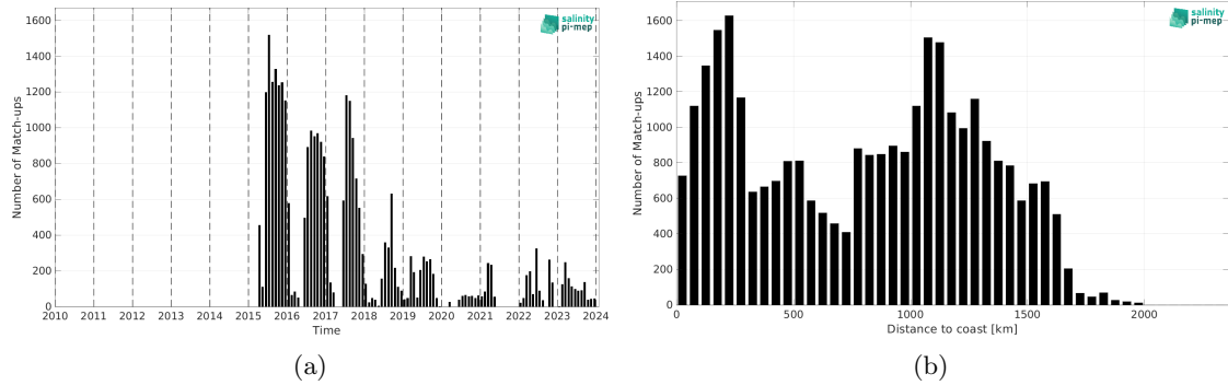
Figure 2: Number of match-ups between Marine mammals and SMAP SSS L3 v5.0 - Monthly (JPL) SSS as a function of time (a) and as function of the distance to coast (b) over the Pacific Ocean Pi-MEP region and for the full satellite product period.
