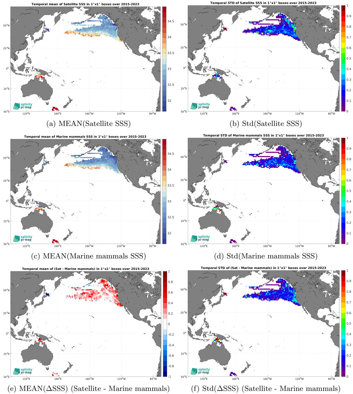
Figure 7: Temporal mean (left) and Std (right) of SSS from SMAP SSS L3 v5.0 - Monthly (JPL) (top), Marine mammals (middle), and of \Delta SSS (Satellite - Marine mammals). Only match-up pairs are used to generate these maps.
