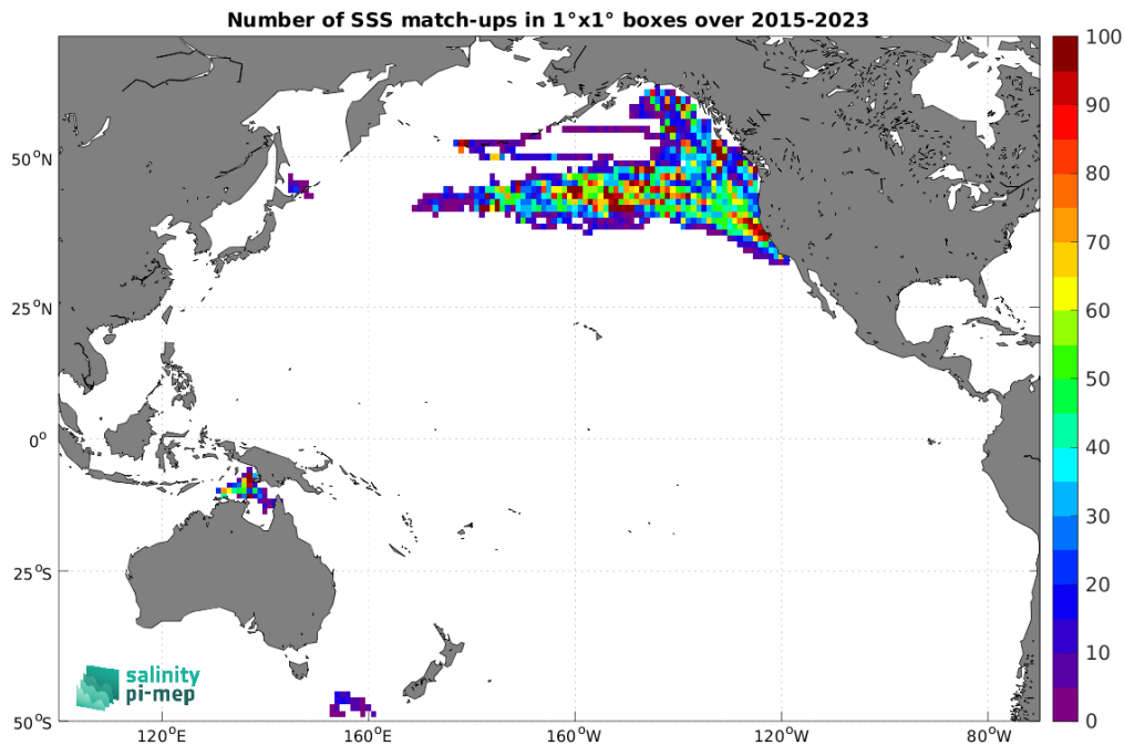
Figure 5: Number of SSS match-ups between Marine mammals SSS and the SMAP SSS L3 v5.0 - Monthly (JPL) SSS product for the Pacific Ocean Pi-MEP region over 1^\circ \times 1^\circ boxes and for the full satellite product period.
