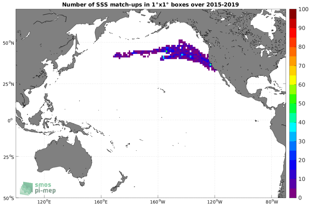
Figure 4: Number of SSS match-ups between Marine mammals SSS and the SMAP SSS L3 v5.0 - Monthly (JPL) SSS product for the Pacific Ocean Pi-MEP region over 1^{\circ} \times 1^{\circ} boxes and for the full satellite product period.
