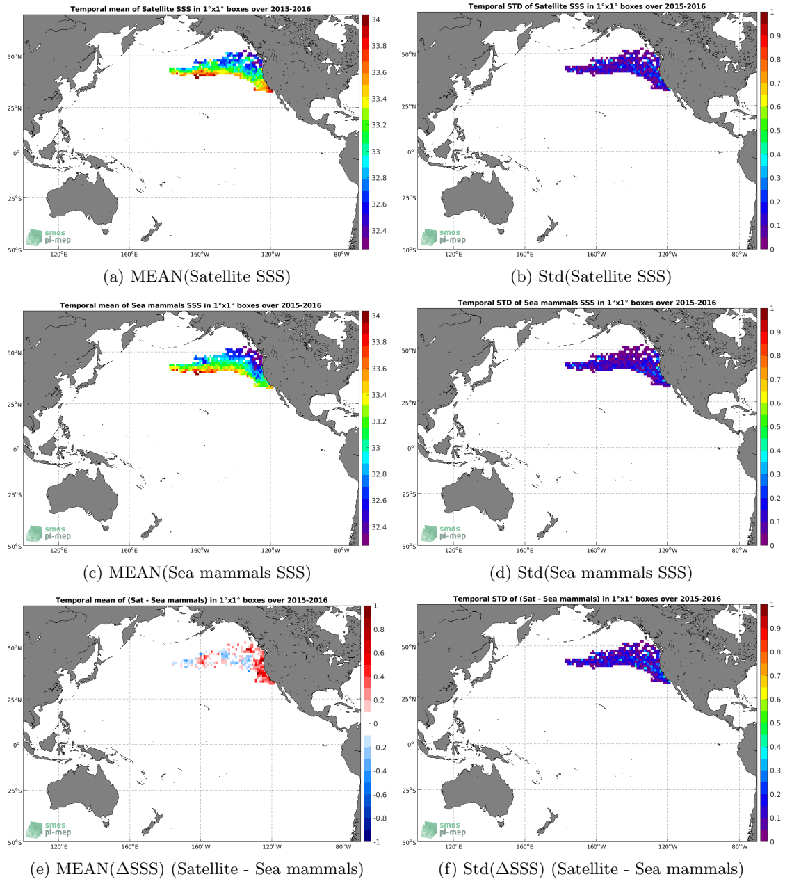
Figure 6: Temporal mean (left) and Std (right) of SSS from SMAP SSS L3 v5.0 - Monthly (JPL) (top), Sea mammals (middle), and of \Delta SSS (Satellite - Sea mammals). Only match-up pairs are used to generate these maps.
