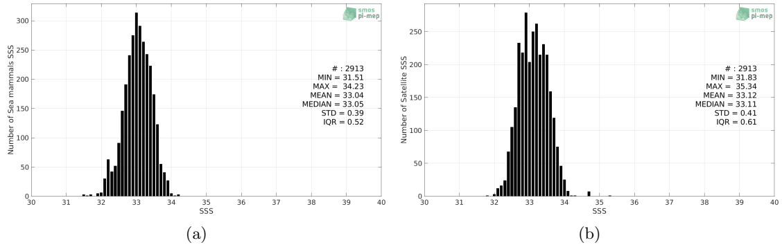
Figure 2: Histograms of SSS from Sea mammals (a) and SMAP SSS L3 v5.0 - Monthly (JPL) (b) considering all match-up pairs per bins of 0.1 over the Pacific Ocean Pi-MEP region and for the full satellite product period.
