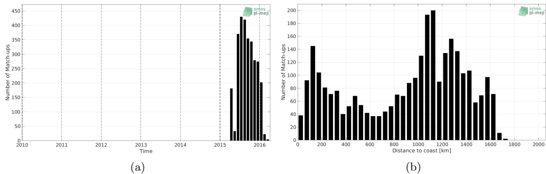
Figure 1: Number of match-ups between Sea mammals and SMAP SSS L3 v5.0 - Monthly (JPL) SSS as a function of time (a) and as function of the distance to coast (b) over the Pacific Ocean Pi-MEP region and for the full satellite product period.
