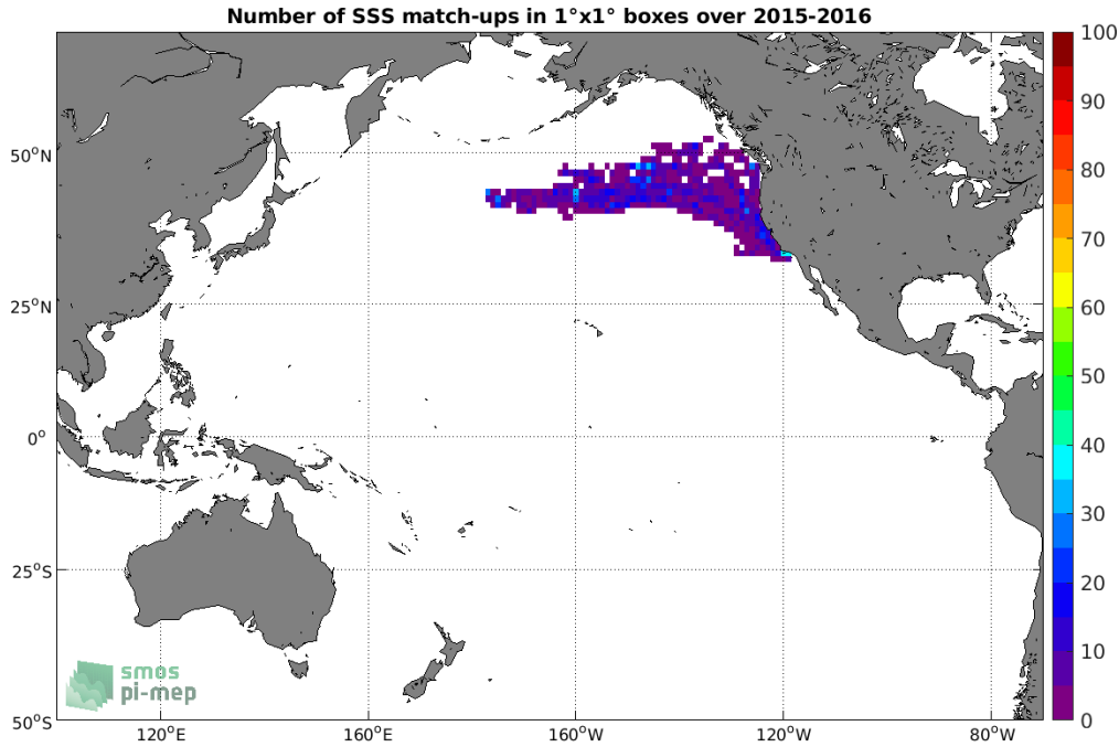
Figure 4: Number of SSS match-ups between Sea mammals SSS and the SMAP SSS L3 v5.0 - Monthly (JPL) SSS product for the Pacific Ocean Pi-MEP region over 1°x1° boxes and for the full satellite product period.
