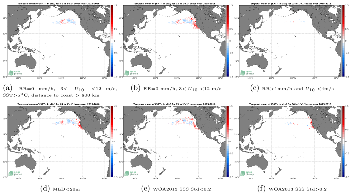
Figure 12: Temporal mean gridded over spatial boxes of size 1°x1° of \Delta SSS (SMAP SSS L3 v5.0 - Monthly (JPL) - Sea mammals) for 6 different subdatasets corresponding to:RR=0 mm/h, 3 < U_{10} < 12 m/s, SST>5°C, distance to coast > 800 km (a), RR=0 mm/h, 3 < U_{10} < 12 m/s (b), RR>1mm/h and U_{10} < 4 m/s (c),MLD<20m (d),WOA2013 SSS Std<0.2 (e),WOA2013 SSS Std>0.2 (f).
