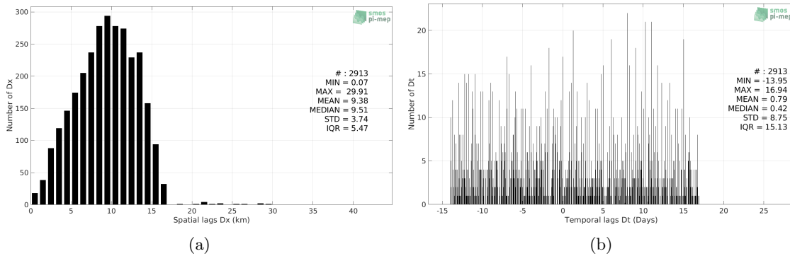
Figure 5: Histograms of the spatial (a) and temporal (b) lags between the location/time of the Sea mammals measurement and the date of the corresponding SMAP SSS L3 v5.0 - Monthly (JPL) SSS pixel.
