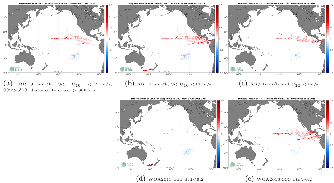
Figure 11: Temporal mean gridded over spatial boxes of size 1^\circ \times 1^\circ of \Delta\text{SSS} (SMAP SSS L3 v5.0 - Monthly (JPL) - Surface drifters) for 5 different subdatasets corresponding to:RR=0 mm/h, 3 < U_{10} < 12 m/s, SST >5^\circ\text{C} , distance to coast > 800 km (a), RR=0 mm/h, 3 < U_{10} < 12 m/s (b), RR >1 mm/h and U_{10} < 4 m/s (c), WOA2013 SSS Std <0.2 (d), WOA2013 SSS Std >0.2 (e).
