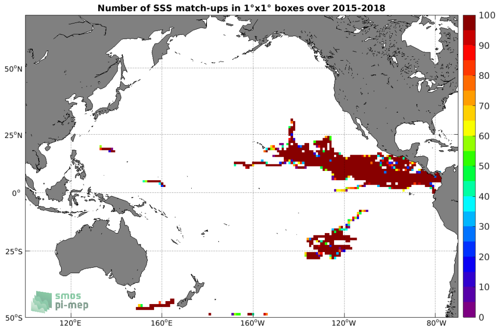
Figure 3: Number of SSS match-ups between Surface drifters SSS and the SMAP SSS L3 v5.0 - Monthly (JPL) SSS product for the Pacific Ocean Pi-MEP region over 1°x1° boxes and for the full satellite product period.
