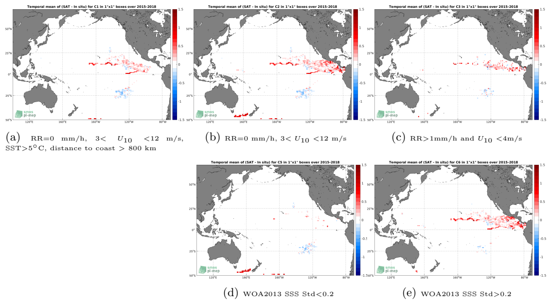
Figure 11: Temporal mean gridded over spatial boxes of size 1°x1° of \Delta SSS (SMAP SSS L3 v5.0 - Monthly (JPL) - Surface drifters) for 5 different subdatasets corresponding to:RR=0 mm/h, 3 < U_{10} < 12 m/s, SST>5°C, distance to coast > 800 km (a), RR=0 mm/h, 3 < U_{10} < 12 m/s (b), RR>1mm/h and U_{10} < 4 m/s (c), WOA2013 SSS Std<0.2 (d), WOA2013 SSS Std>0.2 (e).
