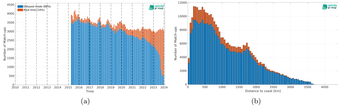
Figure 2: Number of match-ups between Argo and SMAP SSS L3 v5.0 - Monthly (JPL) SSS as a function of time (a) and as function of the distance to coast (b) over the Pacific Ocean Pi-MEP region and for the full satellite product period.
