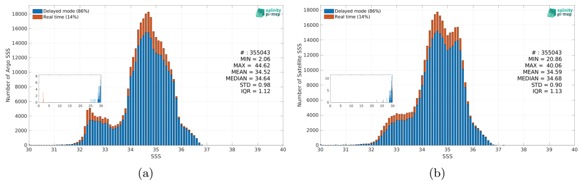
Figure 3: Histograms of SSS from Argo (a) and SMAP SSS L3 v5.0 - Monthly (JPL) (b) considering all match-up pairs per bins of 0.1 over the Pacific Ocean Pi-MEP region and for the full satellite product period.
