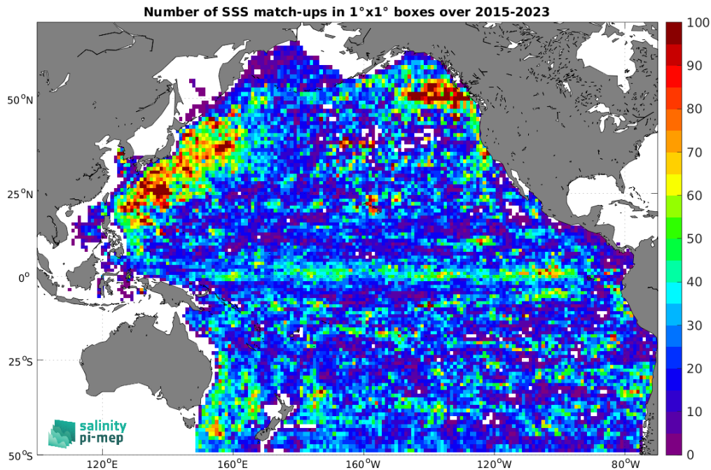
Figure 5: Number of SSS match-ups between Argo SSS and the SMAP SSS L3 v5.0 - Monthly (JPL) SSS product for the Pacific Ocean Pi-MEP region over 1^\circ \times 1^\circ boxes and for the full satellite product period.
