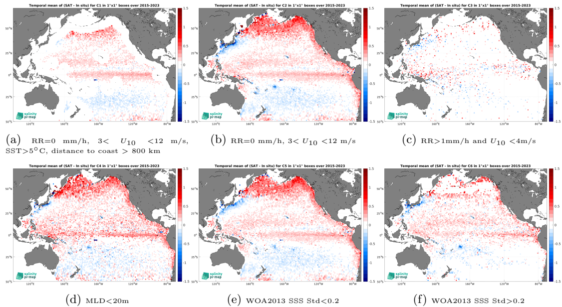
Figure 14: Temporal mean gridded over spatial boxes of size 1^\circ \times 1^\circ of \Delta SSS (SMAP SSS L3 v5.0 - Monthly (JPL) - Argo) for 6 different subdatasets corresponding to:RR=0 mm/h, 3 < U_{10} < 12 m/s, SST > 5^\circ\text{C} , distance to coast > 800 km (a), RR=0 mm/h, 3 < U_{10} < 12 m/s (b), RR > 1 mm/h and U_{10} < 4 m/s (c),MLD < 20 m (d),WOA2013 SSS Std < 0.2 (e),WOA2013 SSS Std > 0.2 (f).
