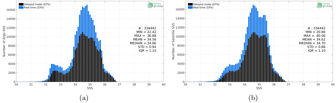
Figure 2: Histograms of SSS from Argo (a) and SMAP SSS L3 v5.0 - Monthly (JPL) (b) considering all match-up pairs per bins of 0.1 over the Pacific Ocean Pi-MEP region and for the full satellite product period.
