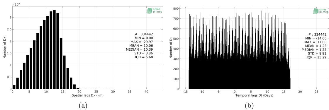
Figure 5: Histograms of the spatial (a) and temporal (b) lags between the time of the Argo measurements and the date of the corresponding SMAP SSS L3 v5.0 - Monthly (JPL) SSS product.
