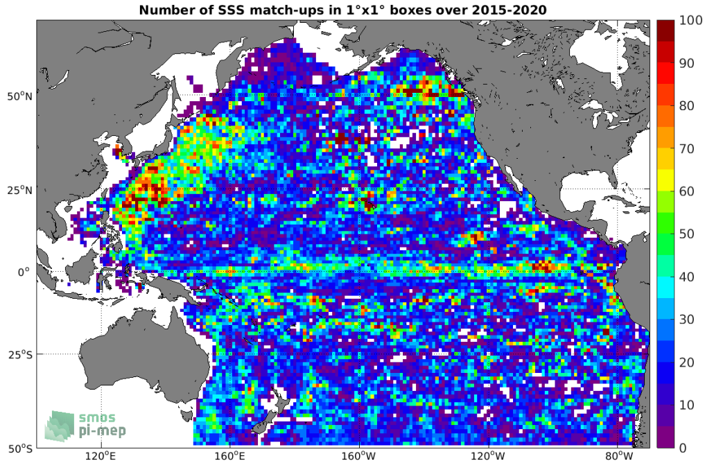
Figure 4: Number of SSS match-ups between Argo SSS and the SMAP SSS L3 v5.0 - Monthly (JPL) SSS product for the Pacific Ocean Pi-MEP region over 1°x1° boxes and for the full satellite product period.
