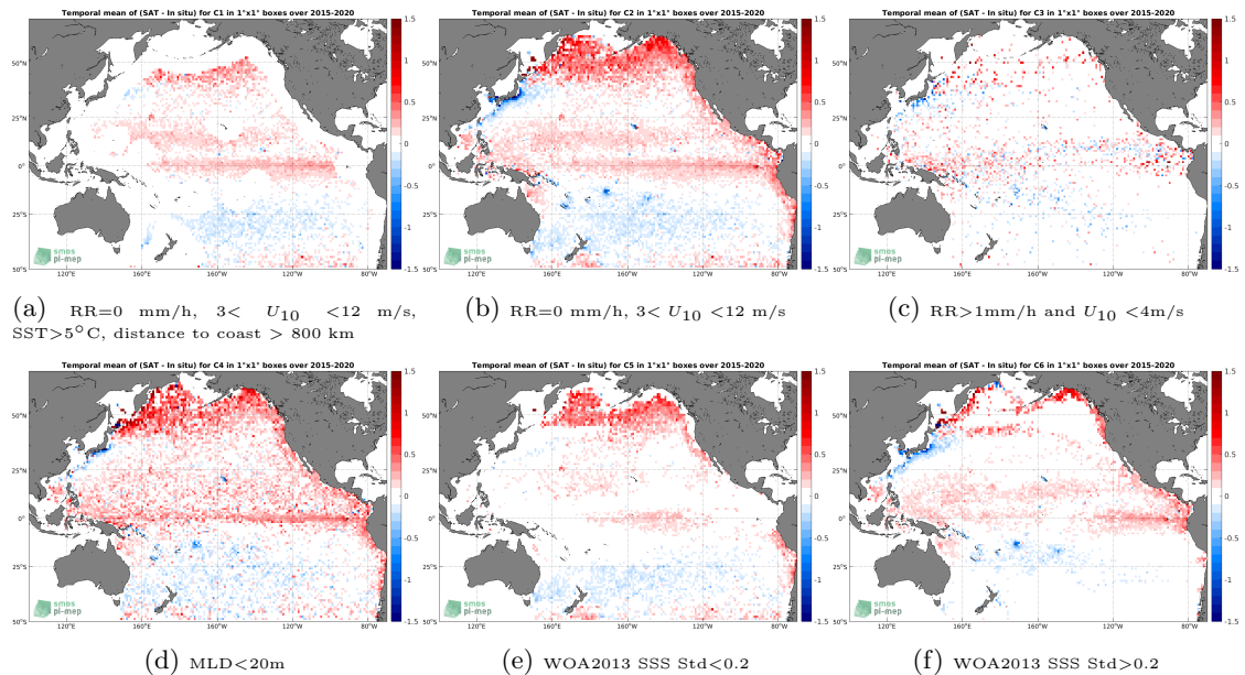
Figure 12: Temporal mean gridded over spatial boxes of size 1^\circ \times 1^\circ of \Delta SSS (SMAP SSS L3 v5.0 - Monthly (JPL) - Argo) for 6 different subdatasets corresponding to: RR=0 mm/h, 3 < U_{10} < 12 m/s, SST > 5°C, distance to coast > 800 km (a), RR=0 mm/h, 3 < U_{10} < 12 m/s (b), RR > 1mm/h and U_{10} < 4 m/s (c), MLD < 20m (d), WOA2013 SSS Std < 0.2 (e), WOA2013 SSS Std > 0.2 (f).
