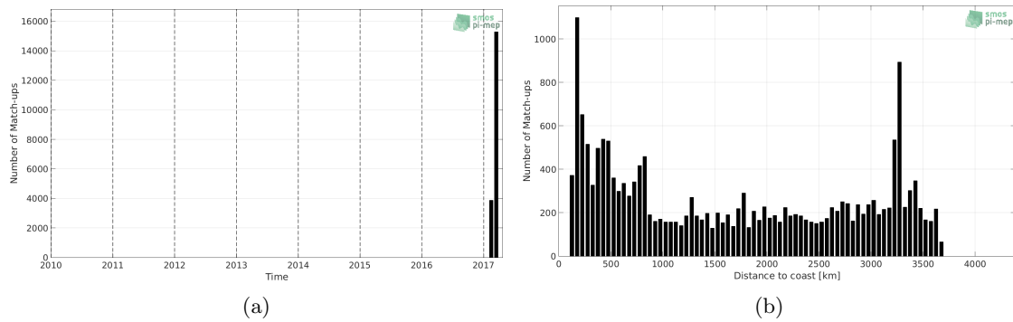
Figure 1: Number of match-ups between TSG-GOSUD-Sailing-ship and SMAP-L3-JPL-V4.2-MONTHLY-60KM SSS as a function of time (a) and as function of the distance to coast (b) over the Pacific Ocean Pi-MEP region and for the full satellite product period.
