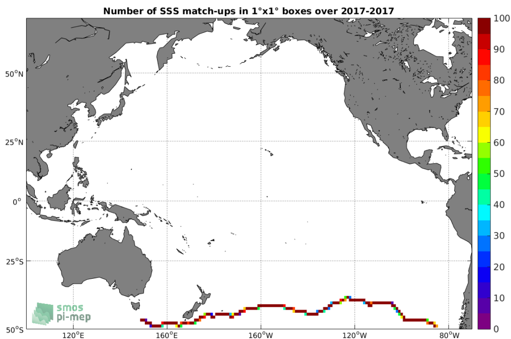
Figure 4: Number of SSS match-ups between TSG-GOSUD-Sailing-ship SSS and the SMAP-L3-JPL-V4.2-MONTHLY-60KM SSS product for the Pacific Ocean Pi-MEP region over 1^\circ \times 1^\circ boxes and for the full satellite product period.
