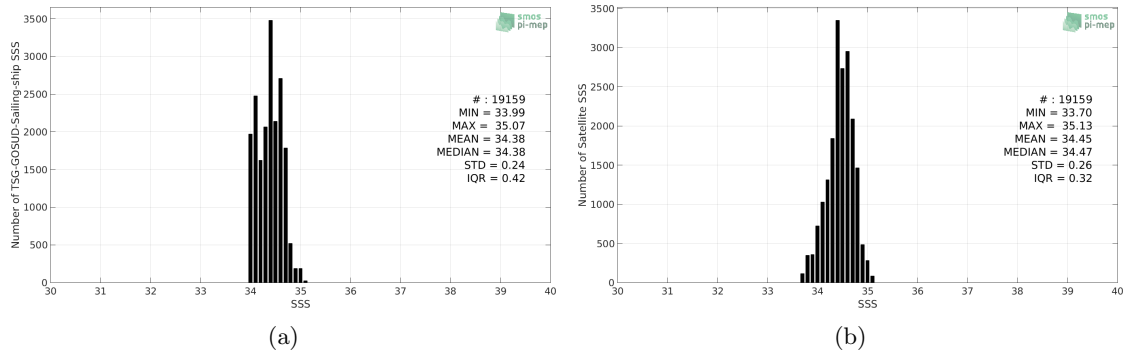
Figure 2: Histograms of SSS from TSG-GOSUD-Sailing-ship (a) and SMAP-L3-JPL-V4.2-MONTHLY-60KM (b) considering all match-up pairs per bins of 0.1 over the Pacific Ocean Pi-MEP region and for the full satellite product period.
