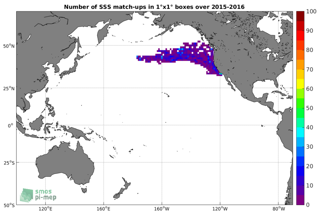
Figure 4: Number of SSS match-ups between Sea mammals SSS and the SMAP-L3-JPL-V4.2-MONTHLY-60KM SSS product for the Pacific Ocean Pi-MEP region over 1^\circ \times 1^\circ boxes and for the full satellite product period.
