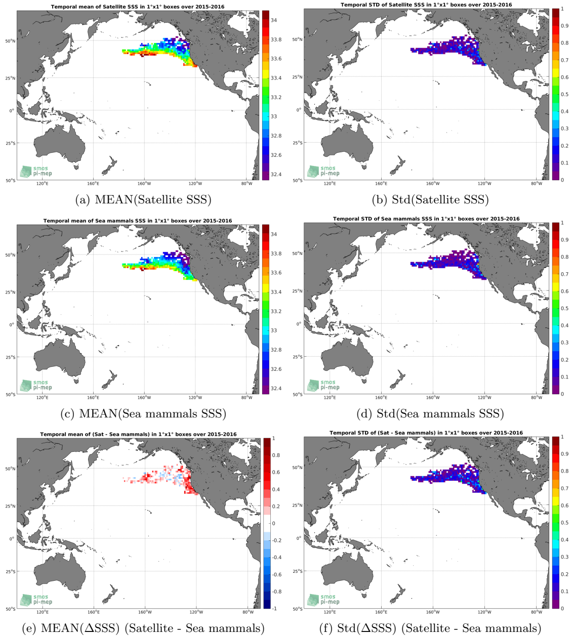
Figure 6: Temporal mean (left) and Std (right) of SSS from SMAP-L3-JPL-V4.2-MONTHLY-60KM (top), Sea mammals (middle), and of \Delta SSS (Satellite - Sea mammals). Only match-up pairs are used to generate these maps.
