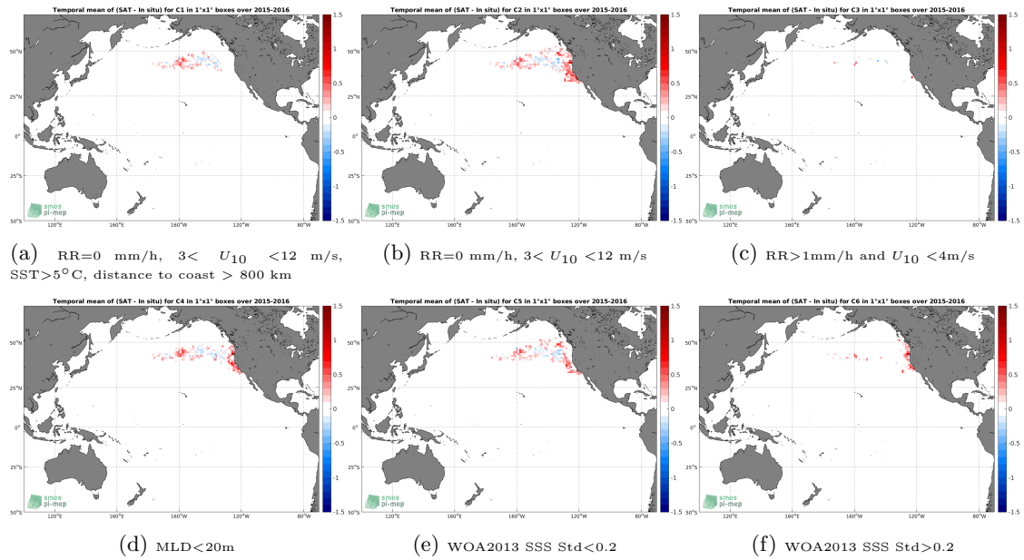
Figure 12: Temporal mean gridded over spatial boxes of size 1^\circ \times 1^\circ of \Delta SSS (SMAP-L3-JPL-V4.2-MONTHLY-60KM - Sea mammals) for 6 different subdatasets corresponding to:RR=0 mm/h, 3 < U_{10} < 12 m/s, SST >5^\circ C, distance to coast > 800 km (a), RR=0 mm/h, 3 < U_{10} < 12 m/s (b), RR >1 mm/h and U_{10} < 4 m/s (c),MLD <20 m (d),WOA2013 SSS Std <0.2 (e),WOA2013 SSS Std >0.2 (f).
