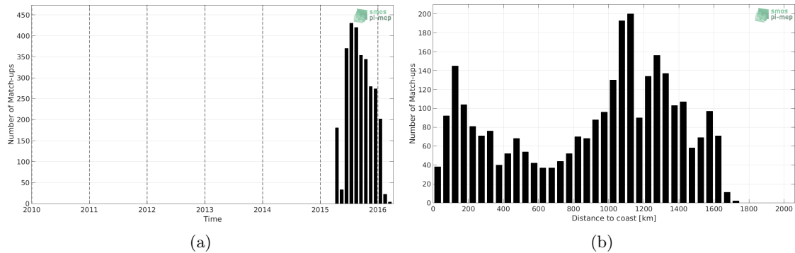
Figure 1: Number of match-ups between Sea mammals and SMAP-L3-JPL-V4.2-MONTHLY-60KM SSS as a function of time (a) and as function of the distance to coast (b) over the Pacific Ocean Pi-MEP region and for the full satellite product period.
