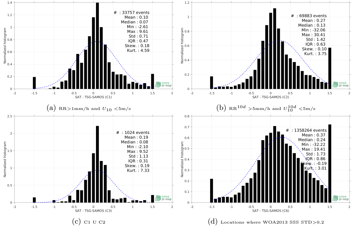
Figure 13: Normalized histogram of \Delta SSS (SMAP-L3-JPL-V4-8DAY-RUNNING-60KM - TSG-SAMOS) for 6 different subdatasets corresponding to: RR > 1mm/h and U_{10} < 5 m/s (a), RR 10d > 5mm/h and U_{10}^{10d} < 5 m/s (b), C1 U C2 (c), Locations where WOA2013 SSS STD > 0.2 (d).
