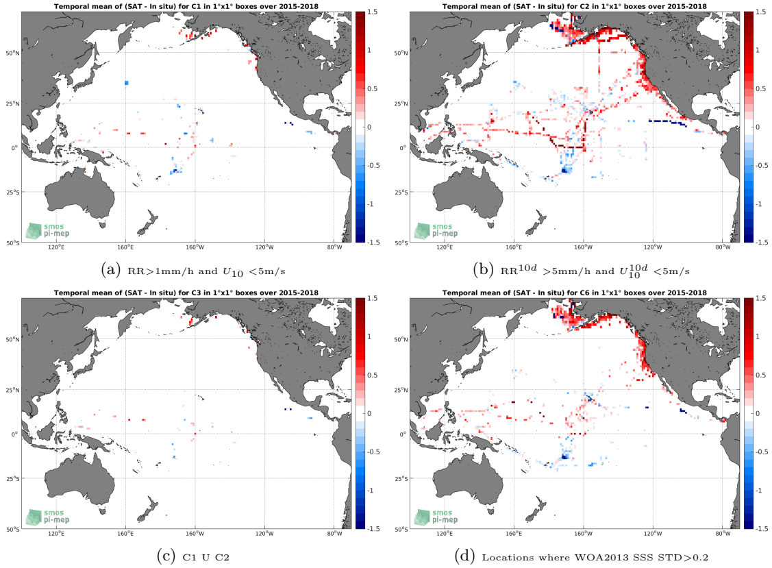
Figure 12: Temporal mean gridded over spatial boxes of size 1^\circ \times 1^\circ of \Delta SSS (SMAP-L3-JPL-V4-8DAY-RUNNING-60KM - TSG-SAMOS) for 4 different subdatasets corresponding to: RR > 1mm/h and U_{10} < 5\text{m/s} (a), RR^{10d} > 5\text{mm/h} and U_{10}^{10d} < 5\text{m/s} (b), C1 U C2 (c), Locations where WOA2013 SSS STD > 0.2 (d).
