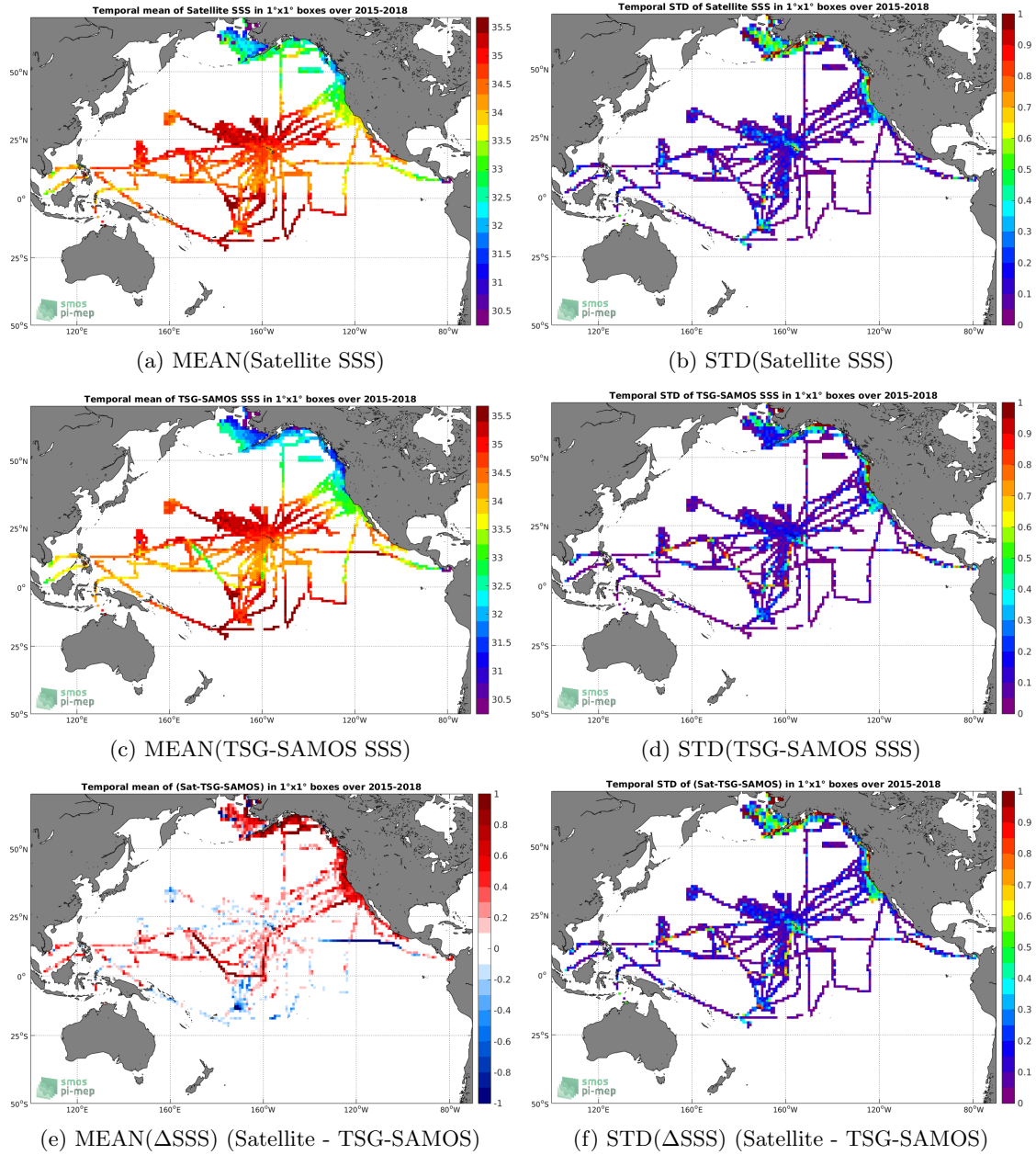
Figure 6: Temporal mean (left) and STD (right) of SSS from SMAP-L3-JPL-V4-8DAY-RUNNING-60KM (top), TSG-SAMOS (middle), and of \Delta SSS (Satellite - TSG-SAMOS). Only match-up pairs are used to generate these maps.
