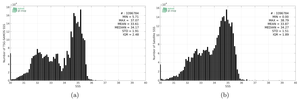
Figure 2: Histograms of SSS from TSG-SAMOS (a) and SMAP-L3-JPL-V4-8DAY-RUNNING-60KM (b) considering all match-up pairs per bins of 0.1 over the Pacific Ocean Pi-MEP region and for the full satellite product period.
