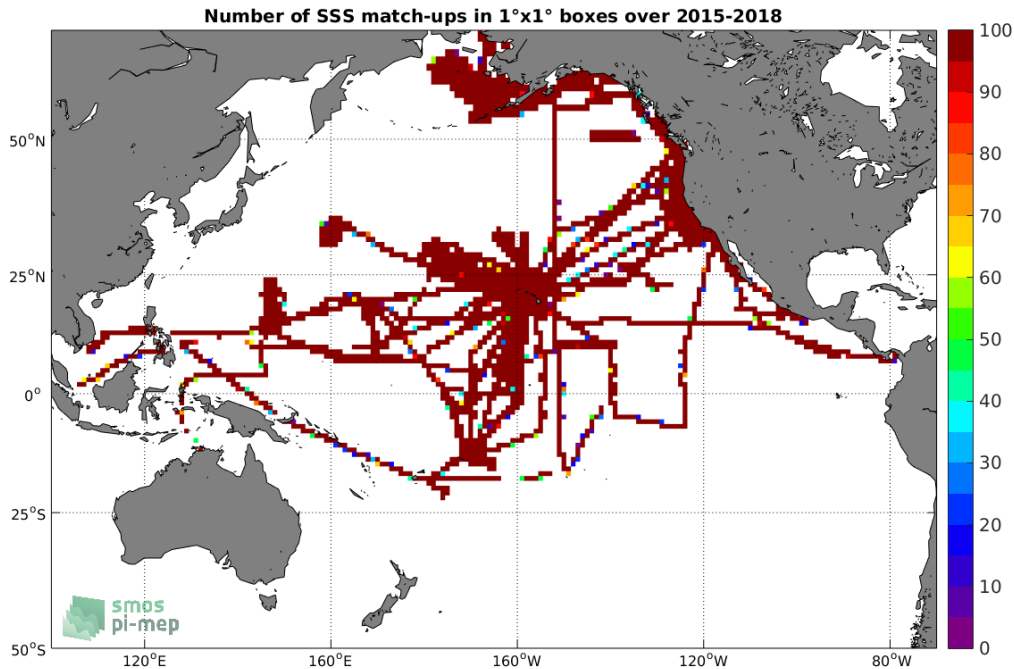
Figure 4: Number of SSS match-ups between TSG-SAMOS SSS and the SMAP-L3-JPL-V4-8DAY-RUNNING-60KM SSS product for the Pacific Ocean Pi-MEP region over 1^\circ \times 1^\circ boxes and for the full satellite product period.
