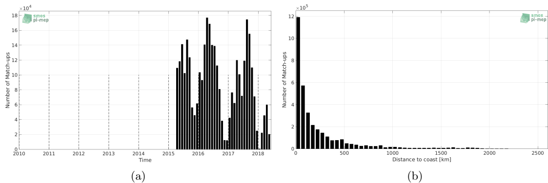
Figure 1: Number of match-ups between TSG-SAMOS and SMAP-L3-JPL-V4-8DAY-RUNNING-60KM SSS as a function of time (a) and as function of the distance to coast (b) over the Pacific Ocean Pi-MEP region and for the full satellite product period.
