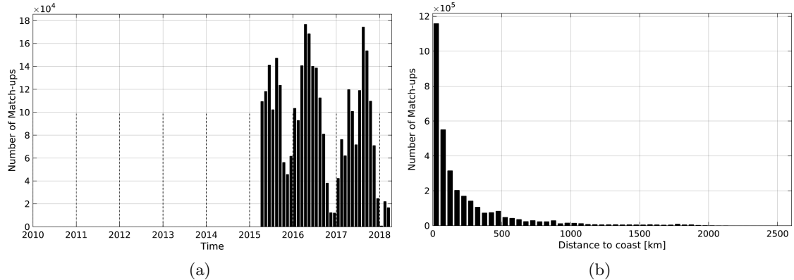
Figure 1: Number of match-ups between TSG-SAMOS and SMAP-L3-JPL-V4-8DAY-RUNNING-60KM SSS as a function of time (a) and as function of the distance to coast (b) over the Pacific Ocean Pi-MEP region and for the full satellite product period.
