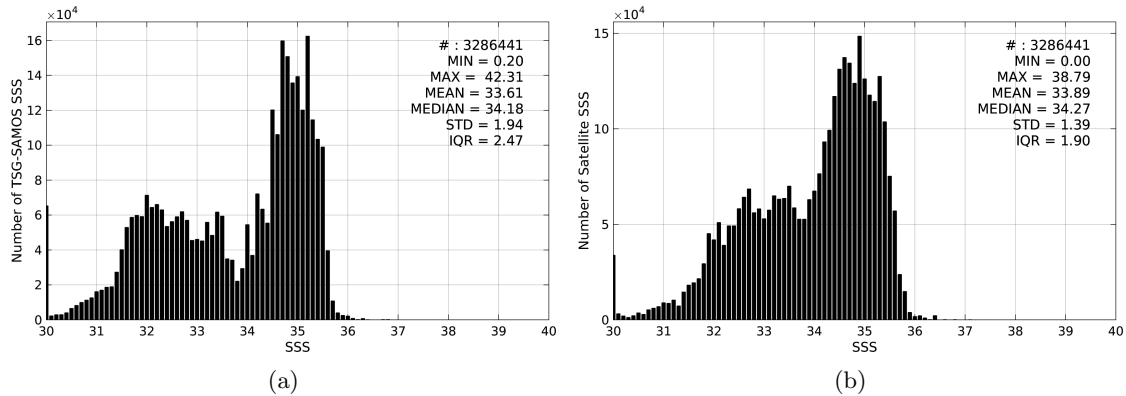
Figure 2: Histograms of SSS from TSG-SAMOS (a) and SMAP-L3-JPL-V4-8DAY-RUNNING-60KM (b) considering all match-up pairs per bins of 0.1 over the Pacific Ocean Pi-MEP region and for the full satellite product period.
