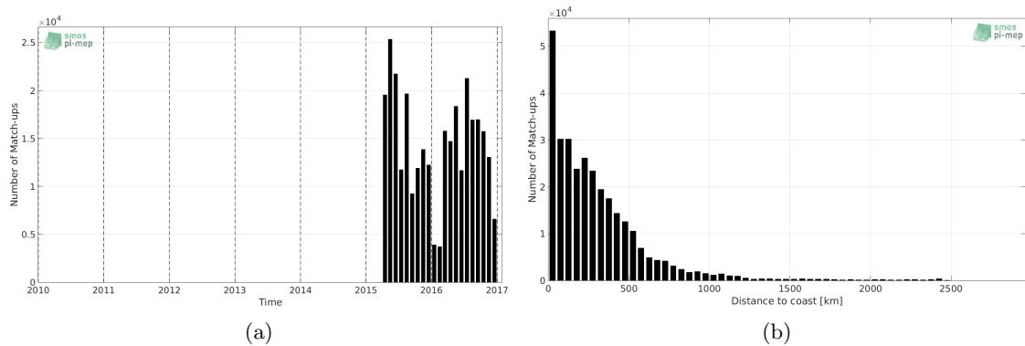
Figure 1: Number of match-ups between TSG-LEGOS-DM and SMAP-L3-JPL-V4-8DAY-RUNNING-60KM SSS as a function of time (a) and as function of the distance to coast (b) over the Pacific Ocean Pi-MEP region and for the full satellite product period.
