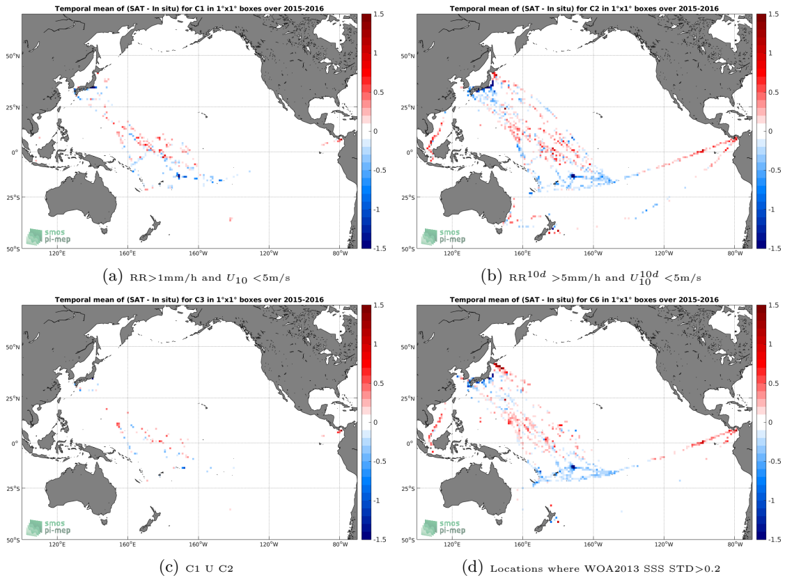
Figure 12: Temporal mean gridded over spatial boxes of size 1^\circ \times 1^\circ of \Delta SSS (SMAP-L3-JPL-V4-8DAY-RUNNING-60KM - TSG-LEGOS-DM) for 4 different subdatasets corresponding to: RR > 1\text{mm/h} and U_{10} < 5\text{m/s} (a), RR^{10d} > 5\text{mm/h} and U_{10}^{10d} < 5\text{m/s} (b), C1 U C2 (c), Locations where WOA2013 SSS STD > 0.2 (d).
