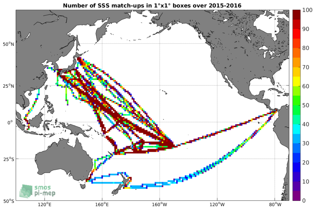
Figure 4: Number of SSS match-ups between TSG-LEGOS-DM SSS and the SMAP-L3-JPL-V4-8DAY-RUNNING-60KM SSS product for the Pacific Ocean Pi-MEP region over 1^\circ \times 1^\circ boxes and for the full satellite product period.
