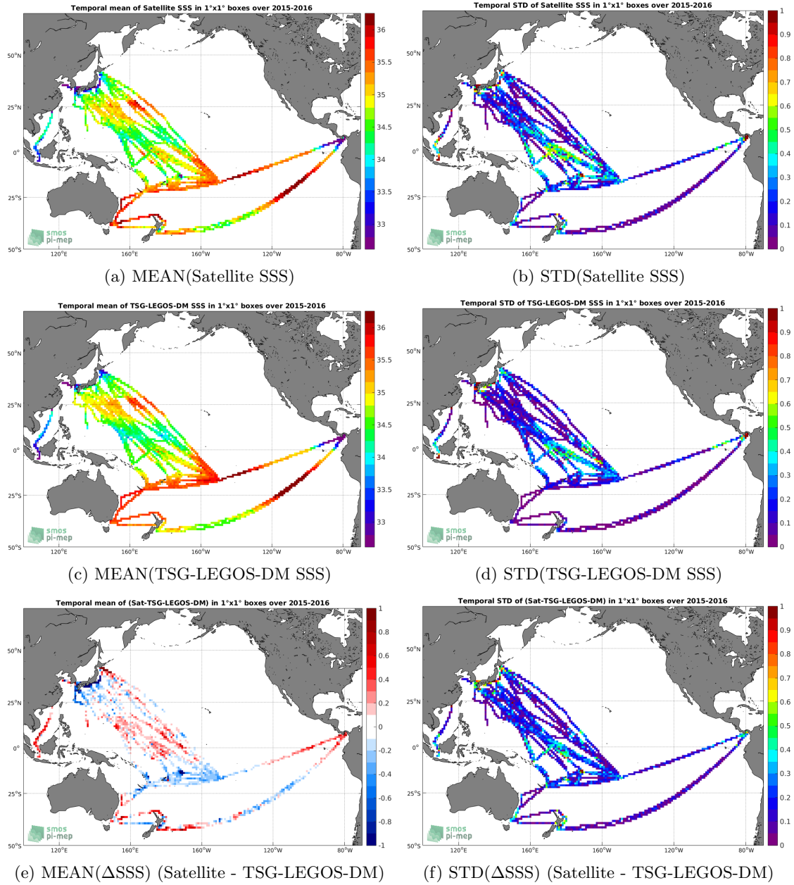
Figure 6: Temporal mean (left) and STD (right) of SSS from SMAP-L3-JPL-V4-8DAY-RUNNING-60KM (top), TSG-LEGOS-DM (middle), and of \Delta SSS (Satellite - TSG-LEGOS-DM). Only match-up pairs are used to generate these maps.
