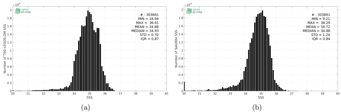
Figure 2: Histograms of SSS from TSG-LEGOS-DM (a) and SMAP-L3-JPL-V4-8DAY-RUNNING-60KM (b) considering all match-up pairs per bins of 0.1 over the Pacific Ocean Pi-MEP region and for the full satellite product period.
