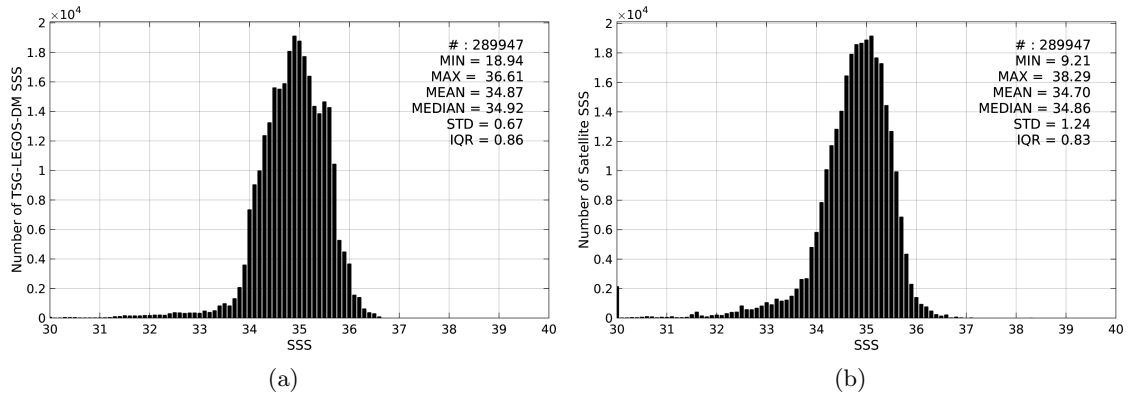
Figure 2: Histograms of SSS from TSG-LEGOS-DM (a) and SMAP-L3-JPL-V4-8DAY-RUNNING-60KM (b) considering all match-up pairs per bins of 0.1 over the Pacific Ocean Pi-MEP region and for the full satellite product period.
