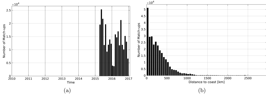
Figure 1: Number of match-ups between TSG-LEGOS-DM and SMAP-L3-JPL-V4-8DAY-RUNNING-60KM SSS as a function of time (a) and as function of the distance to coast (b) over the Pacific Ocean Pi-MEP region and for the full satellite product period.
