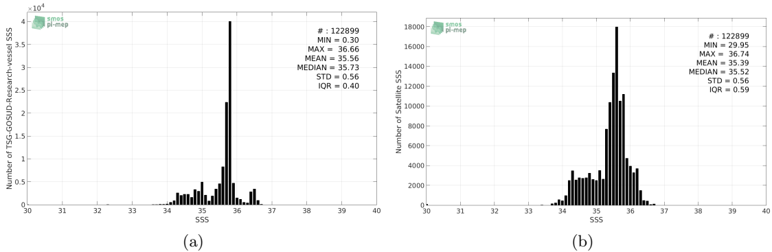
Figure 2: Histograms of SSS from TSG-GOSUD-Research-vessel (a) and SMAP-L3-JPL-V4-8DAY-RUNNING-60KM (b) considering all match-up pairs per bins of 0.1 over the Pacific Ocean Pi-MEP region and for the full satellite product period.
