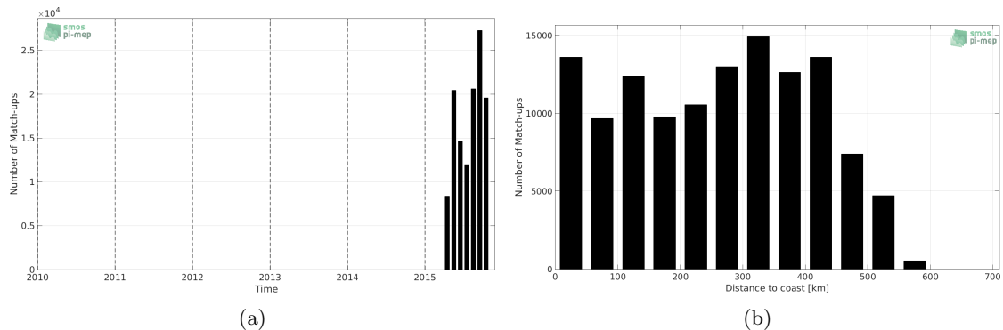
Figure 1: Number of match-ups between TSG-GOSUD-Research-vessel and SMAP-L3-JPL-V4-8DAY-RUNNING-60KM SSS as a function of time (a) and as function of the distance to coast (b) over the Pacific Ocean Pi-MEP region and for the full satellite product period.
