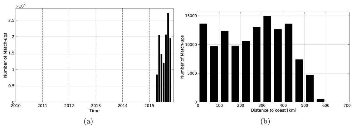
Figure 1: Number of match-ups between TSG-GOSUD-Research-vessel and SMAP-L3-JPL-V4-8DAY-RUNNING-60KM SSS as a function of time (a) and as function of the distance to coast (b) over the Pacific Ocean Pi-MEP region and for the full satellite product period.
