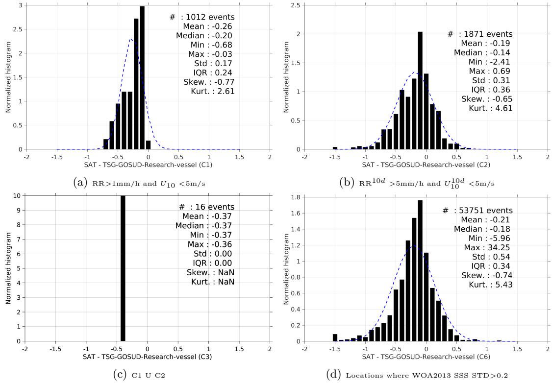
Figure 13: Normalized histogram of \Delta\text{SSS} (SMAP-L3-JPL-V4-8DAY-RUNNING-60KM - TSG-GOSUD-Research-vessel) for 6 different subdatasets corresponding to: \text{RR} > 1\text{mm/h} and U_{10} < 5\text{m/s} (a), \text{RR}^{10d} > 5\text{mm/h} and U_{10}^{10d} < 5\text{m/s} (b), C1 U C2 (c), Locations where WOA2013 SSS STD > 0.2 (d).
