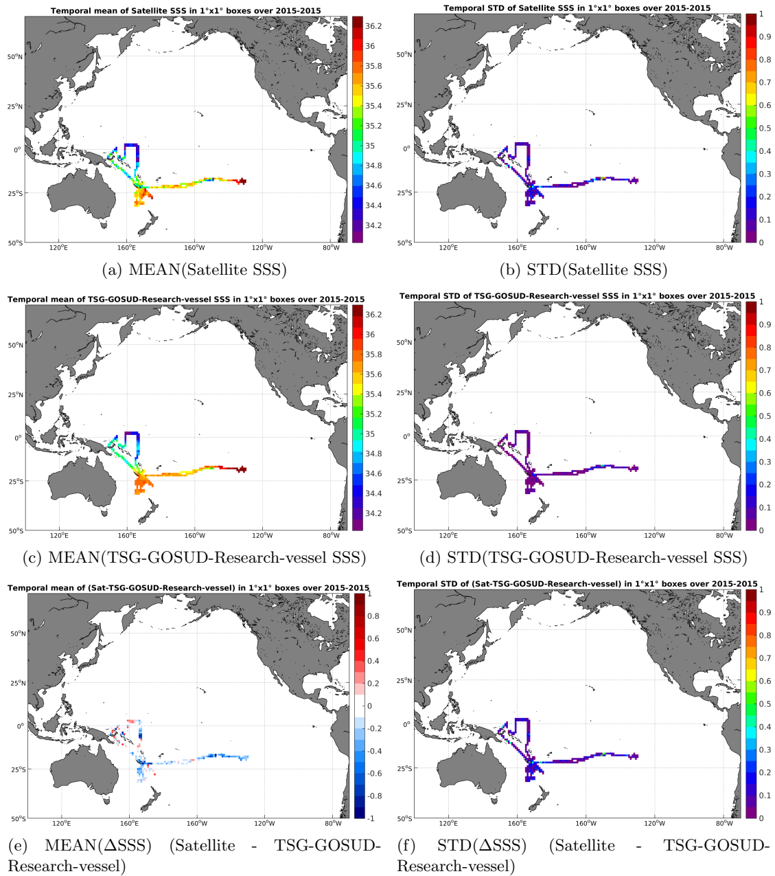
Figure 6: Temporal mean (left) and STD (right) of SSS from SMAP-L3-JPL-V4-8DAY-RUNNING-60KM (top), TSG-GOSUD-Research-vessel (middle), and of \Delta SSS (Satellite - TSG-GOSUD-Research-vessel). Only match-up pairs are used to generate these maps.
