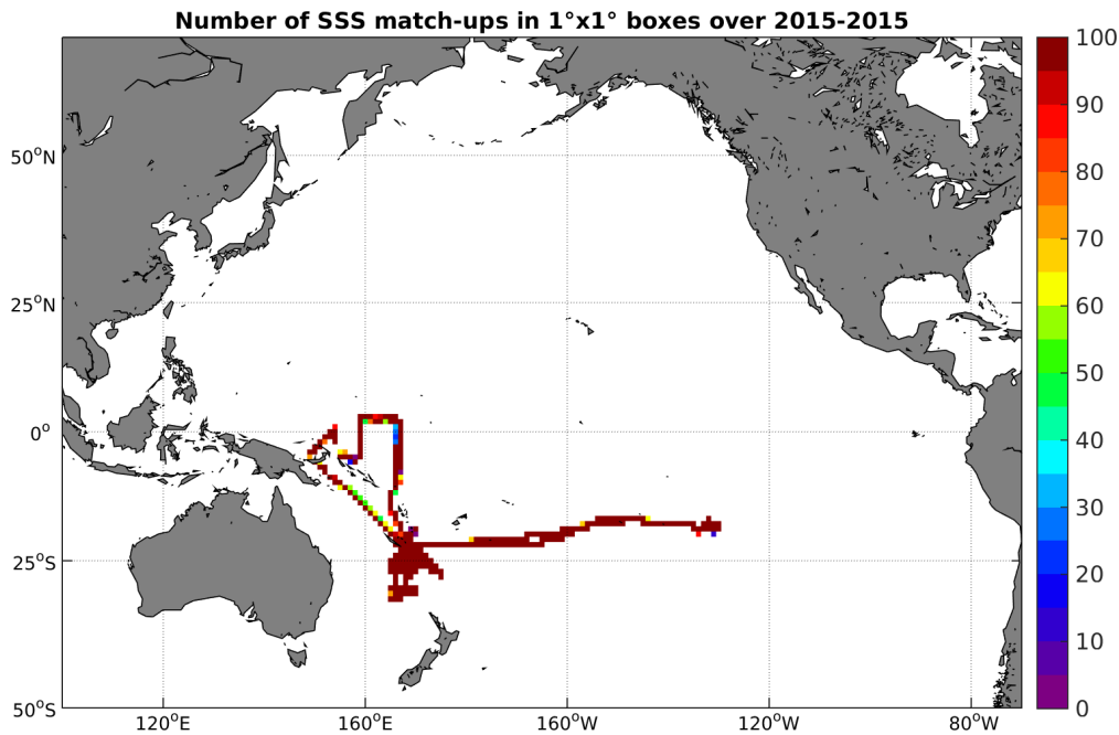
Figure 4: Number of SSS match-ups between TSG-GOSUD-Research-vessel SSS and the SMAP-L3-JPL-V4-8DAY-RUNNING-60KM SSS product for the Pacific Ocean Pi-MEP region over 1^\circ \times 1^\circ boxes and for the full satellite product period.
