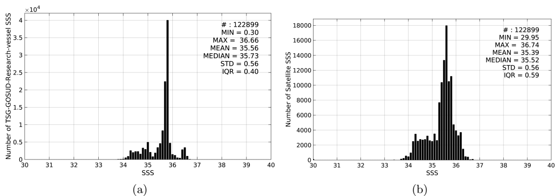
Figure 2: Histograms of SSS from TSG-GOSUD-Research-vessel (a) and SMAP-L3-JPL-V4-8DAY-RUNNING-60KM (b) considering all match-up pairs per bins of 0.1 over the Pacific Ocean Pi-MEP region and for the full satellite product period.
