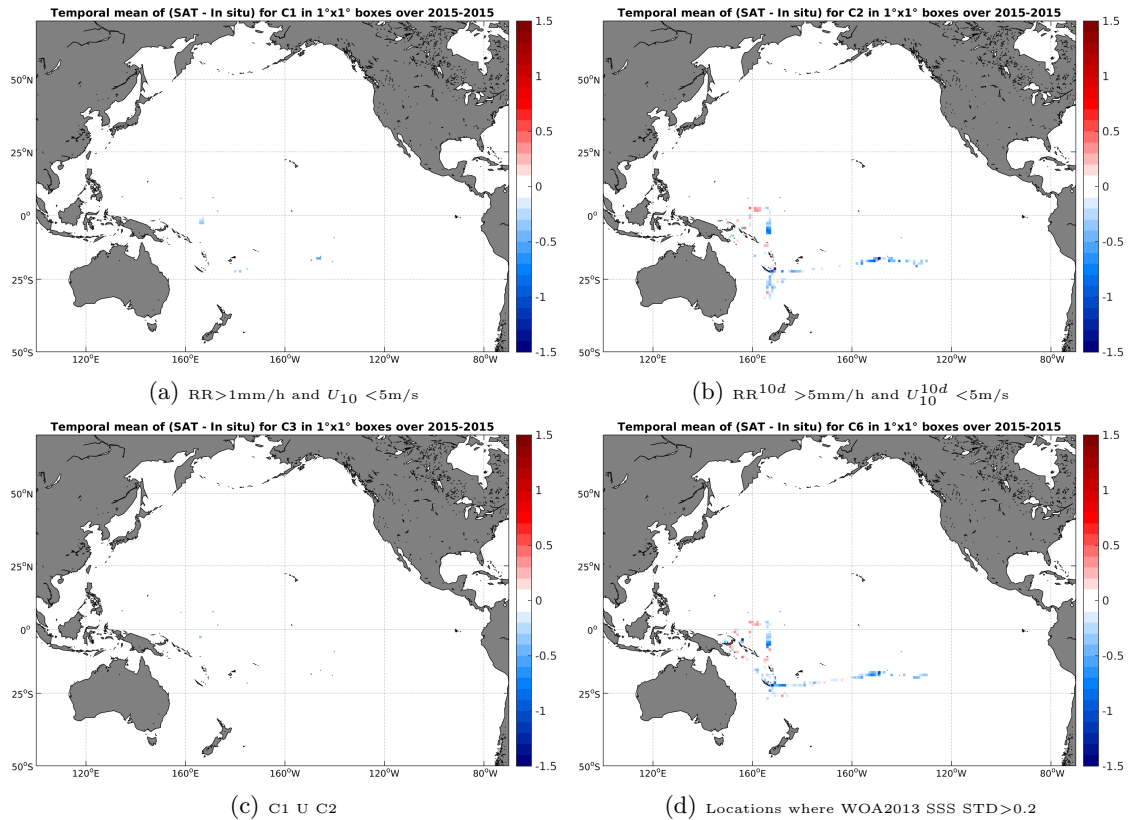
Figure 12: Temporal mean gridded over spatial boxes of size 1^\circ \times 1^\circ of \Delta SSS (SMAP-L3-JPL-V4-8DAY-RUNNING-60KM - TSG-GOSUD-Research-vessel) for 4 different subdatasets corresponding to: RR > 1\text{mm/h} and U_{10} < 5\text{m/s} (a), RR^{10d} > 5\text{mm/h} and U_{10}^{10d} < 5\text{m/s} (b), C1 U C2 (c), Locations where WOA2013 SSS STD > 0.2 (d).
