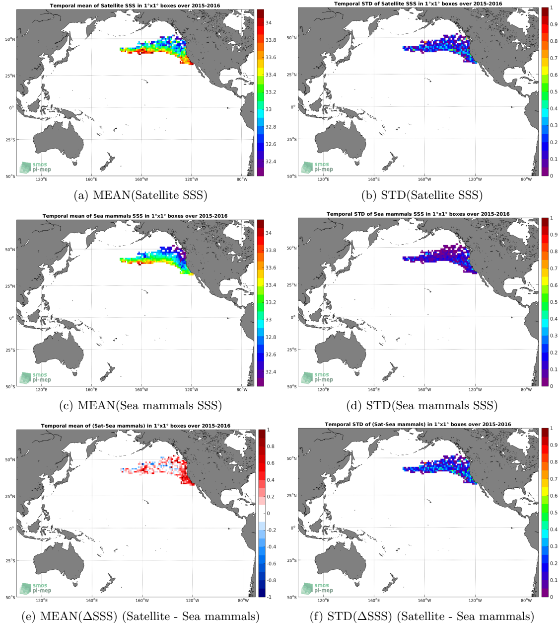
Figure 6: Temporal mean (left) and STD (right) of SSS from SMAP-L3-JPL-V4-8DAY-RUNNING-60KM (top), Sea mammals (middle), and of \Delta SSS (Satellite - Sea mammals). Only match-up pairs are used to generate these maps.
