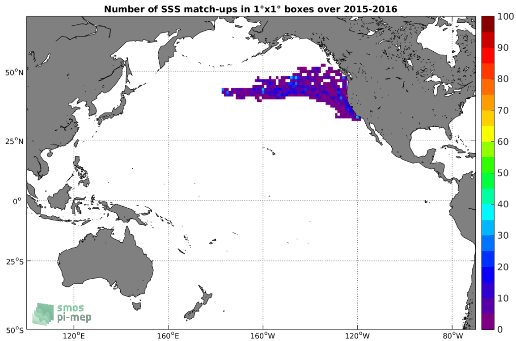
Figure 4: Number of SSS match-ups between Sea mammals SSS and the SMAP-L3-JPL-V4-8DAY-RUNNING-60KM SSS product for the Pacific Ocean Pi-MEP region over 1^\circ \times 1^\circ boxes and for the full satellite product period.
