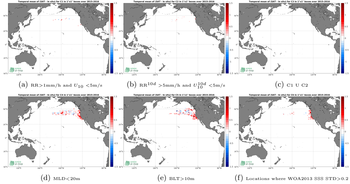
Figure 12: Temporal mean gridded over spatial boxes of size 1^\circ \times 1^\circ of \Delta\text{SSS} (SMAP-L3-JPL-V4-8DAY-RUNNING-60KM - Sea mammals) for 6 different subdatasets corresponding to: \text{RR} > 1\text{mm/h} and U_{10} < 5\text{m/s} (a), \text{RR}^{10d} > 5\text{mm/h} and U_{10}^{10d} < 5\text{m/s} (b), \text{C1} \cup \text{C2} (c), \text{MLD} < 20\text{m} (d), \text{BLT} > 10\text{m} (e), Locations where WOA2013 SSS STD > 0.2 (f).
