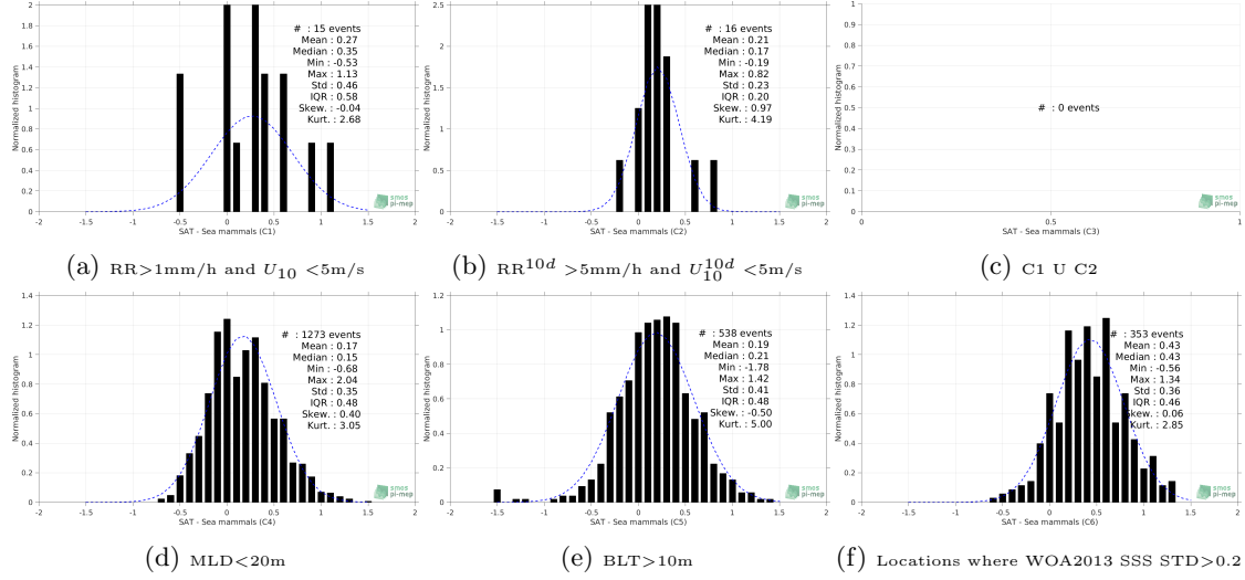
Figure 13: Normalized histogram of \Delta SSS (SMAP-L3-JPL-V4-8DAY-RUNNING-60KM - Sea mammals) for 6 different subdatasets corresponding to: RR > 1\text{mm/h} and U_{10} < 5\text{m/s} (a), RR^{10d} > 5\text{mm/h} and U_{10}^{10d} < 5\text{m/s} (b), C1 \cup C2 (c), MLD < 20\text{m} (d), BLT > 10\text{m} (e), Locations where WOA2013 SSS STD > 0.2 (f).
