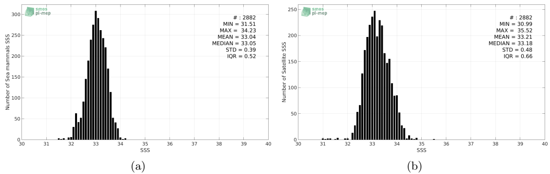
Figure 2: Histograms of SSS from Sea mammals (a) and SMAP-L3-JPL-V4-8DAY-RUNNING-60KM (b) considering all match-up pairs per bins of 0.1 over the Pacific Ocean Pi-MEP region and for the full satellite product period.
