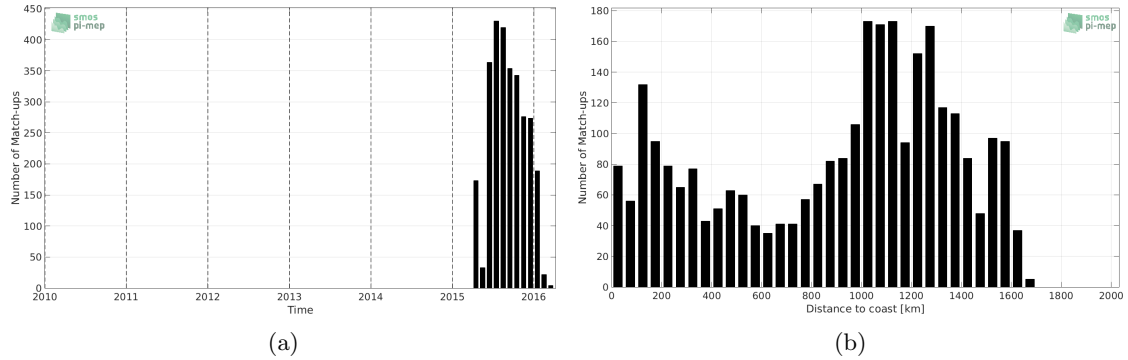
Figure 1: Number of match-ups between Sea mammals and SMAP-L3-JPL-V4-8DAY-RUNNING-60KM SSS as a function of time (a) and as function of the distance to coast (b) over the Pacific Ocean Pi-MEP region and for the full satellite product period.
