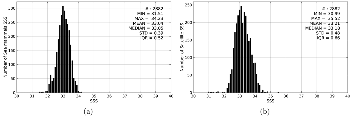
Figure 2: Histograms of SSS from Sea mammals (a) and SMAP-L3-JPL-V4-8DAY-RUNNING-60KM (b) considering all match-up pairs per bins of 0.1 over the Pacific Ocean Pi-MEP region and for the full satellite product period.
