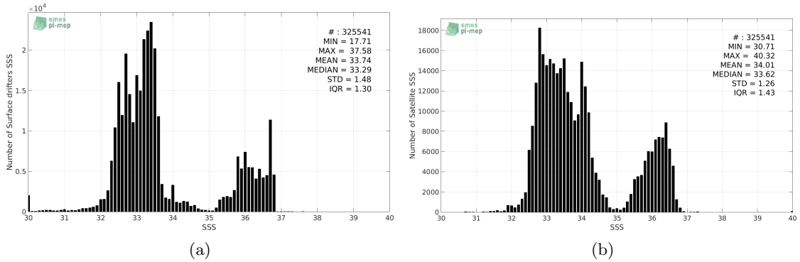
Figure 2: Histograms of SSS from Surface drifters (a) and SMAP-L3-JPL-V4-8DAY-RUNNING-60KM (b) considering all match-up pairs per bins of 0.1 over the Pacific Ocean Pi-MEP region and for the full satellite product period.
