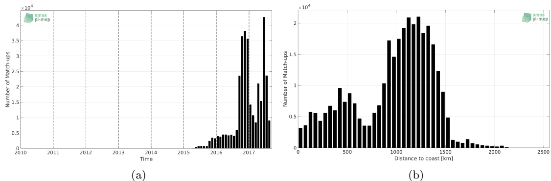
Figure 1: Number of match-ups between Surface drifters and SMAP-L3-JPL-V4-8DAY-RUNNING-60KM SSS as a function of time (a) and as function of the distance to coast (b) over the Pacific Ocean Pi-MEP region and for the full satellite product period.
