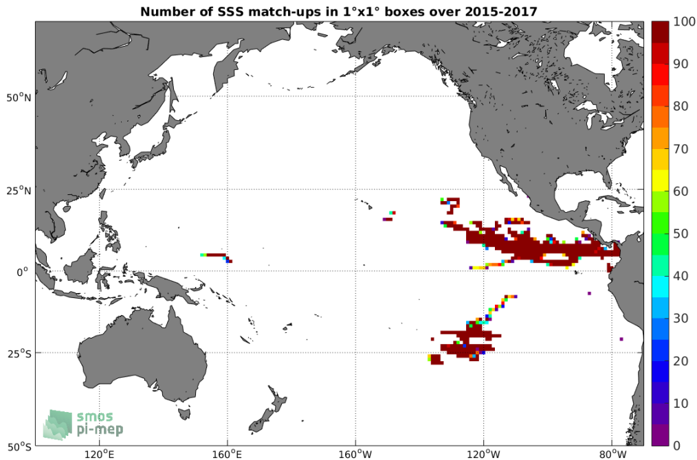
Figure 3: Number of SSS match-ups between Surface drifters SSS and the SMAP-L3-JPL-V4-8DAY-RUNNING-60KM SSS product for the Pacific Ocean Pi-MEP region over 1^{\circ} \times 1^{\circ} boxes and for the full satellite product period.
