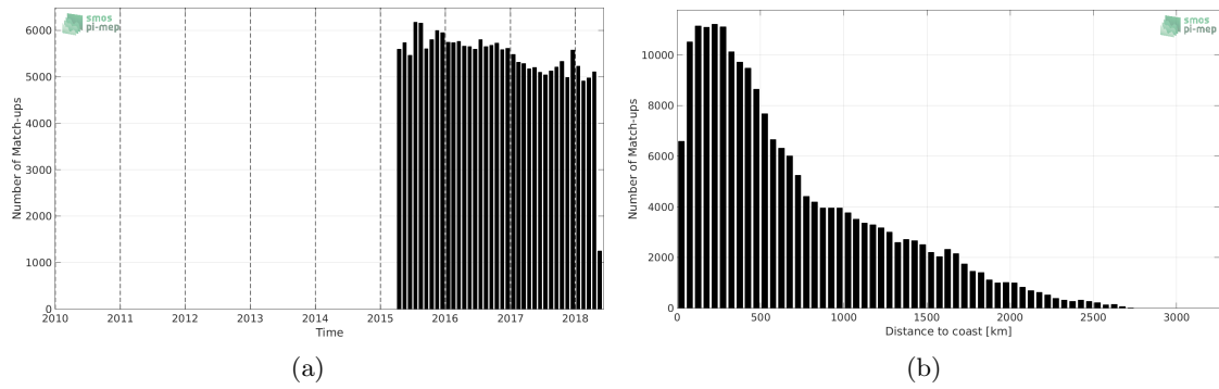
Figure 1: Number of match-ups between Argo and SMAP-L3-JPL-V4-8DAY-RUNNING-60KM SSS as a function of time (a) and as function of the distance to coast (b) over the Pacific Ocean Pi-MEP region and for the full satellite product period.
