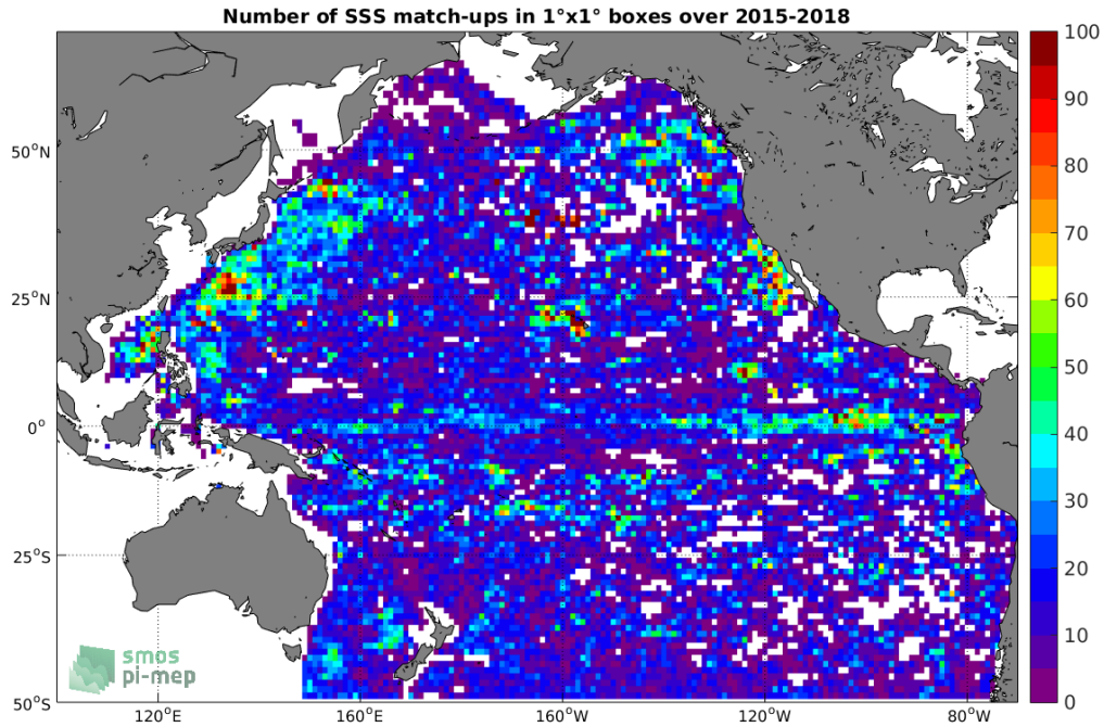
Figure 4: Number of SSS match-ups between Argo SSS and the SMAP-L3-JPL-V4-8DAY-RUNNING-60KM SSS product for the Pacific Ocean Pi-MEP region over 1°x1° boxes and for the full satellite product period.
