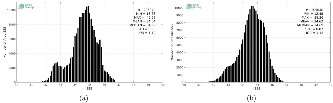
Figure 2: Histograms of SSS from Argo (a) and SMAP-L3-JPL-V4-8DAY-RUNNING-60KM (b) considering all match-up pairs per bins of 0.1 over the Pacific Ocean Pi-MEP region and for the full satellite product period.
