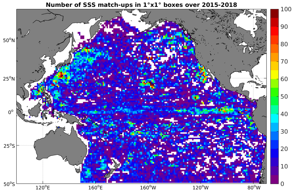
Figure 4: Number of SSS match-ups between Argo SSS and the SMAP-L3-JPL-V4-8DAY-RUNNING-60KM SSS product for the Pacific Ocean Pi-MEP region over 1^\circ \times 1^\circ boxes and for the full satellite product period.
