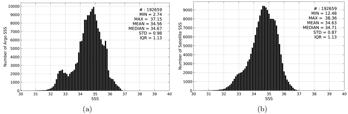
Figure 2: Histograms of SSS from Argo (a) and SMAP-L3-JPL-V4-8DAY-RUNNING-60KM (b) considering all match-up pairs per bins of 0.1 over the Pacific Ocean Pi-MEP region and for the full satellite product period.
