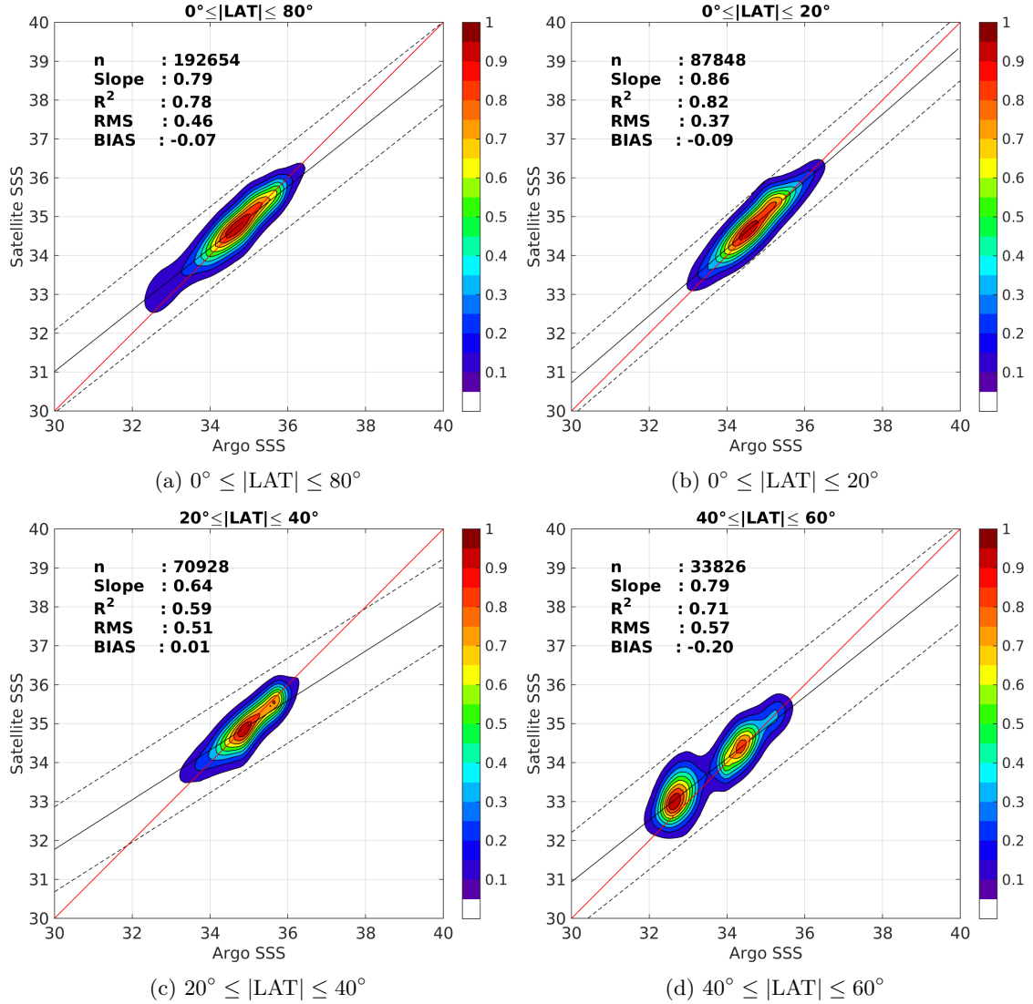
Figure 9: Contour maps of the concentration of SMAP-L3-JPL-V4-8DAY-RUNNING-60KM SSS (y-axis) versus Argo SSS (x-axis) at match-up pairs for different latitude bands. For each plot, the red line shows x=y . The black thin and dashed lines indicate a linear fit through the data cloud and the \pm 95\% confidence levels, respectively. The number match-up pairs n , the slope and R^2 coefficient of the linear fit, the root mean square (RMS) and the mean bias between satellite and in situ data are indicated for each latitude band in each plots.
