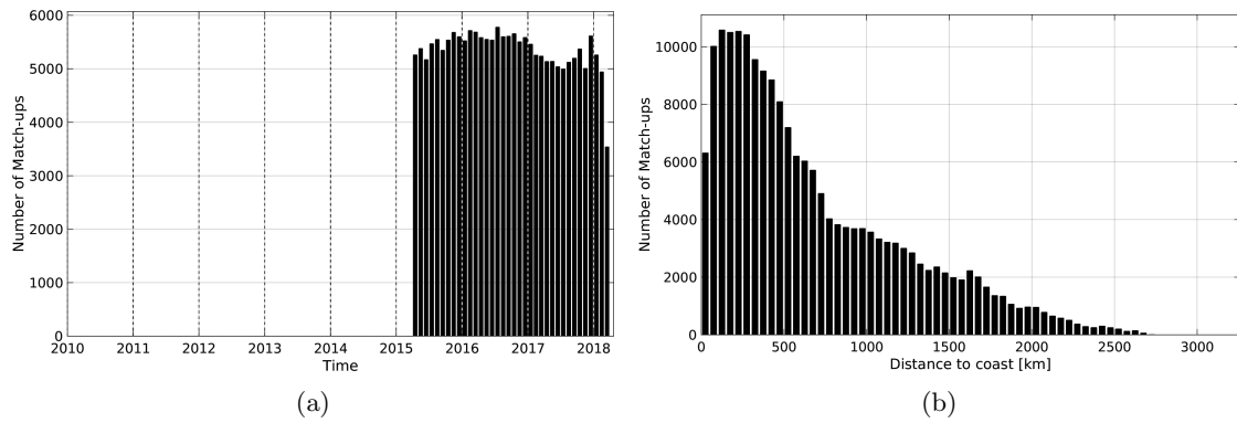
Figure 1: Number of match-ups between Argo and SMAP-L3-JPL-V4-8DAY-RUNNING-60KM SSS as a function of time (a) and as function of the distance to coast (b) over the Pacific Ocean Pi-MEP region and for the full satellite product period.
