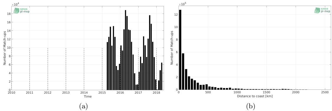
Figure 1: Number of match-ups between TSG-SAMOS and SMAP-L3-JPL-V4-MONTHLY-60KM SSS as a function of time (a) and as function of the distance to coast (b) over the Pacific Ocean Pi-MEP region and for the full satellite product period.
