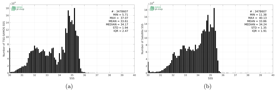
Figure 2: Histograms of SSS from TSG-SAMOS (a) and SMAP-L3-JPL-V4-MONTHLY-60KM (b) considering all match-up pairs per bins of 0.1 over the Pacific Ocean Pi-MEP region and for the full satellite product period.
