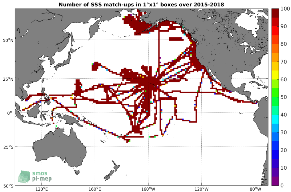
Figure 4: Number of SSS match-ups between TSG-SAMOS SSS and the SMAP-L3-JPL-V4-MONTHLY-60KM SSS product for the Pacific Ocean Pi-MEP region over 1^\circ \times 1^\circ boxes and for the full satellite product period.
