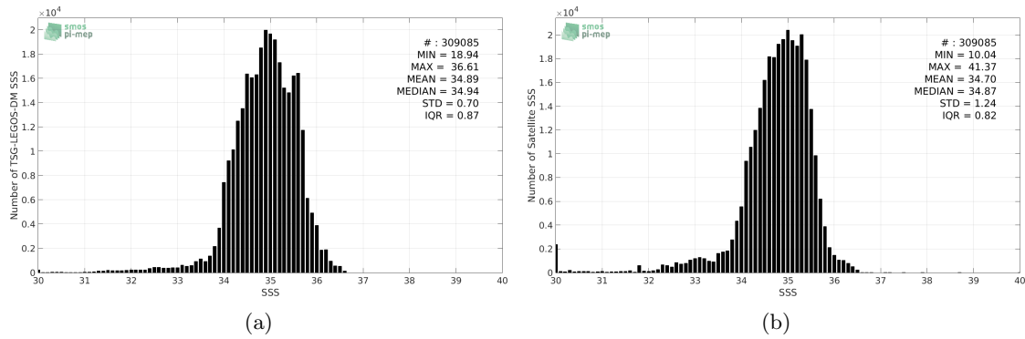
Figure 2: Histograms of SSS from TSG-LEGOS-DM (a) and SMAP-L3-JPL-V4-MONTHLY-60KM (b) considering all match-up pairs per bins of 0.1 over the Pacific Ocean Pi-MEP region and for the full satellite product period.
