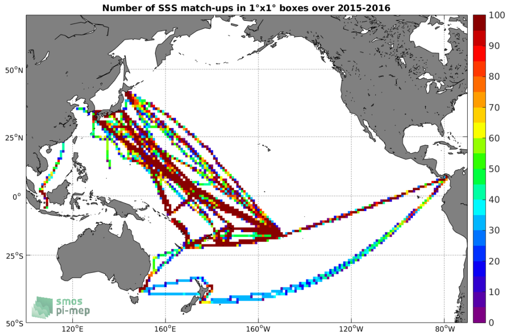
Figure 4: Number of SSS match-ups between TSG-LEGOS-DM SSS and the SMAP-L3-JPL-V4-MONTHLY-60KM SSS product for the Pacific Ocean Pi-MEP region over 1^\circ \times 1^\circ boxes and for the full satellite product period.
