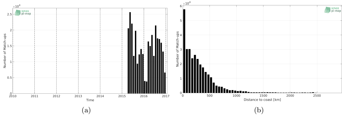
Figure 1: Number of match-ups between TSG-LEGOS-DM and SMAP-L3-JPL-V4-MONTHLY-60KM SSS as a function of time (a) and as function of the distance to coast (b) over the Pacific Ocean Pi-MEP region and for the full satellite product period.
