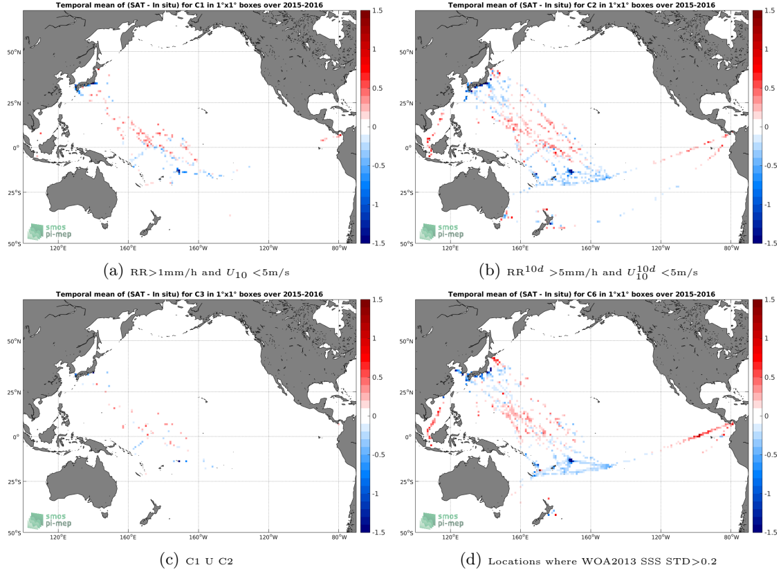
Figure 12: Temporal mean gridded over spatial boxes of size 1^\circ \times 1^\circ of \Delta SSS (SMAP-L3-JPL-V4-MONTHLY-60KM - TSG-LEGOS-DM) for 4 different subdatasets corresponding to: RR > 1\text{mm/h} and U_{10} < 5\text{m/s} (a), RR^{10d} > 5\text{mm/h} and U_{10}^{10d} < 5\text{m/s} (b), C1 U C2 (c), Locations where WOA2013 SSS STD > 0.2 (d).
