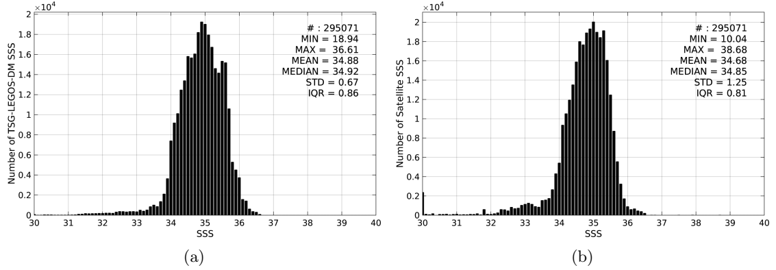
Figure 2: Histograms of SSS from TSG-LEGOS-DM (a) and SMAP-L3-JPL-V4-MONTHLY-60KM (b) considering all match-up pairs per bins of 0.1 over the Pacific Ocean Pi-MEP region and for the full satellite product period.
