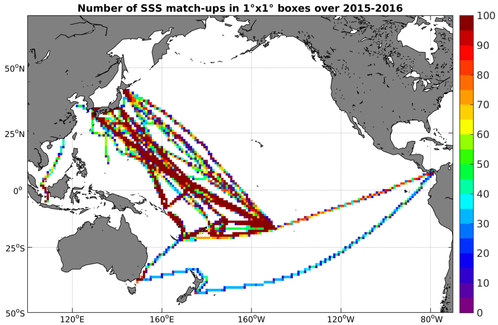
Figure 4: Number of SSS match-ups between TSG-LEGOS-DM SSS and the SMAP-L3-JPL-V4-MONTHLY-60KM SSS product for the Pacific Ocean Pi-MEP region over 1^\circ \times 1^\circ boxes and for the full satellite product period.
