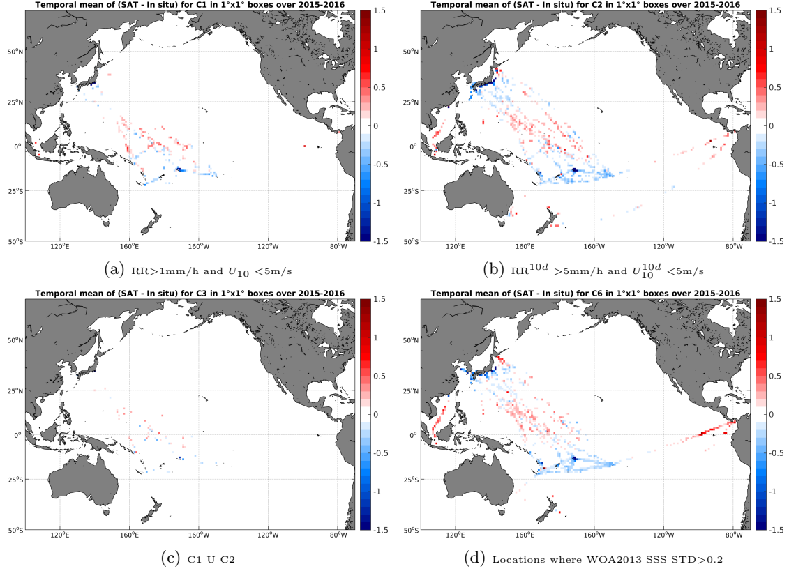
Figure 12: Temporal mean gridded over spatial boxes of size 1^\circ \times 1^\circ of \Delta SSS (SMAP-L3-JPL-V4-MONTHLY-60KM - TSG-LEGOS-DM) for 4 different subdatasets corresponding to: RR > 1mm/h and U_{10} < 5 m/s (a), RR^{10d} > 5 mm/h and U_{10}^{10d} < 5 m/s (b), C1 U C2 (c), Locations where WOA2013 SSS STD > 0.2 (d).
