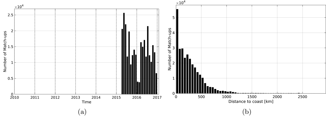
Figure 1: Number of match-ups between TSG-LEGOS-DM and SMAP-L3-JPL-V4-MONTHLY-60KM SSS as a function of time (a) and as function of the distance to coast (b) over the Pacific Ocean Pi-MEP region and for the full satellite product period.
