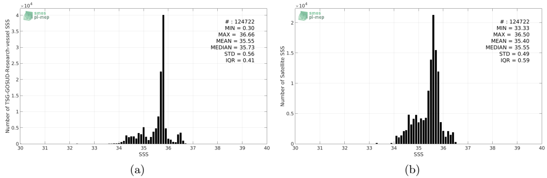
Figure 2: Histograms of SSS from TSG-GOSUD-Research-vessel (a) and SMAP-L3-JPL-V4-MONTHLY-60KM (b) considering all match-up pairs per bins of 0.1 over the Pacific Ocean Pi-MEP region and for the full satellite product period.
