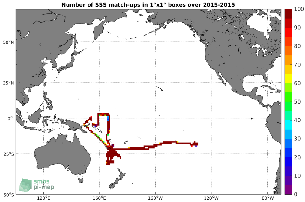
Figure 4: Number of SSS match-ups between TSG-GOSUD-Research-vessel SSS and the SMAP-L3-JPL-V4-MONTHLY-60KM SSS product for the Pacific Ocean Pi-MEP region over 1^\circ \times 1^\circ boxes and for the full satellite product period.
