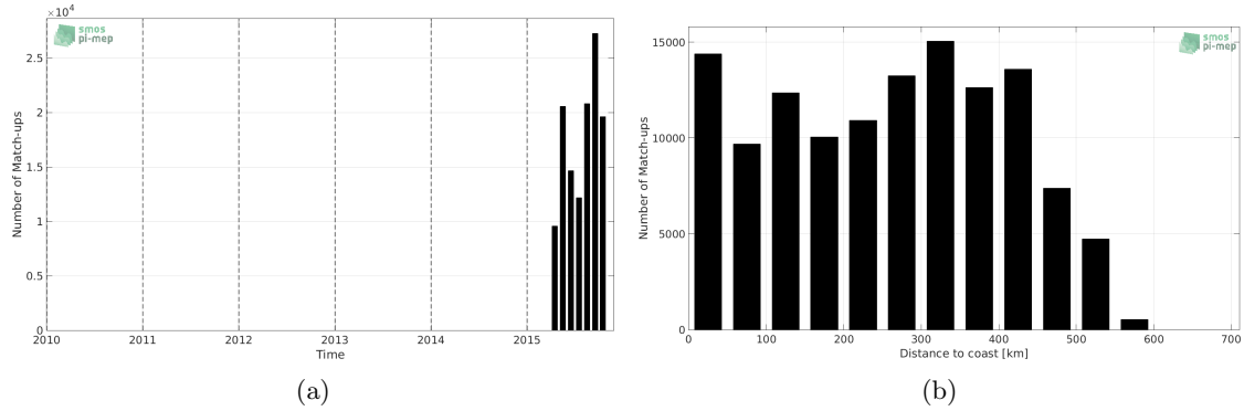
Figure 1: Number of match-ups between TSG-GOSUD-Research-vessel and SMAP-L3-JPL-V4-MONTHLY-60KM SSS as a function of time (a) and as function of the distance to coast (b) over the Pacific Ocean Pi-MEP region and for the full satellite product period.
