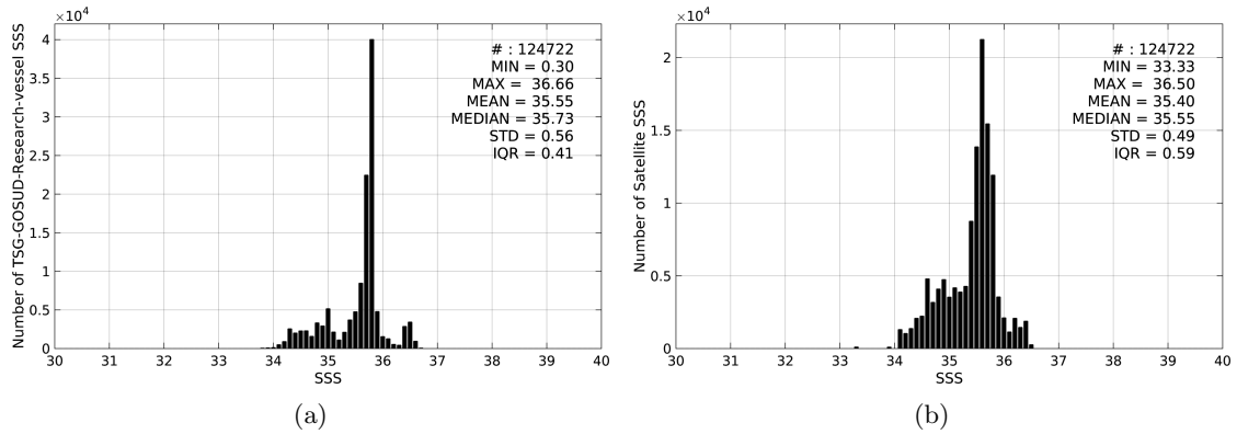
Figure 2: Histograms of SSS from TSG-GOSUD-Research-vessel (a) and SMAP-L3-JPL-V4-MONTHLY-60KM (b) considering all match-up pairs per bins of 0.1 over the Pacific Ocean Pi-MEP region and for the full satellite product period.
