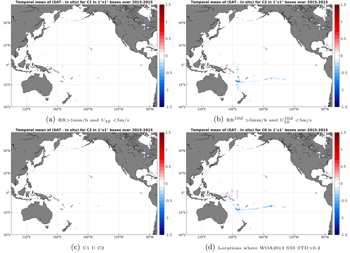
Figure 12: Temporal mean gridded over spatial boxes of size 1^\circ \times 1^\circ of \Delta SSS (SMAP-L3-JPL-V4-MONTHLY-60KM - TSG-GOSUD-Research-vessel) for 4 different subdatasets corresponding to: RR > 1\text{mm/h} and U_{10} < 5\text{m/s} (a), RR^{10d} > 5\text{mm/h} and U_{10}^{10d} < 5\text{m/s} (b), C1 U C2 (c), Locations where WOA2013 SSS STD > 0.2 (d).
