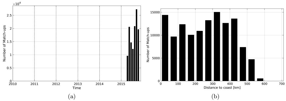
Figure 1: Number of match-ups between TSG-GOSUD-Research-vessel and SMAP-L3-JPL-V4-MONTHLY-60KM SSS as a function of time (a) and as function of the distance to coast (b) over the Pacific Ocean Pi-MEP region and for the full satellite product period.
