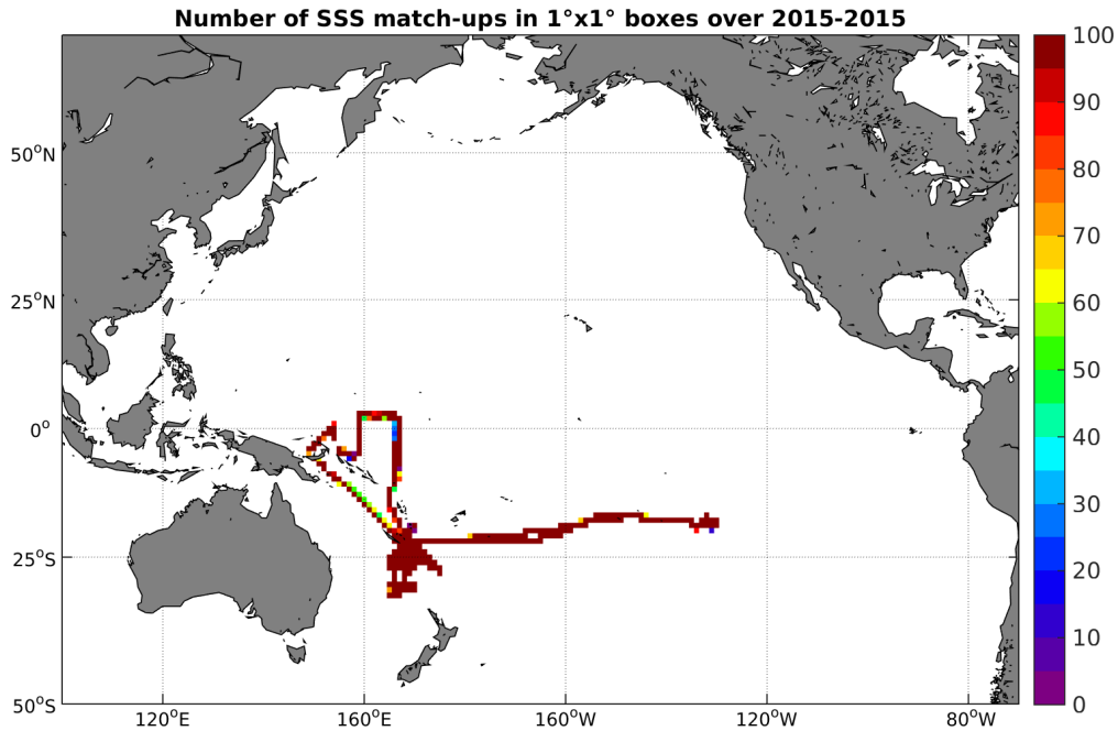
Figure 4: Number of SSS match-ups between TSG-GOSUD-Research-vessel SSS and the SMAP-L3-JPL-V4-MONTHLY-60KM SSS product for the Pacific Ocean Pi-MEP region over 1^\circ \times 1^\circ boxes and for the full satellite product period.
