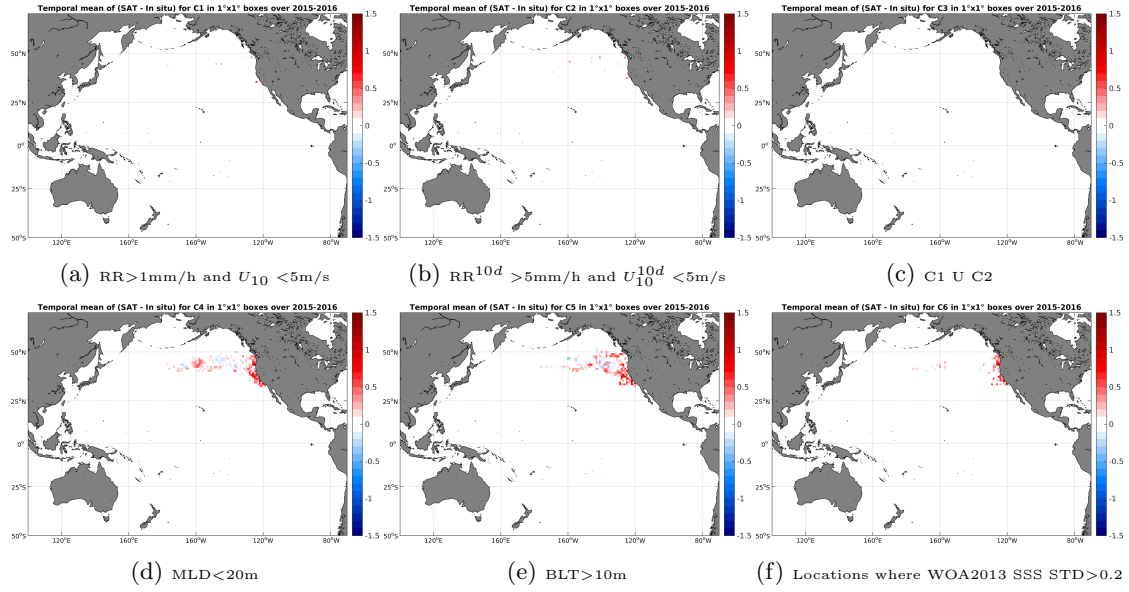
Figure 12: Temporal mean gridded over spatial boxes of size 1^\circ \times 1^\circ of \Delta SSS (SMAP-L3-JPL-V4-MONTHLY-60KM - Sea mammals) for 6 different subdatasets corresponding to: RR > 1\text{mm/h} and U_{10} < 5\text{m/s} (a), RR^{10d} > 5\text{mm/h} and U_{10}^{10d} < 5\text{m/s} (b), C1 U C2 (c), MLD < 20\text{m} (d), BLT > 10\text{m} (e), Locations where WOA2013 SSS STD > 0.2 (f).
