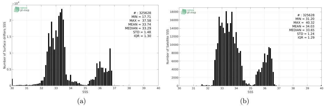
Figure 2: Histograms of SSS from Surface drifters (a) and SMAP-L3-JPL-V4-MONTHLY-60KM (b) considering all match-up pairs per bins of 0.1 over the Pacific Ocean Pi-MEP region and for the full satellite product period.
