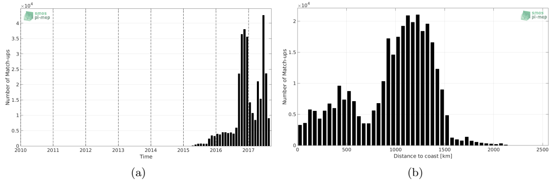
Figure 1: Number of match-ups between Surface drifters and SMAP-L3-JPL-V4-MONTHLY-60KM SSS as a function of time (a) and as function of the distance to coast (b) over the Pacific Ocean Pi-MEP region and for the full satellite product period.
