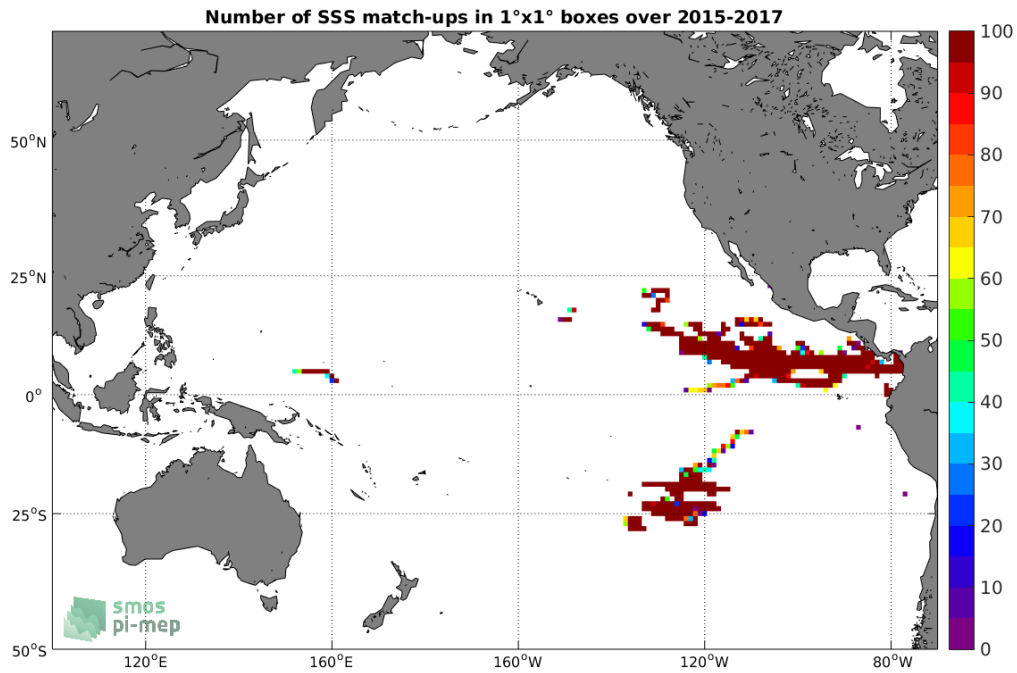
Figure 3: Number of SSS match-ups between Surface drifters SSS and the SMAP-L3-JPL-V4-MONTHLY-60KM SSS product for the Pacific Ocean Pi-MEP region over 1°x1° boxes and for the full satellite product period.
