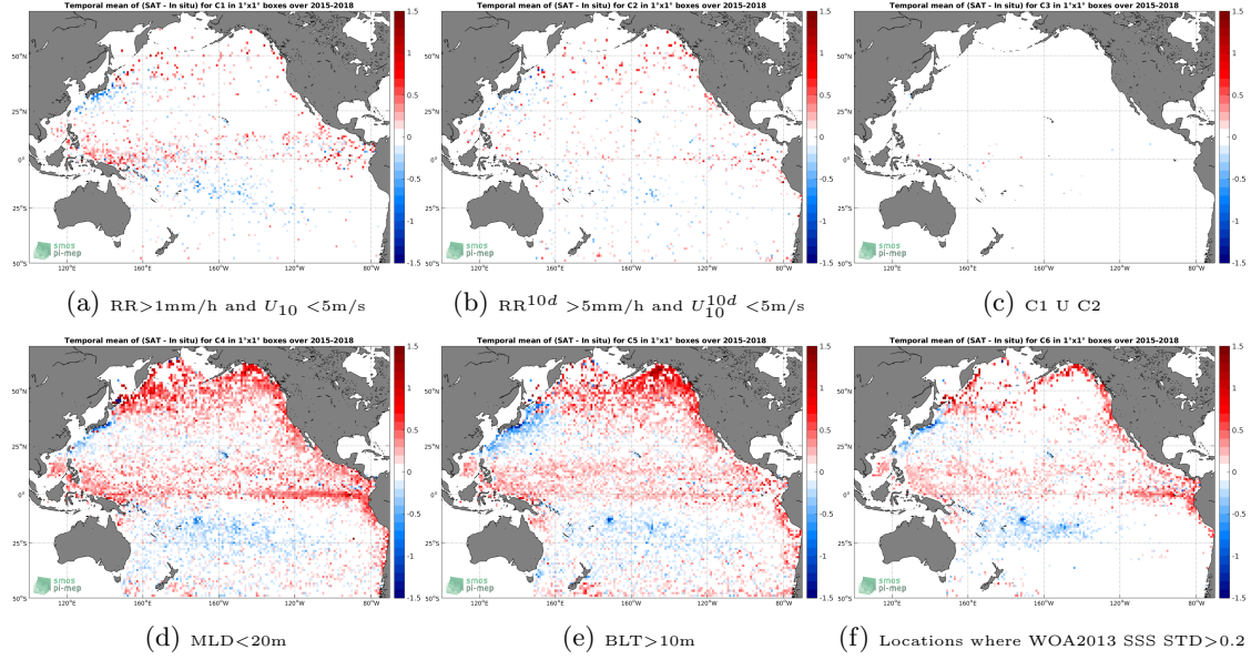
Figure 12: Temporal mean gridded over spatial boxes of size 1^\circ \times 1^\circ of \Delta\text{SSS} (SMAP-L3-JPL-V4-MONTHLY-60KM - Argo) for 6 different subdatasets corresponding to: RR > 1\text{mm/h} and U_{10} < 5\text{m/s} (a), RR^{10d} > 5\text{mm/h} and U_{10}^{10d} < 5\text{m/s} (b), C1 U C2 (c), MLD < 20\text{m} (d), BLT > 10\text{m} (e), Locations where WOA2013 SSS STD > 0.2 (f).
