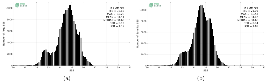
Figure 2: Histograms of SSS from Argo (a) and SMAP-L3-JPL-V4-MONTHLY-60KM (b) considering all match-up pairs per bins of 0.1 over the Pacific Ocean Pi-MEP region and for the full satellite product period.
