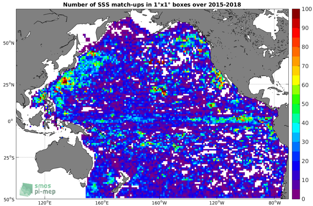
Figure 4: Number of SSS match-ups between Argo SSS and the SMAP-L3-JPL-V4-MONTHLY-60KM SSS product for the Pacific Ocean Pi-MEP region over 1°x1° boxes and for the full satellite product period.
