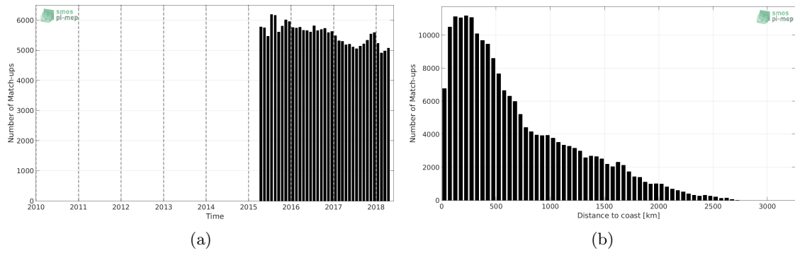
Figure 1: Number of match-ups between Argo and SMAP-L3-JPL-V4-MONTHLY-60KM SSS as a function of time (a) and as function of the distance to coast (b) over the Pacific Ocean Pi-MEP region and for the full satellite product period.
