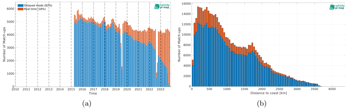
Figure 1: Number of match-ups between Argo and SMAP SSS L2-AVERAGED v5.0 (JPL) SSS as a function of time (a) and as function of the distance to coast (b) over the Pacific Ocean Pi-MEP region and for the full satellite product period.
