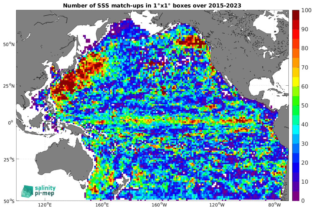
Figure 4: Number of SSS match-ups between Argo SSS and the SMAP SSS L2-AVERAGED v5.0 (JPL) SSS product for the Pacific Ocean Pi-MEP region over 1^\circ \times 1^\circ boxes and for the full satellite product period.
