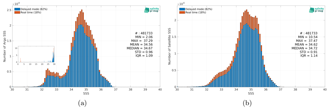
Figure 2: Histograms of SSS from Argo (a) and SMAP SSS L2-AVERAGED v5.0 (JPL) (b) considering all match-up pairs per bins of 0.1 over the Pacific Ocean Pi-MEP region and for the full satellite product period.
