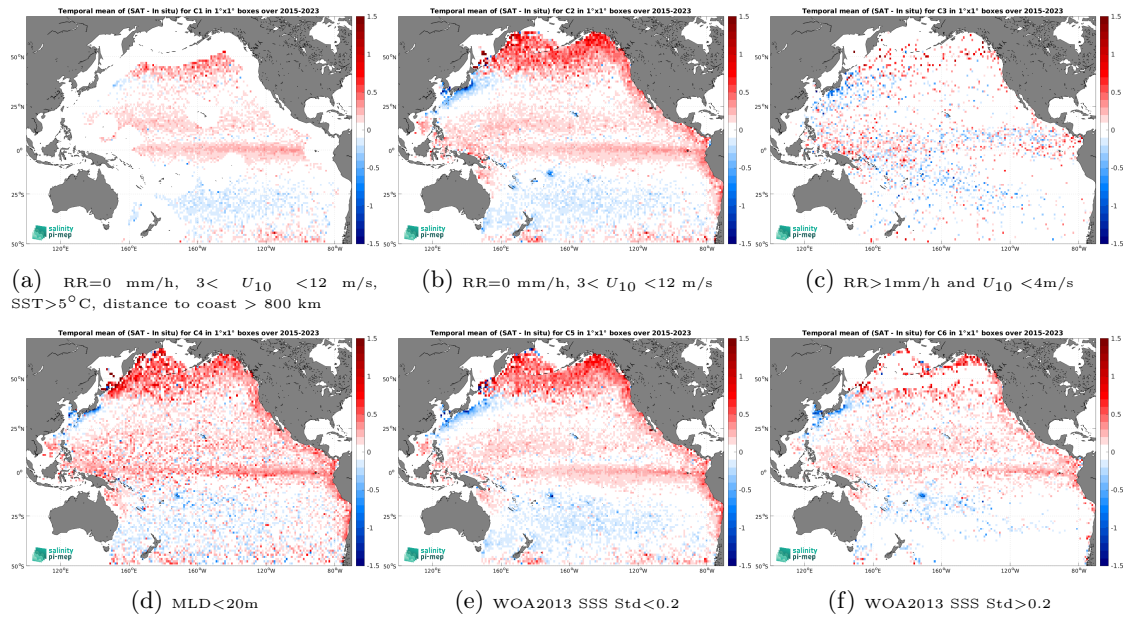
Figure 12: Temporal mean gridded over spatial boxes of size 1^\circ \times 1^\circ of \Delta SSS (SMAP SSS L2-AVERAGED v5.0 (JPL) - Argo) for 6 different subdatasets corresponding to:RR=0 mm/h, 3 < U_{10} < 12 m/s, SST > 5^\circ\text{C} , distance to coast > 800 km (a), RR=0 mm/h, 3 < U_{10} < 12 m/s (b), RR > 1 mm/h and U_{10} < 4 m/s (c),MLD < 20 m (d),WOA2013 SSS Std < 0.2 (e),WOA2013 SSS Std > 0.2 (f).
