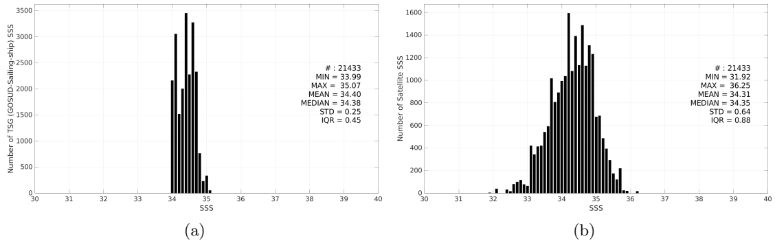
Figure 3: Histograms of SSS from TSG (GOSUD-Sailing-ship) (a) and SMAP SSS L2 v6 (RSS) (b) considering all match-up pairs per bins of 0.1 over the Pacific Ocean Pi-MEP region and for the full satellite product period.
