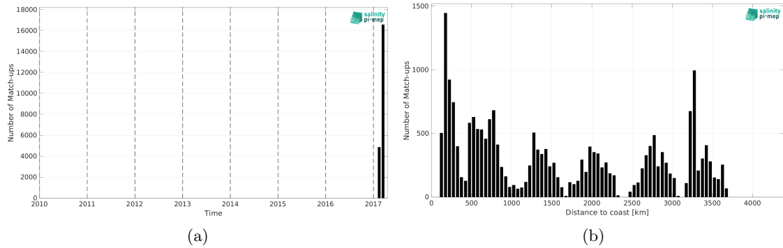
Figure 2: Number of match-ups between TSG (GOSUD-Sailing-ship) and SMAP SSS L2 v6 (RSS) SSS as a function of time (a) and as function of the distance to coast (b) over the Pacific Ocean Pi-MEP region and for the full satellite product period.
