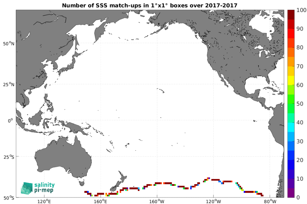
Figure 5: Number of SSS match-ups between TSG (GOSUD-Sailing-ship) SSS and the SMAP SSS L2 v6 (RSS) SSS product for the Pacific Ocean Pi-MEP region over 1^\circ \times 1^\circ boxes and for the full satellite product period.
