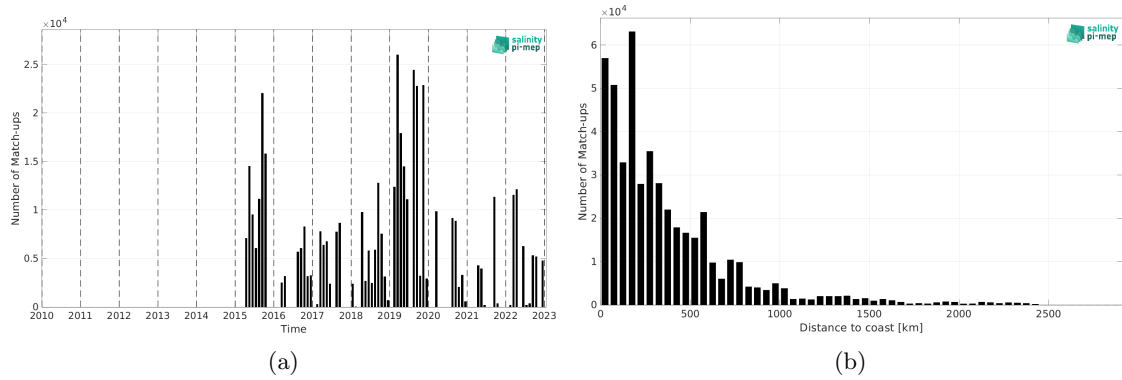
Figure 2: Number of match-ups between TSG (GOSUD-Research-vessel) and SMAP SSS L2 v6 (RSS) SSS as a function of time (a) and as function of the distance to coast (b) over the Pacific Ocean Pi-MEP region and for the full satellite product period.
