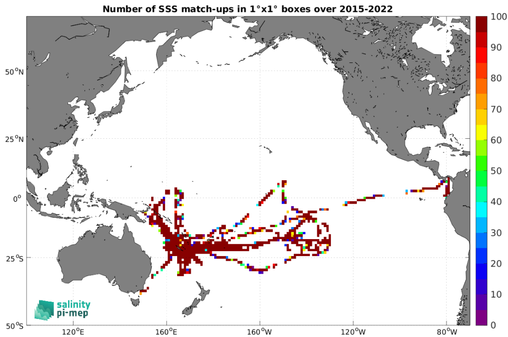
Figure 5: Number of SSS match-ups between TSG (GOSUD-Research-vessel) SSS and the SMAP SSS L2 v6 (RSS) SSS product for the Pacific Ocean Pi-MEP region over 1^\circ \times 1^\circ boxes and for the full satellite product period.
