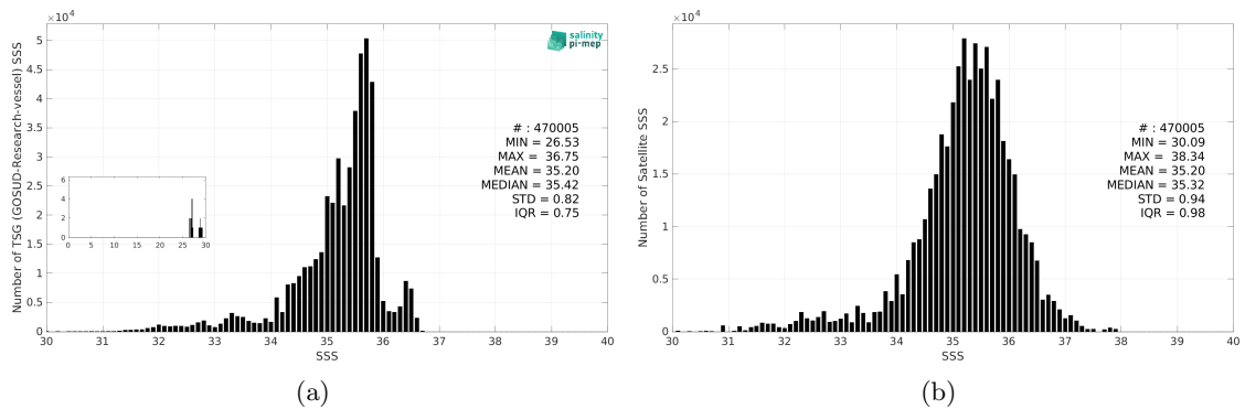
Figure 3: Histograms of SSS from TSG (GOSUD-Research-vessel) (a) and SMAP SSS L2 v6 (RSS) (b) considering all match-up pairs per bins of 0.1 over the Pacific Ocean Pi-MEP region and for the full satellite product period.
