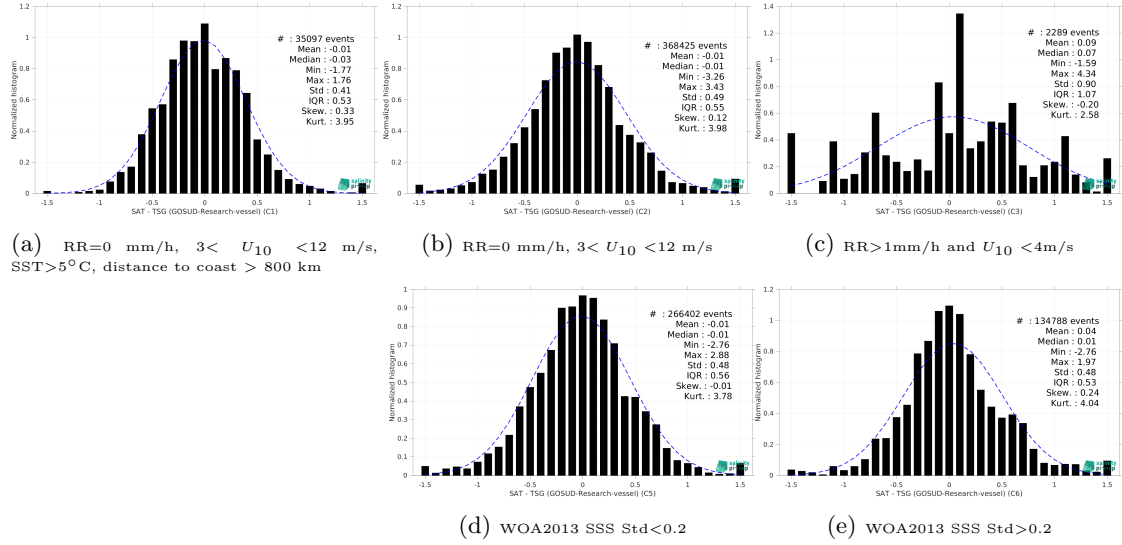
Figure 15: Normalized histogram of \Delta\text{SSS} (SMAP SSS L2 v6 (RSS) - TSG (GOSUD-Research-vessel)) for 5 different subdatasets corresponding to: RR=0 mm/h, 3 < U_{10} < 12 m/s, SST>5°C, distance to coast > 800 km (a), RR=0 mm/h, 3 < U_{10} < 12 m/s (b), RR>1mm/h and U_{10} < 4 m/s (c), WOA2013 SSS Std<0.2 (d), WOA2013 SSS Std>0.2 (e).
